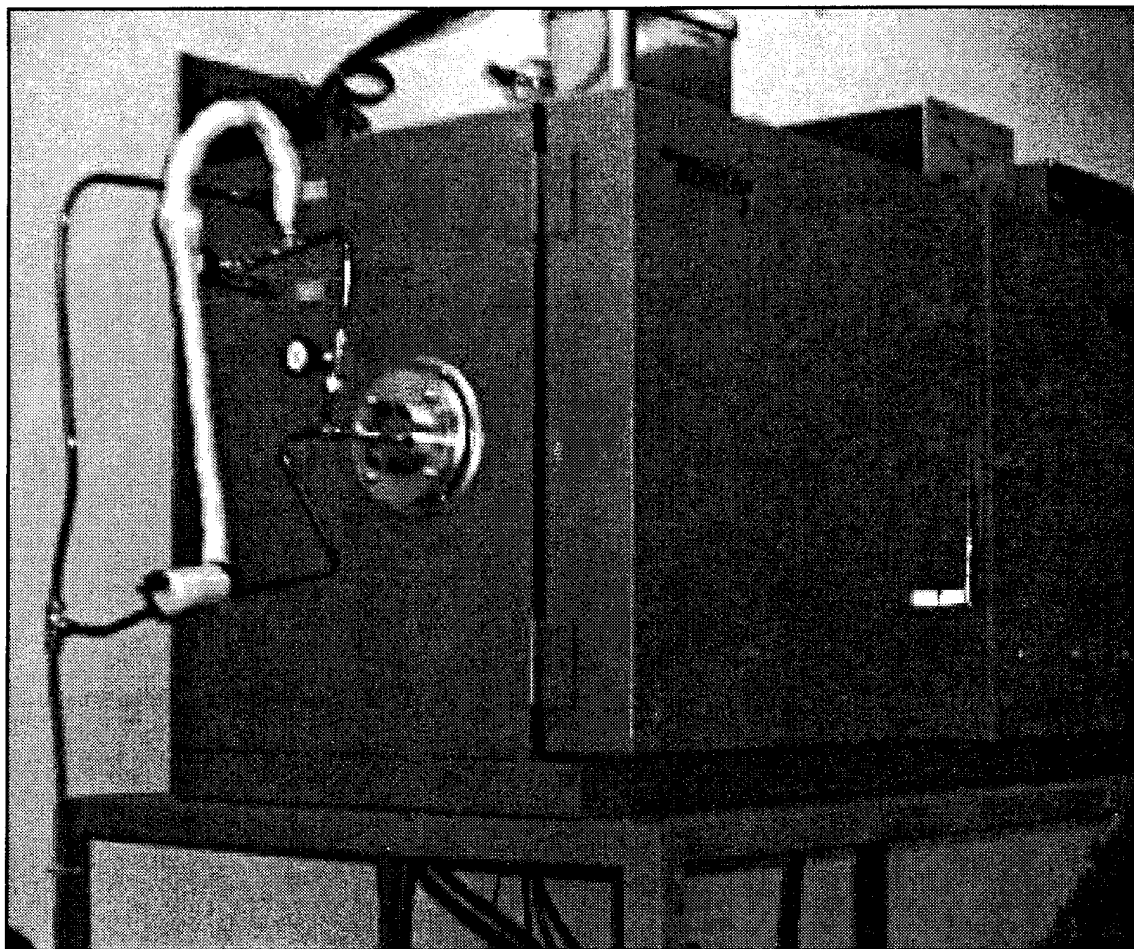
Figure 1.7 One Cubic Foot Thermal-Vacuum Chamber
