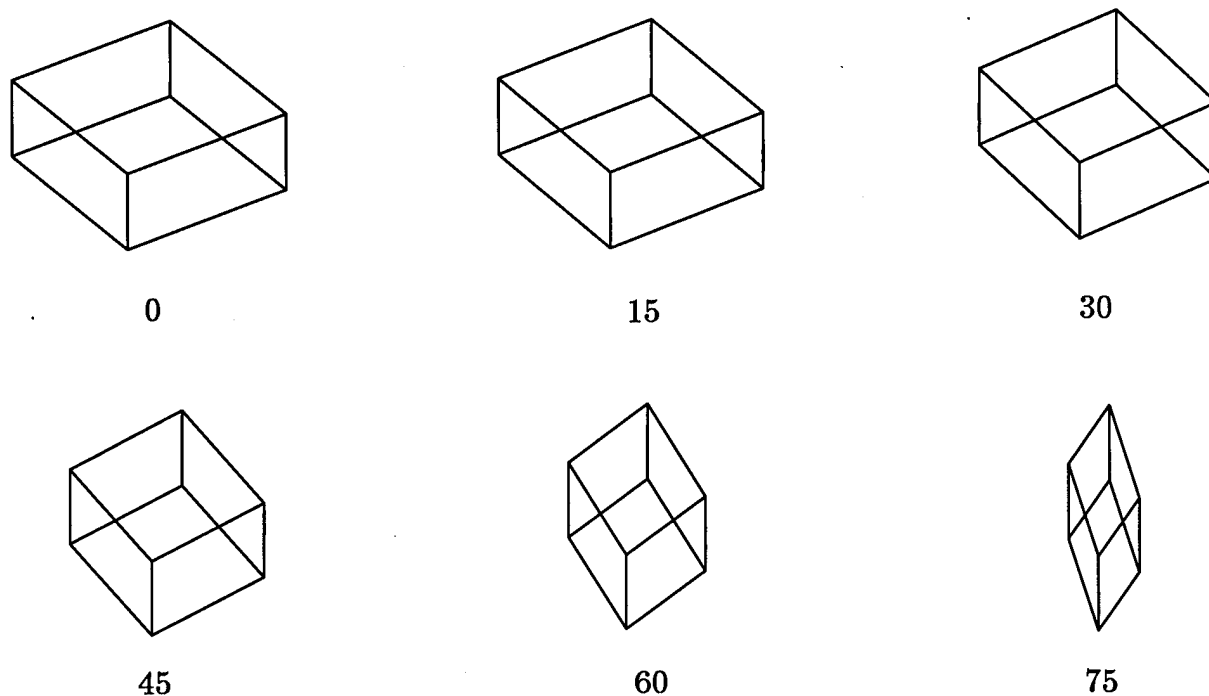
Figure 6: Rotated views of Figure 2(g). Angle in degrees.
