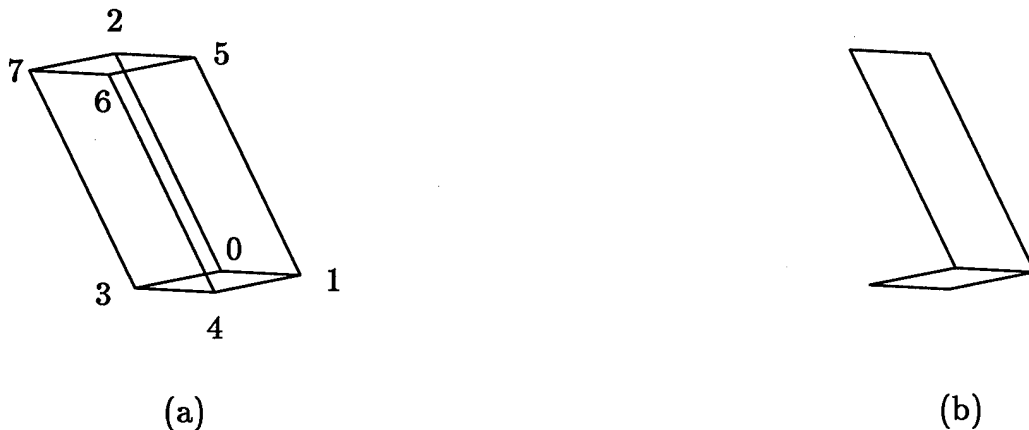
Figure 5: Interpretation of non-conforming p-image
