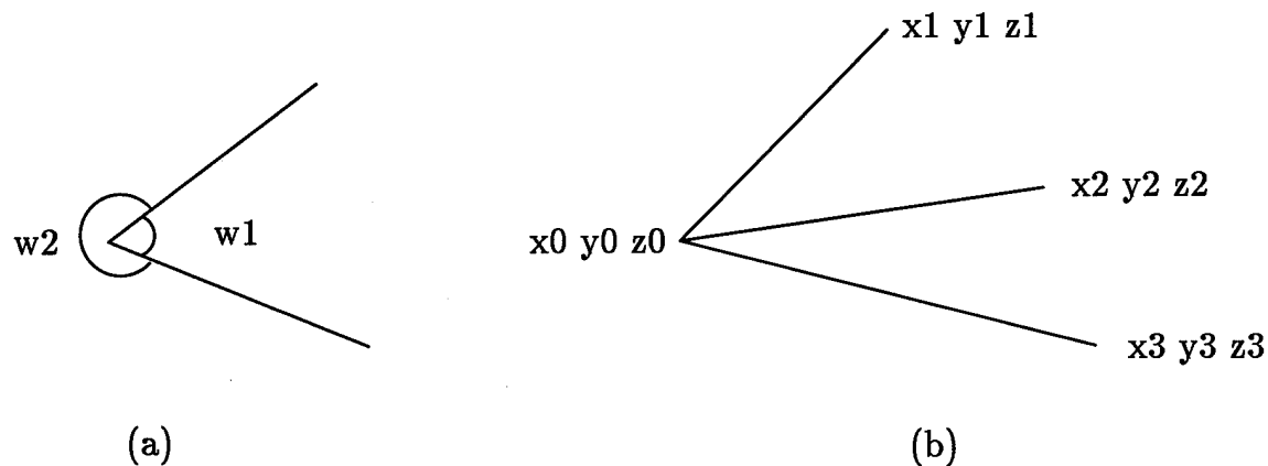
Figure 9: (a) Angle. (b) Triple vertex.
