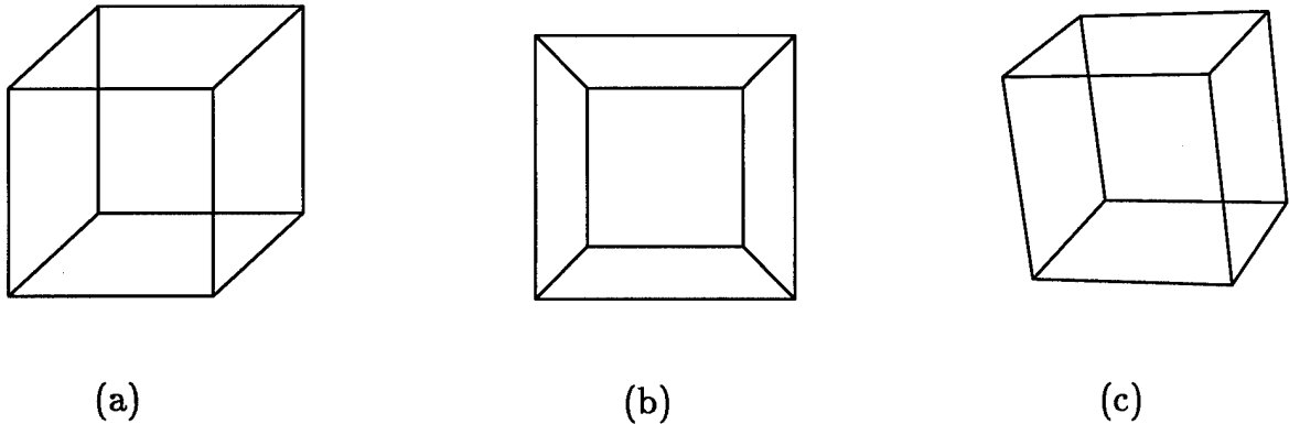
Figure 8: (a) A paradoxical p-image. There is no cube that projects to this image. (b) Perspective projection of frontal cube. (c) Perspective projection of tilted cube.
