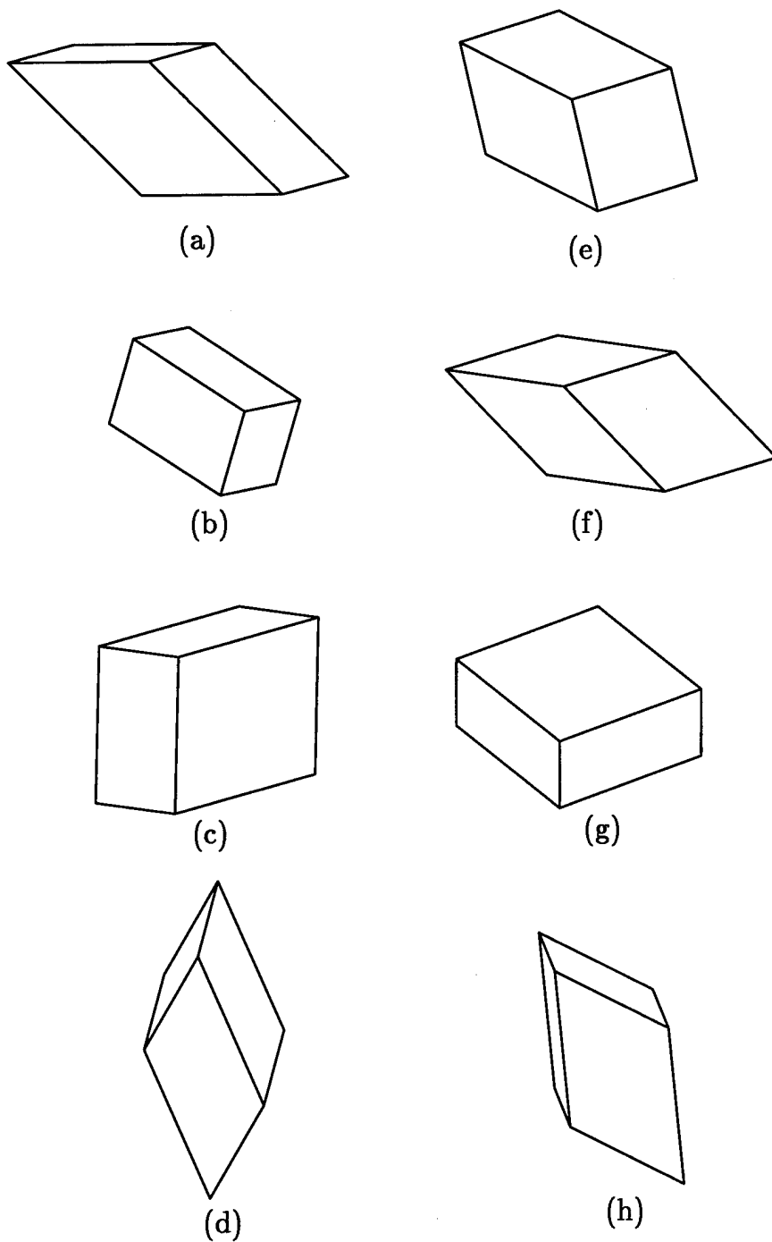
Figure 4: Reduced p-images corresponding to Figure 2.
