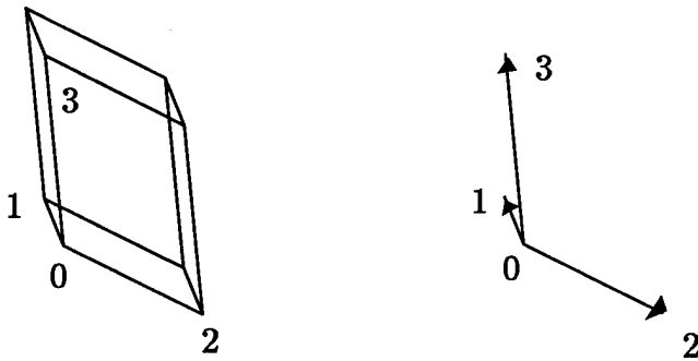
Figure 3: Basis vectors for p-image.
