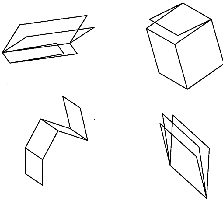
Figure 1: Random parallelogram meshes.
