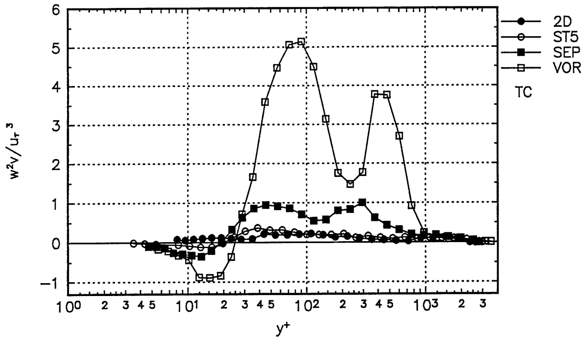
Figure 18. \overline{w^2v}/u_\tau^3 triple product at different stations in tunnel coordinates. ●, 2-D; ○, Station 5, ■, Separation station; □, Vortex station.
