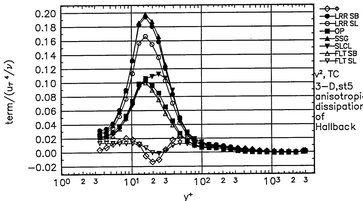
Figure 112. Comparison of \overline{v^2} normal stress transport experimental pressure-strain term \hat{\phi} , to theoretical pressure-strain terms for Station 5. Gibson-Lauder, \bullet ; Launder-Reece-Rodi (LRR), \circ ; Oberlack-Peters (OP), \blacksquare ; Speziale-Sarkar-Gatski (SSG), \blacktriangle ; Shih-Lumley/Choi-Lumley (SLCL), \blacktriangledown ; Fu-Lauder-Tselepidakis 1 (FLT1), \triangle ; Fu-Lauder-Tselepidakis 2 (FLT2), \triangledown . No near-wall corrections, anisotropic dissipation of Hallbäck.
