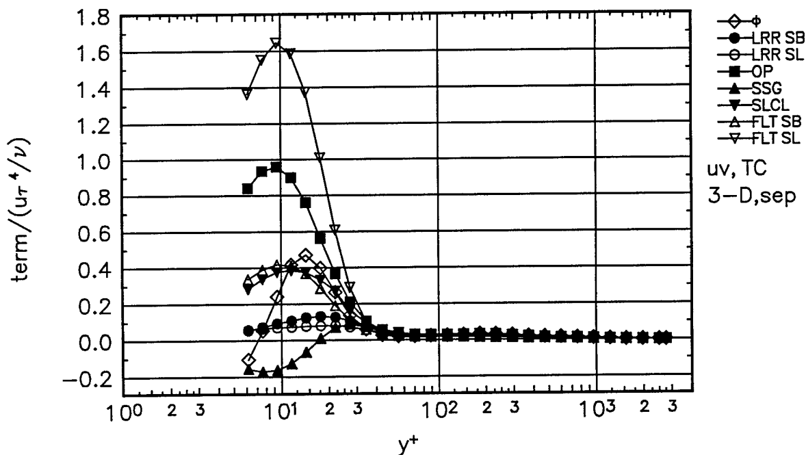
Figure 72. Comparison of \bar{uv} shear stress transport experimental pressure-strain term \hat{\phi} , to theoretical pressure-strain terms for Separation station. Gibson-Lauder, \bullet ; Launder-Reece-Rodi (LRR), \circ ; Oberlack-Peters (OP), \blacksquare ; Speziale-Sarkar-Gatski (SSG), \blacktriangle ; Shih-Lumley/Choi-Lumley (SLCL), \nabla ; Fu-Lauder-Tselepidakis 1 (FLT1), \triangle ; Fu-Lauder-Tselepidakis 2 (FLT2), \nabla . No near-wall corrections, dissipation is assumed zero.
