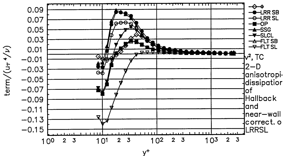
Figure 156. Comparison of \overline{v^2} normal stress transport experimental pressure-strain term \hat{\phi} , to theoretical pressure-strain terms for the 2-D station. Gibson-Lauder, \bullet ; Launder-Reece-Rodi (LRR), \circ ; Oberlack-Peters (OP), \blacksquare ; Speziale-Sarkar-Gatski (SSG), \blacktriangle ; Shih-Lumley/Choi-Lumley (SLCL), \nabla ; Fu-Lauder-Tselepidakis 1 (FLT1), \triangle ; Fu-Lauder-Tselepidakis 2 (FLT2), \nabla . Near-wall corrections of Launder-Reece-Rodi (1975), anisotropic dissipation of Hallback (1990).
