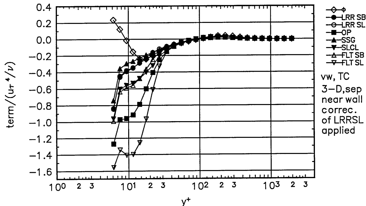
Figure 148. Comparison of \overline{vw} shear stress transport experimental pressure-strain term \phi , to theoretical pressure-strain terms for Separation station. Gibson-Lauder, \bullet ; Launder-Reece-Rodi (LRR), \circ ; Oberlack-Peters (OP), \blacksquare ; Speziale-Sarkar-Gatski (SSG), \blacktriangle ; Shih-Lumley/Choi-Lumley (SLCL), \nabla ; Fu-Lauder-Tselepidakis 1 (FLT1), \triangle ; Fu-Lauder-Tselepidakis 2 (FLT2), \nabla . Near-wall corrections of Launder-Reece-Rodi (1975), dissipation is assumed zero.
