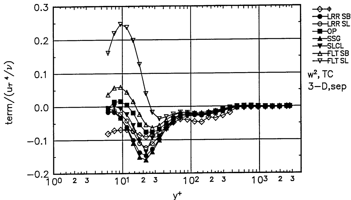
Figure 71. Comparison of \bar{w}^2 normal stress transport experimental pressure-strain term \hat{\phi} , to theoretical pressure-strain terms for Separation station. Gibson-Lauder, \bullet ; Launder-Reece-Rodi (LRR), \circ ; Oberlack-Peters (OP), \blacksquare ; Speziale-Sarkar-Gatski (SSG), \blacktriangle ; Shih-Lumley/Choi-Lumley (SLCL), \nabla ; Fu-Lauder-Tselepidakis 1 (FLT1), \triangle ; Fu-Lauder-Tselepidakis 2 (FLT2), \nabla . No near-wall corrections, dissipation is assumed isotropic.
