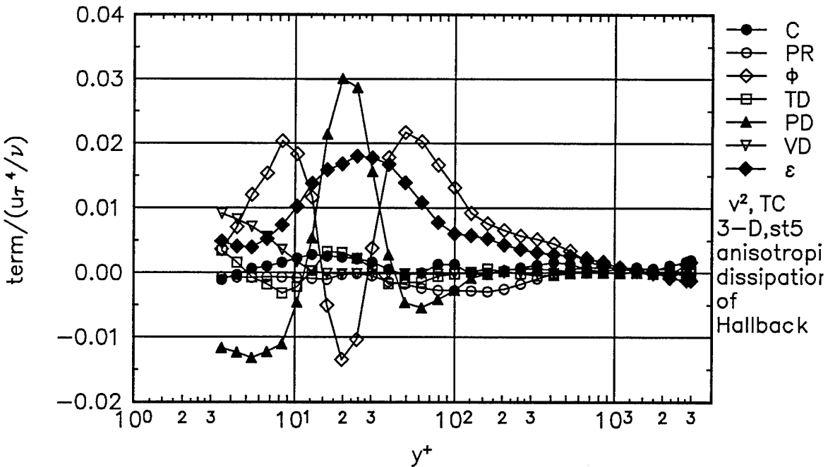
Figure 90. \overline{v^2} normal stress transport budget with anisotropic dissipation model of Hallbäck et al (1990) at Station 5 in tunnel coordinates. ●, convection (C); ○, production (PR); ◇, pressure-strain ( \phi ); □, turbulent diffusion (TD); ▲, pressure diffusion (PD); ▽, viscous diffusion (VD); ◆, dissipation ( \epsilon ).
