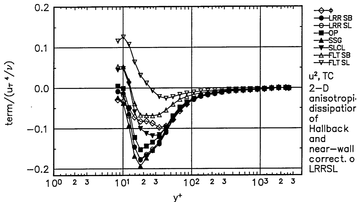
Figure 155. Comparison of \overline{u^2} normal stress transport experimental pressure-strain term \hat{\phi} , to theoretical pressure-strain terms for the 2-D station. Gibson-Lauder, \bullet ; Launder-Reece-Rodi (LRR), \circ ; Oberlack-Peters (OP), \blacksquare ; Speziale-Sarkar-Gatski (SSG), \blacktriangle ; Shih-Lumley/Choi-Lumley (SLCL), \nabla ; Fu-Lauder-Tselepidakis 1 (FLT1), \triangle ; Fu-Lauder-Tselepidakis 2 (FLT2), \nabla . Near-wall corrections of Launder-Reece-Rodi (1975), anisotropic dissipation of Hallback (1990).
