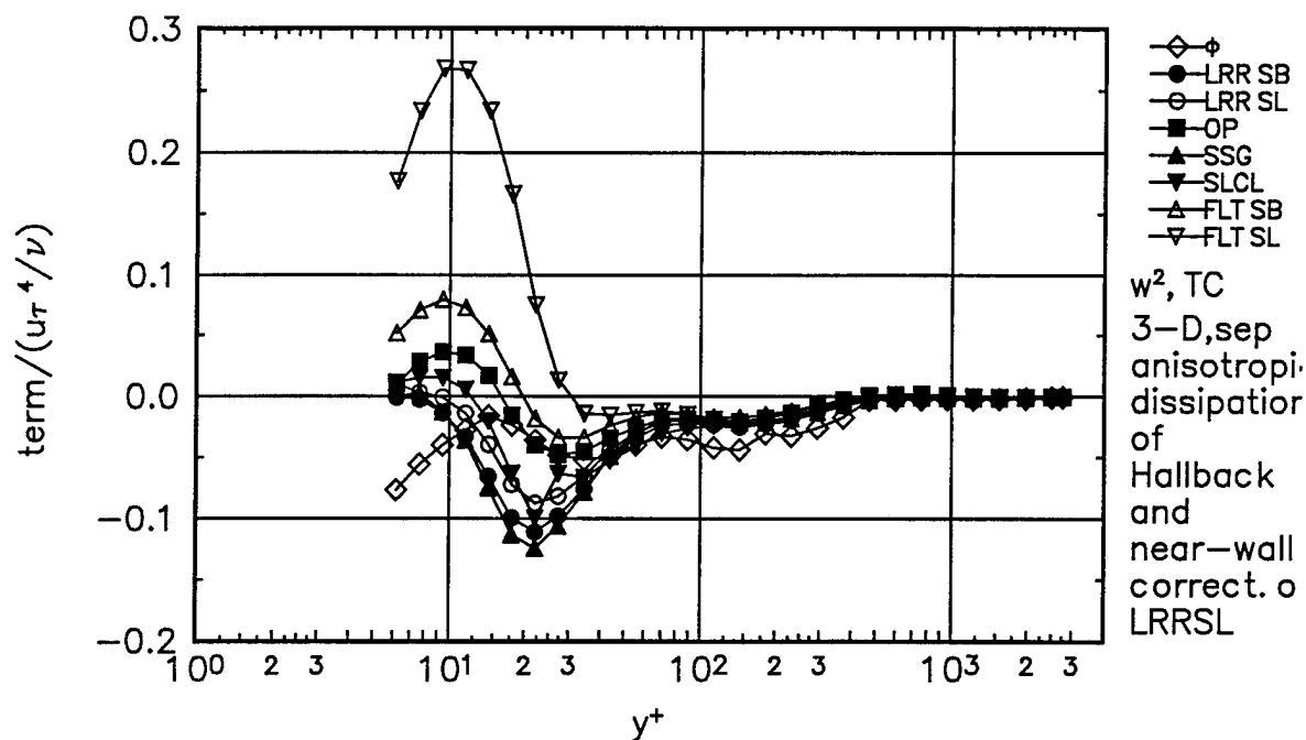
Figure 167. Comparison of \overline{w^2} normal stress transport experimental pressure-strain term \hat{\phi} , to theoretical pressure-strain terms for Separation station. Gibson-Lauder, \bullet ; Launder-Reece-Rodi (LRR), \circ ; Oberlack-Peters (OP), \blacksquare ; Speziale-Sarkar-Gatski (SSG), \blacktriangle ; Shih-Lumley/Choi-Lumley (SLCL), \nabla ; Fu-Lauder-Tselepidakis 1 (FLT1), \triangle ; Fu-Lauder-Tselepidakis 2 (FLT2), \nabla . Near-wall corrections of Launder-Reece-Rodi (1975), anisotropic dissipation of Hallbäck (1990).
