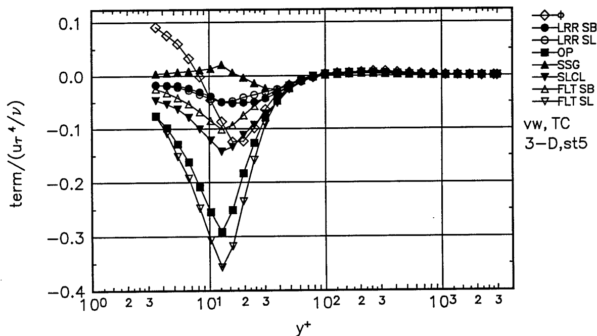
Figure 68. Comparison of \overline{vw} shear stress transport experimental pressure-strain term \phi , to theoretical pressure-strain terms for Station 5. Gibson-Lauder, \bullet ; Launder-Reece-Rodi (LRR), \circ ; Oberlack-Peters (OP), \blacksquare ; Speziale-Sarkar-Gatski (SSG), \blacktriangle ; Shih-Lumley/Choi-Lumley (SLCL), \nabla ; Fu-Lauder-Tselepidakis 1 (FLT1), \triangle ; Fu-Lauder-Tselepidakis 2 (FLT2), \nabla . No near-wall corrections, dissipation is assumed zero.
