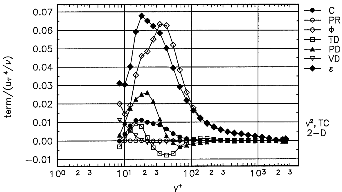
Figure 30. \overline{v^2} normal stress transport budget with isotropic dissipation assumption at 2-D station in tunnel coordinates. ●, convection (C); ○, production (PR); ◇, pressure-strain ( \phi ); □, turbulent diffusion (TD); ▲, pressure diffusion (PD); ▽, viscous diffusion (VD); ◆, dissipation ( \epsilon ).
