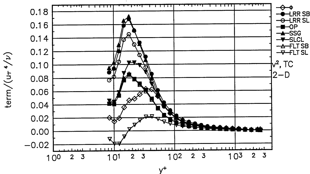
Figure 58. Comparison of \overline{v^2} normal stress transport experimental pressure-strain term \phi , to theoretical pressure-strain terms for the 2-D station. Gibson-Lauder, \bullet ; Launder-Reece-Rodi (LRR), \circ ; Oberlack-Peters (OP), \blacksquare ; Speziale-Sarkar-Gatski (SSG), \blacktriangle ; Shih-Lumley/Choi-Lumley (SLCL), \nabla ; Fu-Lauder-Tselepidakis 1 (FLT1), \triangle ; Fu-Lauder-Tselepidakis 2 (FLT2), \nabla . No near-wall corrections, dissipation is assumed isotropic.
