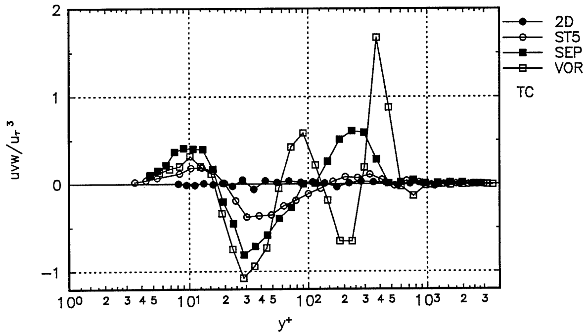
Figure 19. \overline{uvw}/u_\tau^3 triple product at different stations in tunnel coordinates. ●, 2-D; ○, Station 5, ■, Separation station; □, Vortex station.
