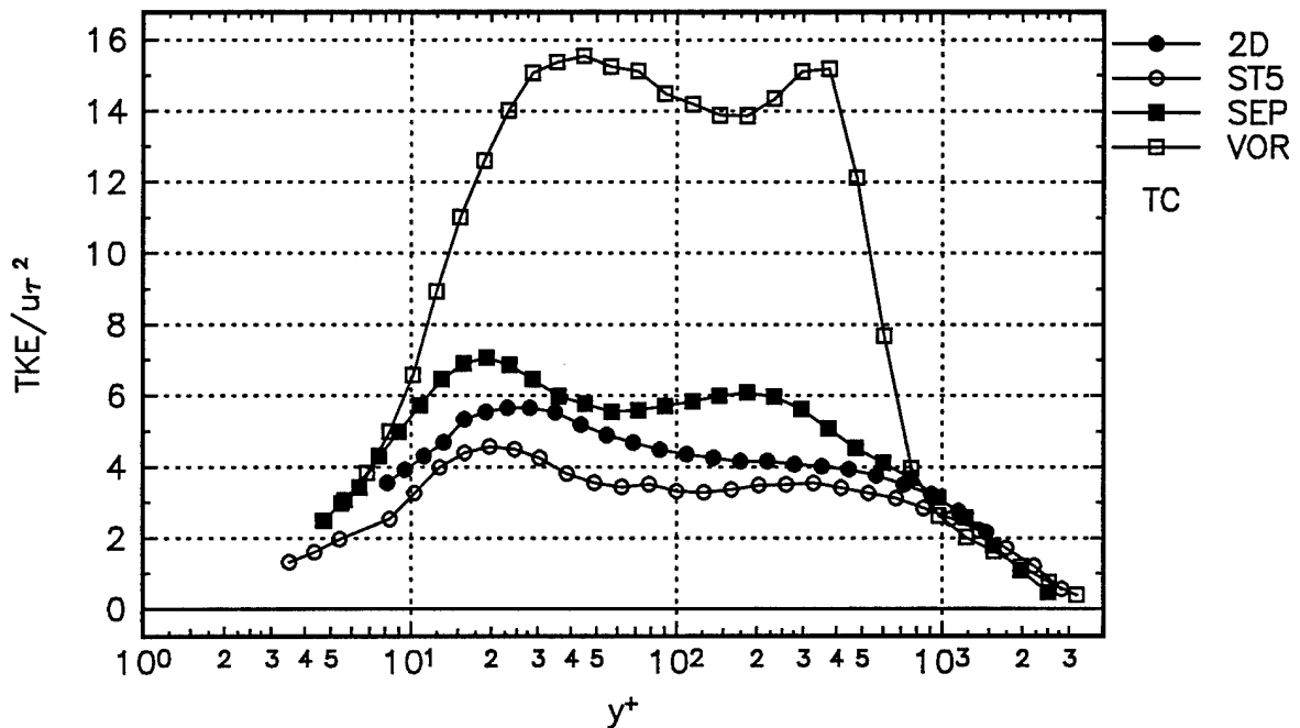
Figure 27. Turbulent kinetic energy profiles calculated at different stations. ●, 2-D; ○, Station 5, ■, Separation station; □, Vortex station.
