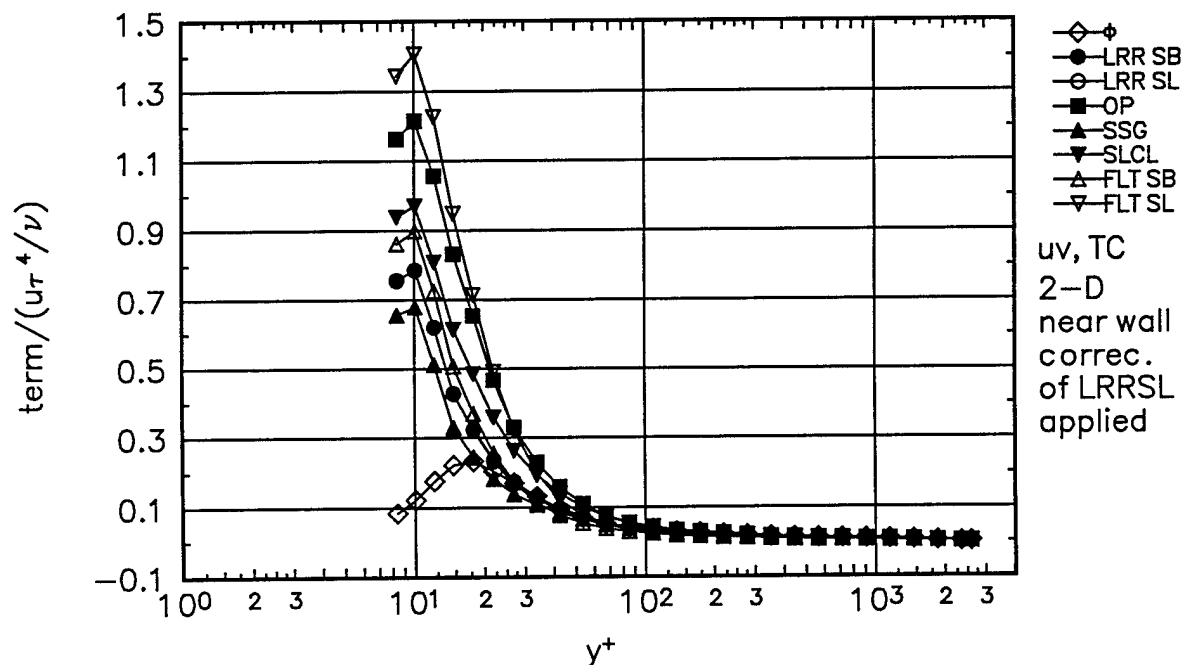
Figure 136. Comparison of \overline{uv} shear stress transport experimental pressure-strain term \phi , to theoretical pressure-strain terms for the 2-D station. Gibson-Lauder, \bullet ; Launder-Reece-Rodi (LRR), \circ ; Oberlack-Peters (OP), \blacksquare ; Speziale-Sarkar-Gatski (SSG), \blacktriangle ; Shih-Lumley/Choi-Lumley (SLCL), \nabla ; Fu-Lauder-Tselepidakis 1 (FLT1), \triangle ; Fu-Lauder-Tselepidakis 2 (FLT2), \nabla . Near-wall corrections of Launder-Reece-Rodi (1975), dissipation is assumed zero.
