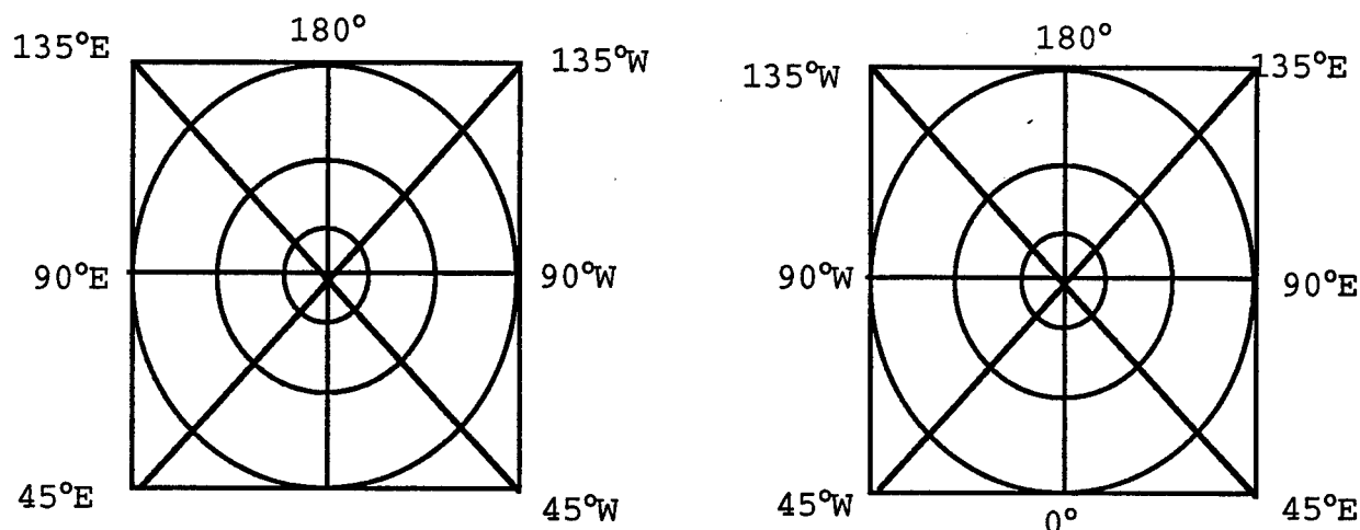
Figure 7.5. Meridians and parallels in the Universal Polar Stereographic Projection. Left: South Zone, Right: North Zone (Not drawn to scale.)
