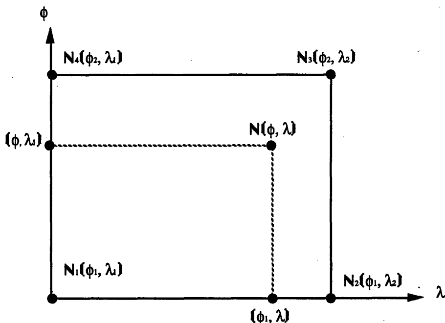
Figure F-1 Coordinate System Associated with Geoid Separation Bi-Linear Interpolation Method
