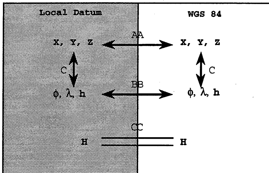
Figure 8.3. Datum shifts.
