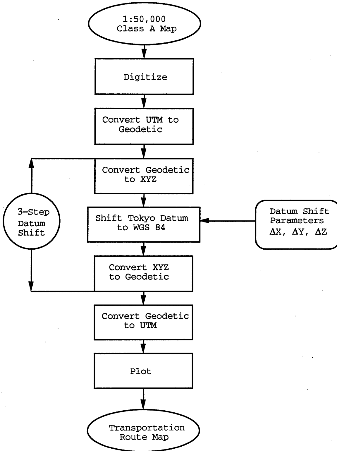
Figure 8.5. System Model
