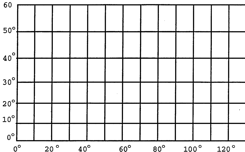
FIGURE 7.1. Meridians (longitude) and parallels (latitude) in the Mercator projection.
