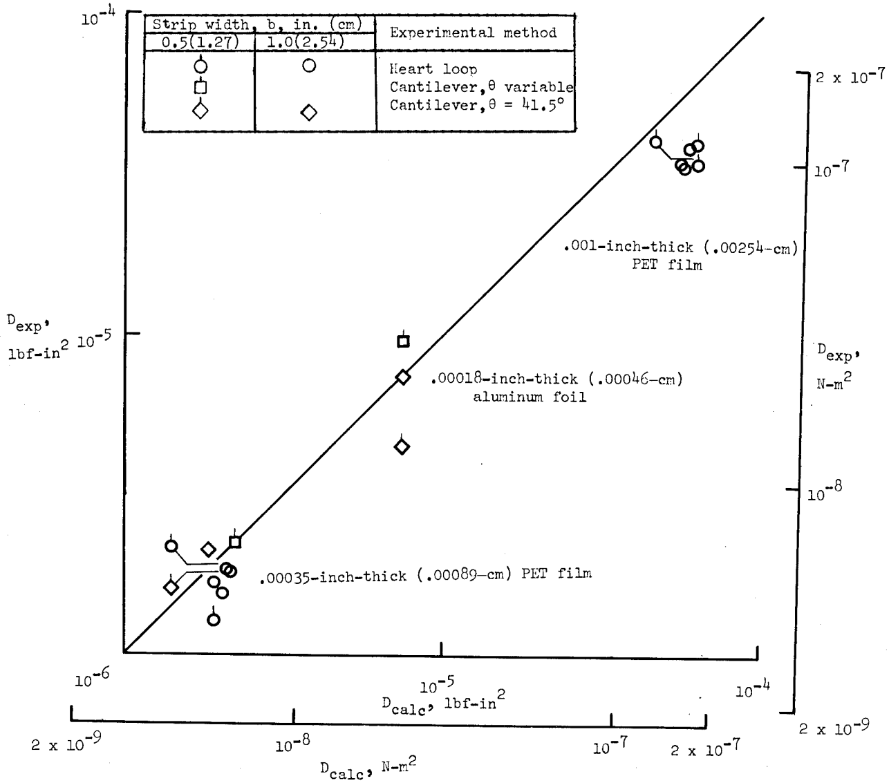
Figure 6.- Comparison of calculated and measured rigidity of PET film and aluminum foil. All 0.5-in. (1.27-cm) values were normalized to unit width when plotted.
