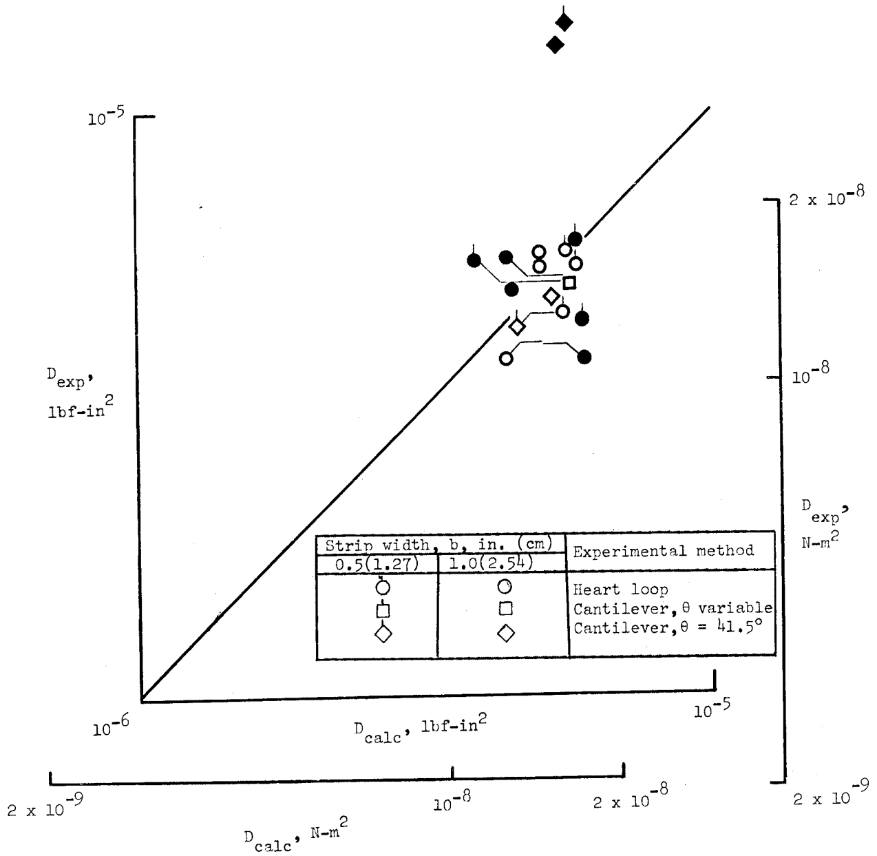
Figure 7.- Comparison of calculated and measured rigidity of Echo I material. All 0.5-in. (1.27-cm) values were normalized to unit width when plotted. Closed symbols denote aluminum in compression.
