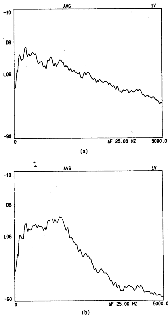
Fig. 8. FFT display of long-term spectrum (0-5-kHz range). (a) Particular male speaker. (b) Particular male speaker on a typical forensic recording.
