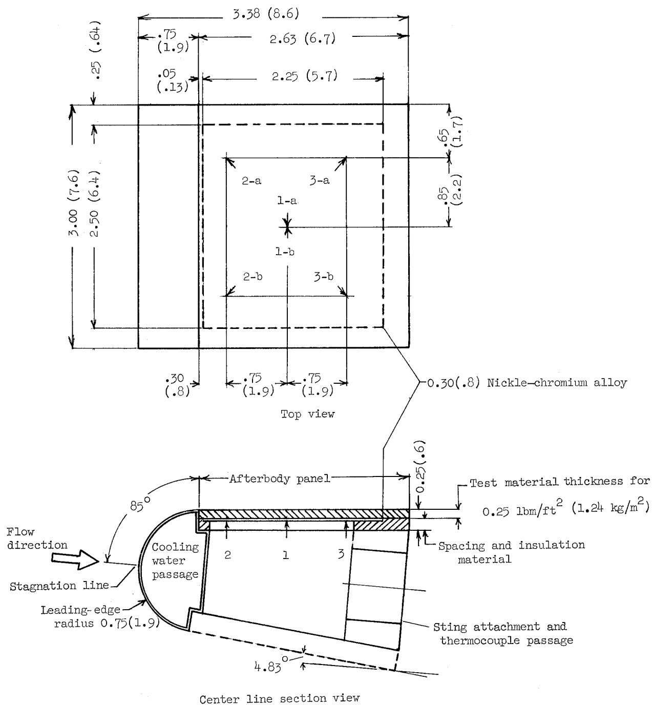
Figure 2.- Afterbody model configuration and thermocouple positions. All dimensions are in inches (centimeters).
