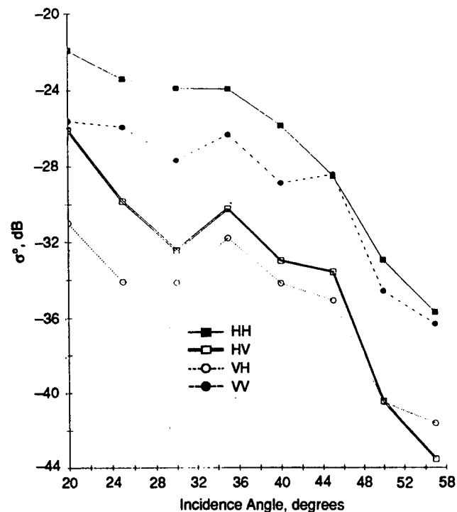
Fig. 9-32. Normalized radar cross section of rough ice at 35 GHz [Colom, 1991].
