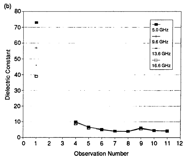
Fig. 9-11. The magnitude of the complex dielectric constant |\epsilon^*| (a) as derived from the measurement of reflectivity and (b) by prediction.
