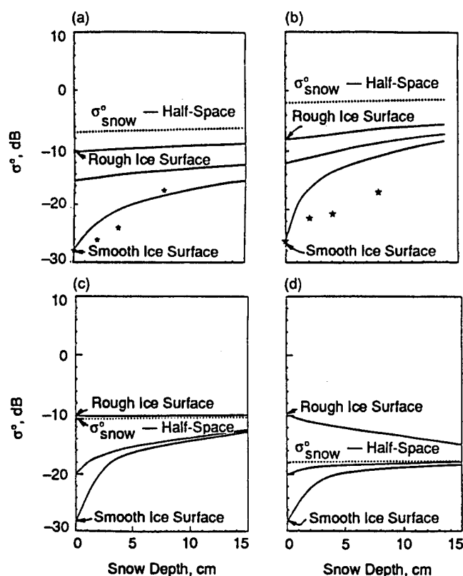
Fig. 5-14. The effect of a dry snow cover on sea ice is shown as a function of snow depth at (a) 8.6 GHz, and (b) 17.6 GHz for an angle of 50°. The solid lines are predicted \sigma^0 for snow cover and can be very low (smooth ice) or close to that of a half space of dry snow (rough ice). The effect of wet snow on sea ice is shown for a liquid water content of (c) 1% and (d) 3% for 8.6 GHz for an angle of 50° [Kim, 1984; Kim et al., 1984a].
