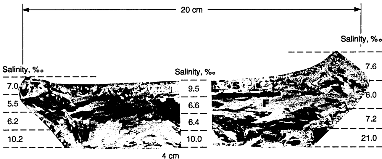
Fig. 9-6. Vertical thin-section structure and salinity profiles from a 4 cm thick pancake from CRRELEX'90. The sequence of ice textures from top to bottom of the pan is slush ice (s) underlain by platey frazil ice (f).
