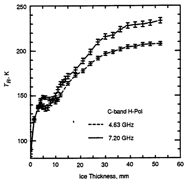
Fig. 9-13. Brightness temperature versus thickness during initial growth at two C-band frequencies and horizontal polarization. These observations cover the same ice sheet as in Figure 9-12 [Grenfell et al., 1988].
