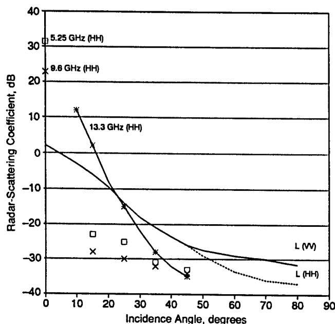
Fig. 5-8. Radar-scattering coefficient data at L-band for a medium sea [Wetzel, 1990], at 13.3 GHz (HH) for a calm ocean [Gray et al., 1982], and 5.3 GHz (HH) and 9.6 GHz (HH) for water between ice floes in the MIZ [Onstott et al., 1987].
