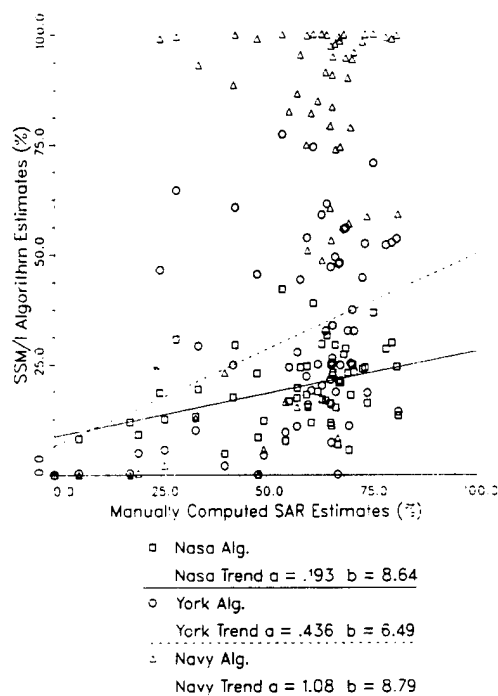
Figure 5. Multiyear Ice Concentration Estimates vs SAR for 17 March 1989 Greenland Sea Data.
