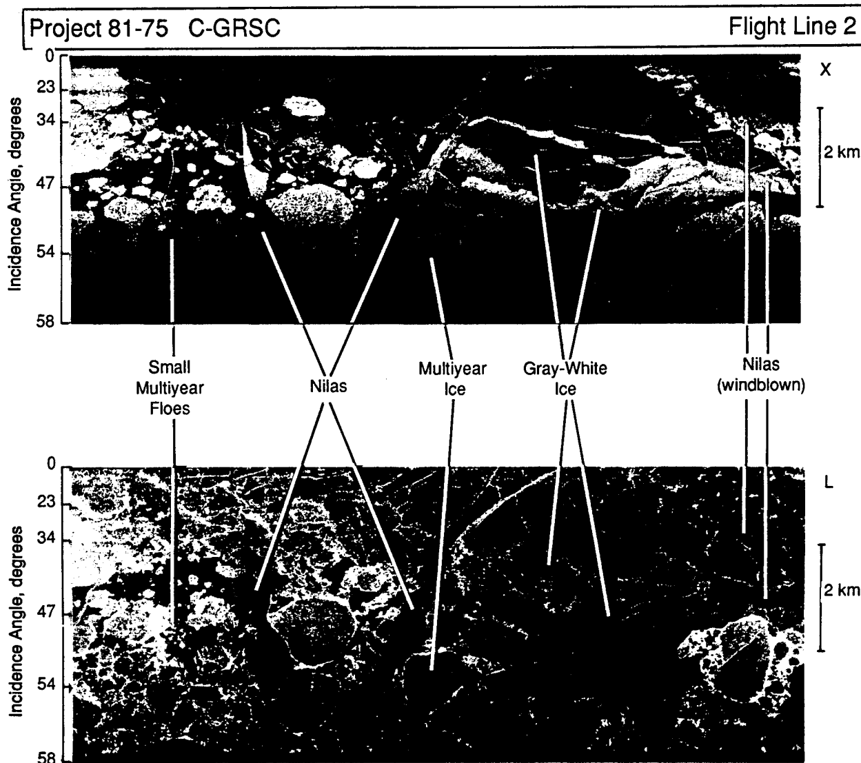
Fig. 5-28. Ice floe imagery obtained on November 1, 1981, during the Beaufort Sea Project at X-band (9.4 GHz) and L-band (1.2 GHz). Features include nilas, gray-white ice, and multiyear ice. The incidence angle range goes from 0^{\circ} to 58^{\circ} .
