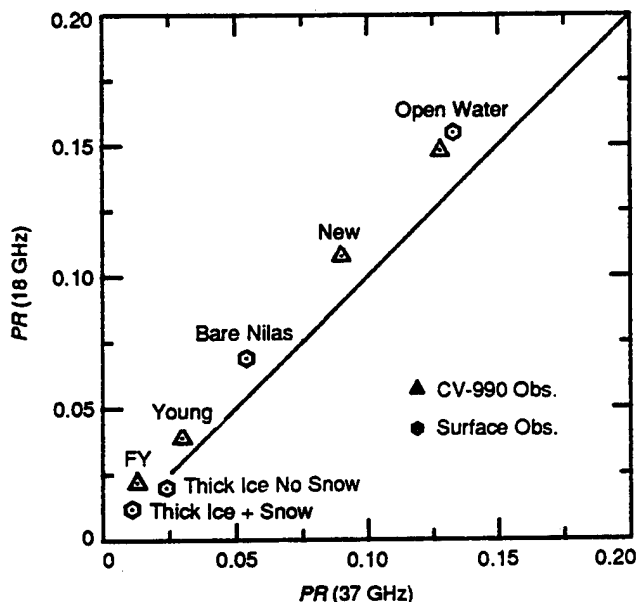
Fig. 14-8. Polarization ratio for combined aircraft-based and surface observations in the Bering Sea [Cavaliere et al., 1986]. The nadir angle is 45^\circ .
