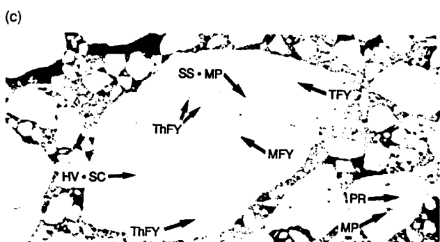
Fig. 5-29. Ice floe imagery obtained on June 29, 1984, during MIZEX'84 at (a) X-band (9.4 GHz), (b) L-band (1.2 GHz), and (c) with an aerial camera. Surface features include snow-covered ice (SC); heavily snow-covered ice (HV•SC); thick (TFY), medium (MFY), and thin first-year (ThFY) ice; pressure ridges (PR); sub-surface melt ponds (SS•MP); and melt pools (MP).
