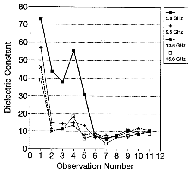
Figure 4. The Magnitude of the Complex Dielectric Constant ( \epsilon_r' ) as Derived from the Reflectivity Measurements.
