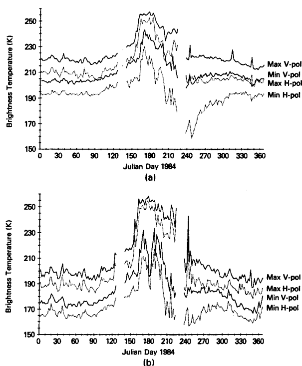
Fig. 3. Maximum and minimum (a) 18 GHz H and V and (b) 37 GHz H and V SMMR brightness temperatures for a 600 \times 600 \text{ km}^2 region north of the Canadian archipelago for 1984.
