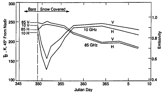
Fig. 9-35. Brightness temperatures and emissivities at 10 and 85 GHz and 45° incidence angle before and after the development of a snow cover on top of a saline ice sheet [Lohanick, 1992].
