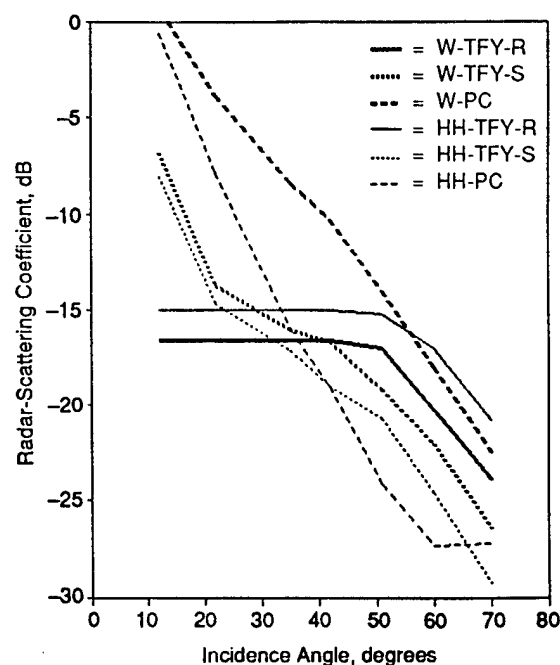
Fig. 5-15. The radar backscatter response is shown as a function of angle for smooth first-year ice of pancake origin (pans of 2- to 3-m diameters, 4-cm-high rims, and a thickness of 1.65 m), and of pancake ice (1- to 2-m pans and a thickness of 10 to 15 cm). These observations were made at 9.6 GHz. (W = water, R = rough, S = smooth, and PC = pancake ice.)
