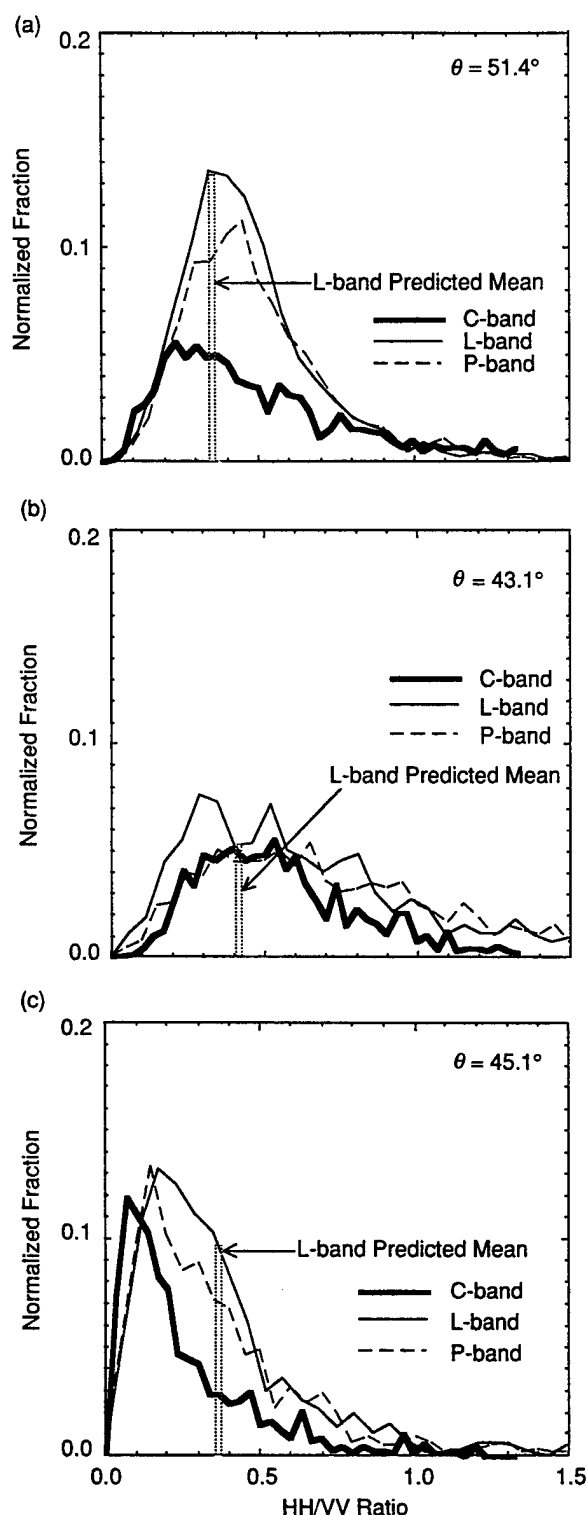
Fig. 24-3. Normalized distributions in the Beaufort Sea of individual hh/vv ratios at each frequency for (a) MY ice in box 1, (b) thick FY ice in box 2, and (c) thin FY ice in box 5. The measured L-band mean ratios are 0.44, 0.6, and 0.37 for Figure 24-1 boxes 1, 2 and 5, respectively; first-order model predictions are shown for comparison.
