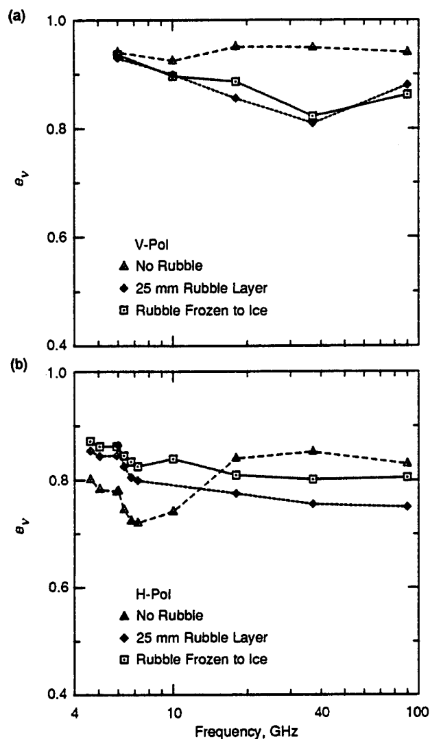
Fig. 9-30. Emissivity spectra of 150-mm-thick ice before and after the addition of a 25-mm layer of ice rubble at (a) vertical and (b) horizontal polarizations [Grenfell et al., 1988].
