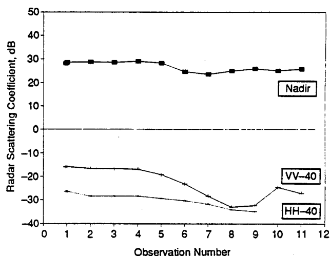
Fig. 9-8. The time series response of the backscatter coefficient at 5.0 GHz during the evolution of open water to new ice at nadir and 40° (VV and HH).
