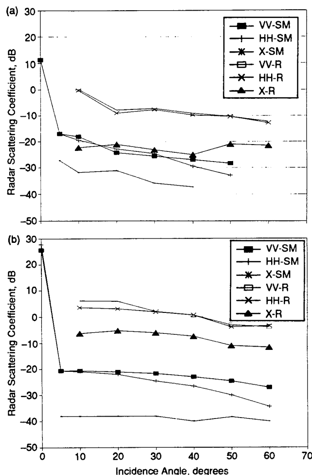
Fig. 9-29. Radar scattering coefficient response for ice with a rough (R) or smooth (SM) surface. The response is shown at (a) 5.0 and (b) 10.0 GHz.
