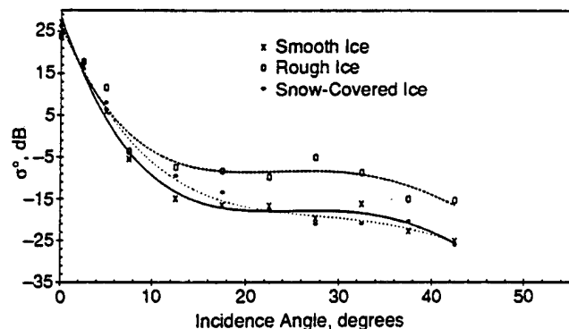
Fig. 9-26. Effects of surface conditions on backscatter angle response at 9.6 GHz and HH polarization.
