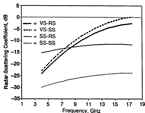
Fig. 5-6. Relative contributions of surface and volume scattering for MY ice [Kim, 1984]. The surface roughness parameters are the correlation length \ell of 8.6 cm for both smooth and rough surfaces, and height standard deviation \sigma of 0.81 cm for the rough surface and 0.15 cm for the smooth surface. The ice density is 700 kg/m 3 , the air bubble radius is 1 mm, and the complex dielectric constant is 3.15 - j0.01 . (VS = volume scatter, RS = rough surface, and SS = smooth surface.)
