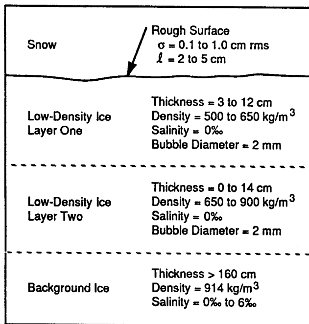
Fig. 5-5. The upper portion of multiyear ice, with a physical-property description of the various layers.
