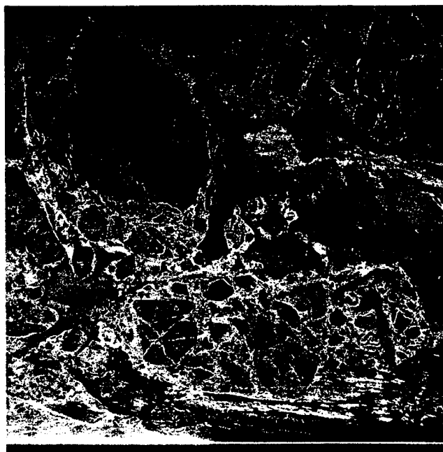
Fig. 5-26. Ice floe imagery obtained on March 21, 1989, during CEAREX with the ERIM/NADC P-3 SAR. Features include open water, nilas, gray ice, and multiyear ice. The polarization is VV and the incidence angle range goes from 20^\circ to 70^\circ . (a) An L-band (1.2-GHz) image, (b) a C-band (5.3-GHz) image, and (c) an X-band (9.4-GHz) image.
