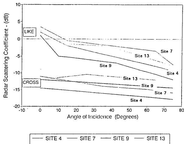
Figure 3. The angular response of the scattering coefficients for four multiyear ice hummocks at 10 GHz and like- and cross- polarizations. The responses at VV and HH polarizations were nearly identical, as were the VH and HV responses.
