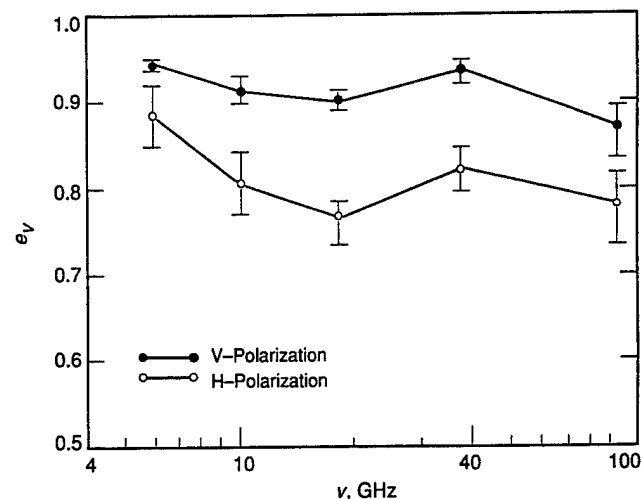
Fig. 9-24. Microwave emissivity versus frequency for the desalinated blocks in January 1989. The error bars denote the standard deviation for four independent samples.
