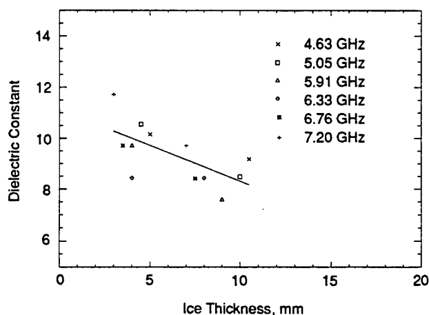
Fig. 9-15. Calculated dielectric constant as a function of the ice thickness.
