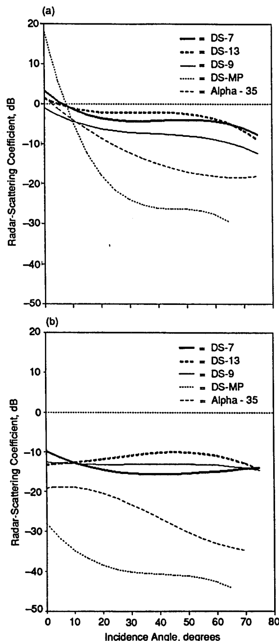
Fig. 5-17. The angular response of the scattering coefficients for four multiyear ice hummocks and a melt pool at 10 GHz and at (a) like- and (b) cross-polarizations. The responses at VV- and HH-polarizations are nearly identical, as are the VH and HV responses.
