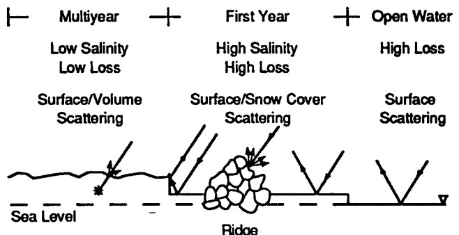
Fig. 5-1. Backscatter interactions for multiyear ice, first-year ice, and smooth open water.
