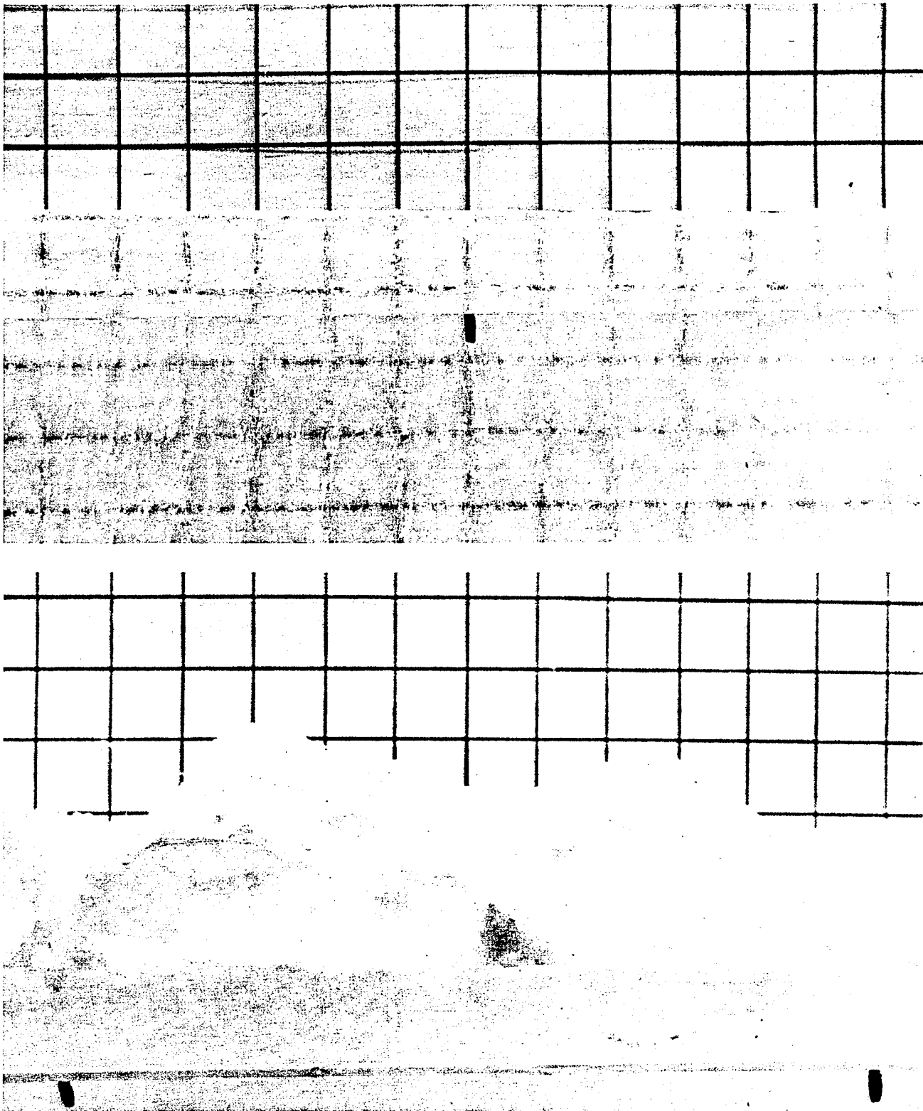
Fig. 9-28. Vertical thick sections showing the air-ice interface for (a) slightly rough and (b) very rough grey ice. The grid spacing is 1 cm.
