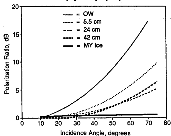
Fig. 5-16. The measured polarization ratio P_r = \sigma_{VV}/\sigma_{HH} at 5.25 GHz is shown as a function of incidence angle for open water, 5.5-, 24-, and 42-cm-thick first-year ice, and multiyear ice. The average rms deviation for these data is 0.7 dB.
