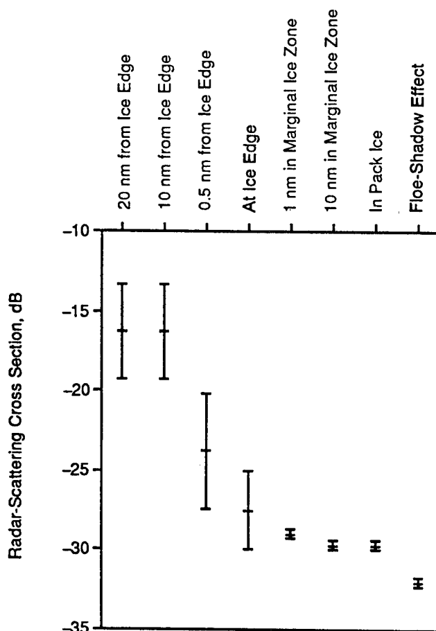
Fig. 5-10. Radar-scattering cross sections of the liquid ocean at 9.6 GHz, HH-polarization, and 25°, obtained as a function of position from the ice edge on July 5, 1984, in the marginal ice zone in the Fram Strait [Onstott, 1990a].
