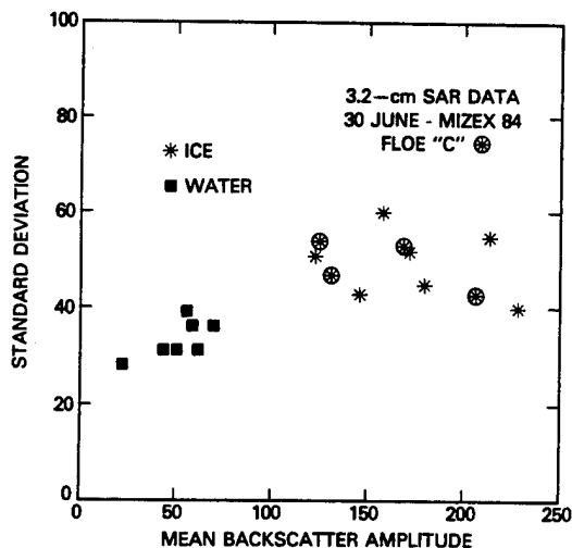
Fig. 8. SAR X-band (3.2 cm) image statistics for floe C area based on 60 × 60 m sample area.
