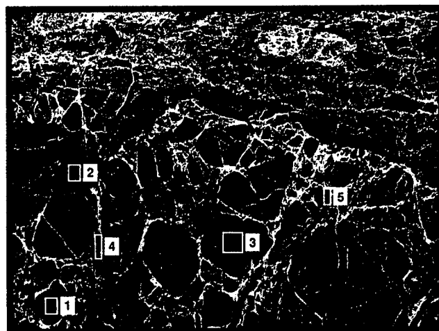
Fig. 24-1. Three-frequency total power image acquired by the JPL polarimeter at the location 73^\circ 13.4' N 142^\circ 1.1' W at 17:21:26 GMT (i.e., 08:21:26 local time) on March 11, 1988, in the Beaufort Sea [Drinkwater et al., 1991a]. These data are overlaid as a false-color image, with the C-band in blue, L-band in green, and P-band in red.
