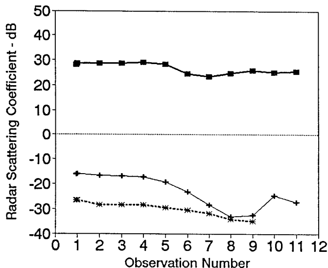
Figure 1. Time Series Response of the Backscatter Response at 5.25 GHz During the Evolution of Open Water to New Ice at Nadir and 40° (VV & HH).
