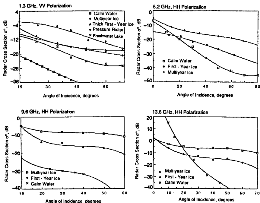
Fig. 5-19. Radar backscatter cross sections at L-, C-, X-, and Ku-bands during winter, illustrating the contrast in ice type and water signatures as a function of frequency and incidence angle.
