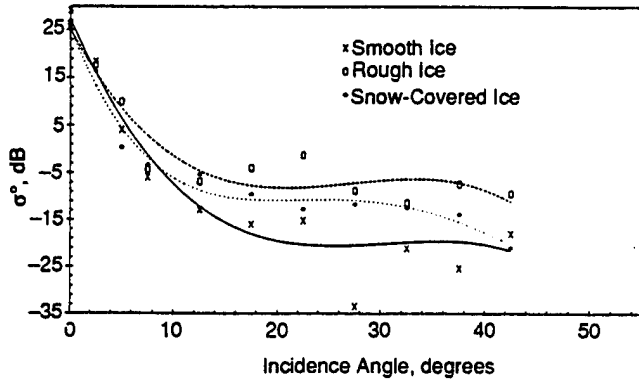
Fig. 9-33. Effects of surface conditions on backscatter angle response at 13.6 GHz and HH polarization.
