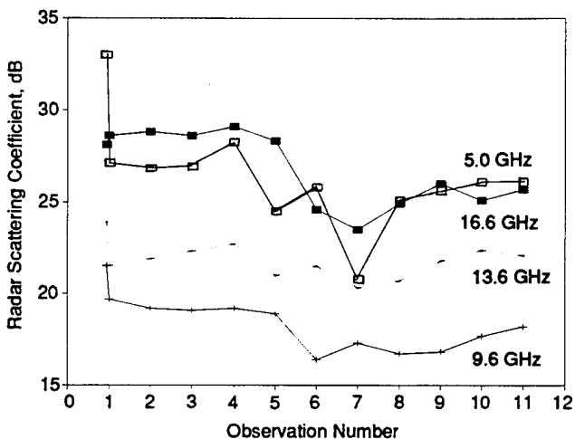
Fig. 9-10. The time series response of backscatter at vertical incidence during the evolution from open water to new ice shown as a function of frequency from 5.0 to 16.6 GHz.
