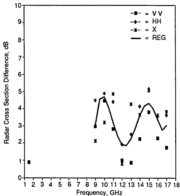
Fig. 5-13. The difference in radar-scattering coefficients for the case of thick first-year ice with and without an 8-cm snow layer. These data represent the average backscatter difference for angles between 20° and 60°. (X = cross-polarization.)
