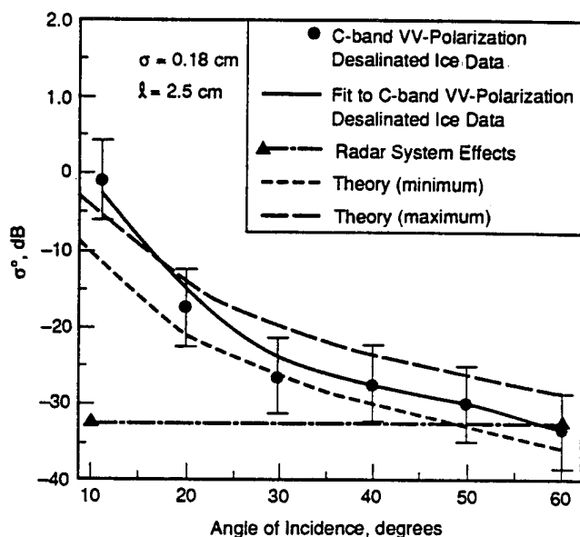
Fig. 9-21. Backscatter cross section of desalinated ice sheet at C-band, as determined from data obtained during CRRELEX'88, compared with predictions of the Small Perturbation Method.
