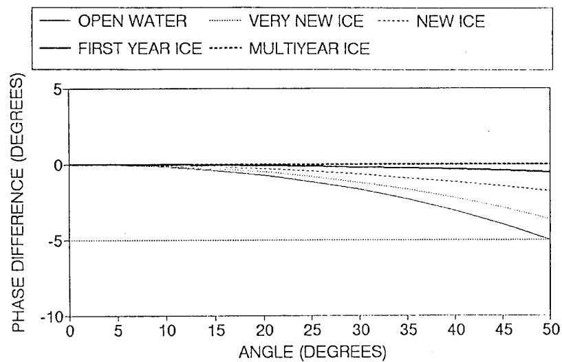
Figure 2. The Phase Difference Ratio ( \theta_{HH/VV} ) for Open Water, Very New Ice, New Ice, First Year Ice, and Multiyear Ice has Been Calculated Based on the Small Perturbation Model and Measured Dielectric Constants.
