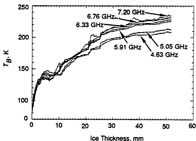
Fig. 9-14. Brightness temperature of CRRELEX'88 sheet 1B versus thickness at the six C-band frequencies of the Stepped Frequency Microwave Radiometer. The measurements were taken at horizontal polarization and a 35° incidence angle. Data from Figure 9-13 are included here without the associated uncertainty bars.
