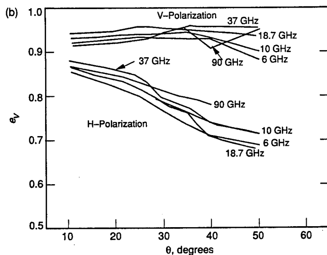
Fig. 9-23. (a) Emissivity spectra from 6 to 90 GHz of a desalinated ice sheet at V- and H-polarizations. (b) Microwave emissivity versus incidence angle for the desalinated pond ice. Curves give the results for the five observation frequencies.
