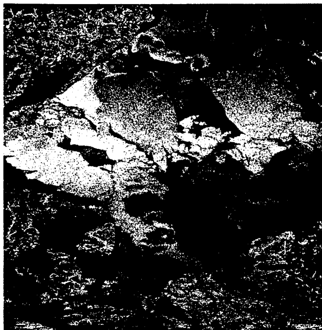
Fig. 5-27. Ice floe imagery obtained on March 20, 1989, during CEAREX with the ERIM/NADC P-3 C-band (5.3-GHz) SAR. Features include open water, nilas, gray ice, and multiyear ice. The majority of the image is composed of gray ice of various ages and thicknesses. The brighter the image intensity, the thicker the ice sheet. The polarization is VV, and the incidence angle range goes from 20° to 70°.
