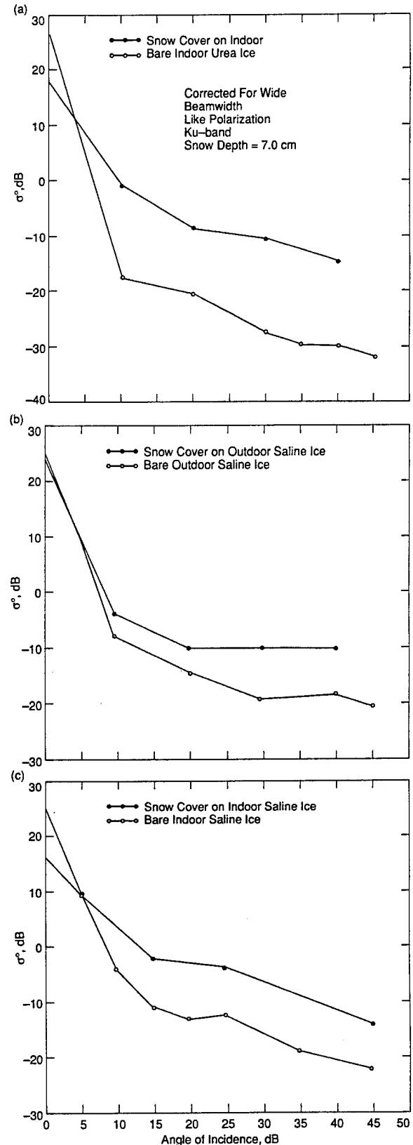
Fig. 9-37. Angular response of the backscatter coefficient at 13.9 GHz for three different bare and then snow-covered ice sheets: (a) urea grown indoors; (b) saline grown outdoors; and (c) saline grown indoors.
