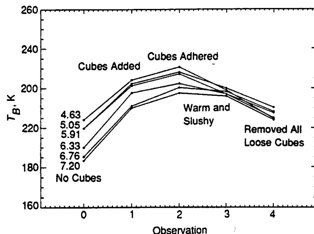
Fig. 9-31. C-band brightness temperature with varying surface roughness. Observation 1 was made immediately after adding approximately 2.5 cm of ice cubes to a 13.2-cm-thick ice sheet. Observation 2 was made the following morning, after most cubes had become frozen to the ice surface. Three hours later, the surface temperature had increased to -4^\circ\text{C} for observation 3. Finally, for the last observation, the surface was raked to remove all loose cubes.
