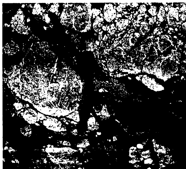
Fig. 5-26. Ice floe imagery obtained on March 21, 1989, during CEAREX with the ERIM/NADC P-3 SAR. Features include open water, nilas, gray ice, and multiyear ice. The polarization is VV and the incidence angle range goes from 20^\circ to 70^\circ . (a) An L-band (1.2-GHz) image, (b) a C-band (5.3-GHz) image, and (c) an X-band (9.4-GHz) image.
