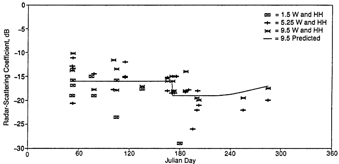
Fig. 5-23. Seasonal backscatter response for first-year sea ice at 1.5, 5.25, and 9.5 GHz, an angle of 40^\circ , and like-polarization (VV or HH).
