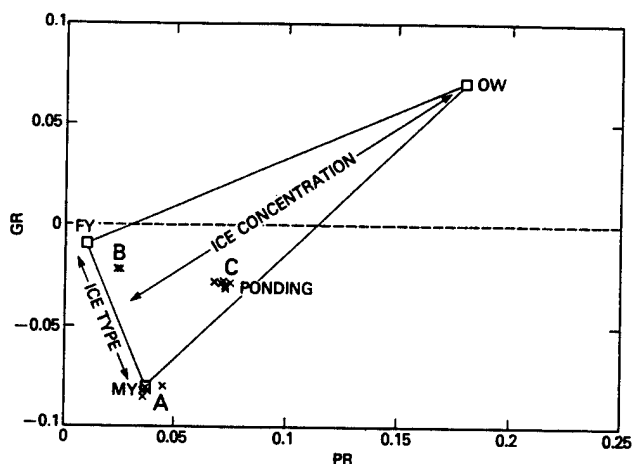
Fig. 7. GR versus PR plot for 30 June, 1984, showing clusters of measurements corresponding to floes A, B, and C shown in Figure 5.
