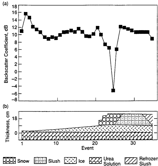
Fig. 9-36. (a) Evolution of backscatter coefficient with successive, controlled changes in ice sheet properties. Data were collected with a 13.9-GHz radar operating at normal incidence over an indoor tank filled with an urea solution. (b) The initial formation of ice from the melt (event 1) through the point at which the ice was about 9 cm thick (event 21) is shown. Events 22, 23 and 24 represent the addition of three snow layers. Event 25 represents the moment at which flooding begins.
