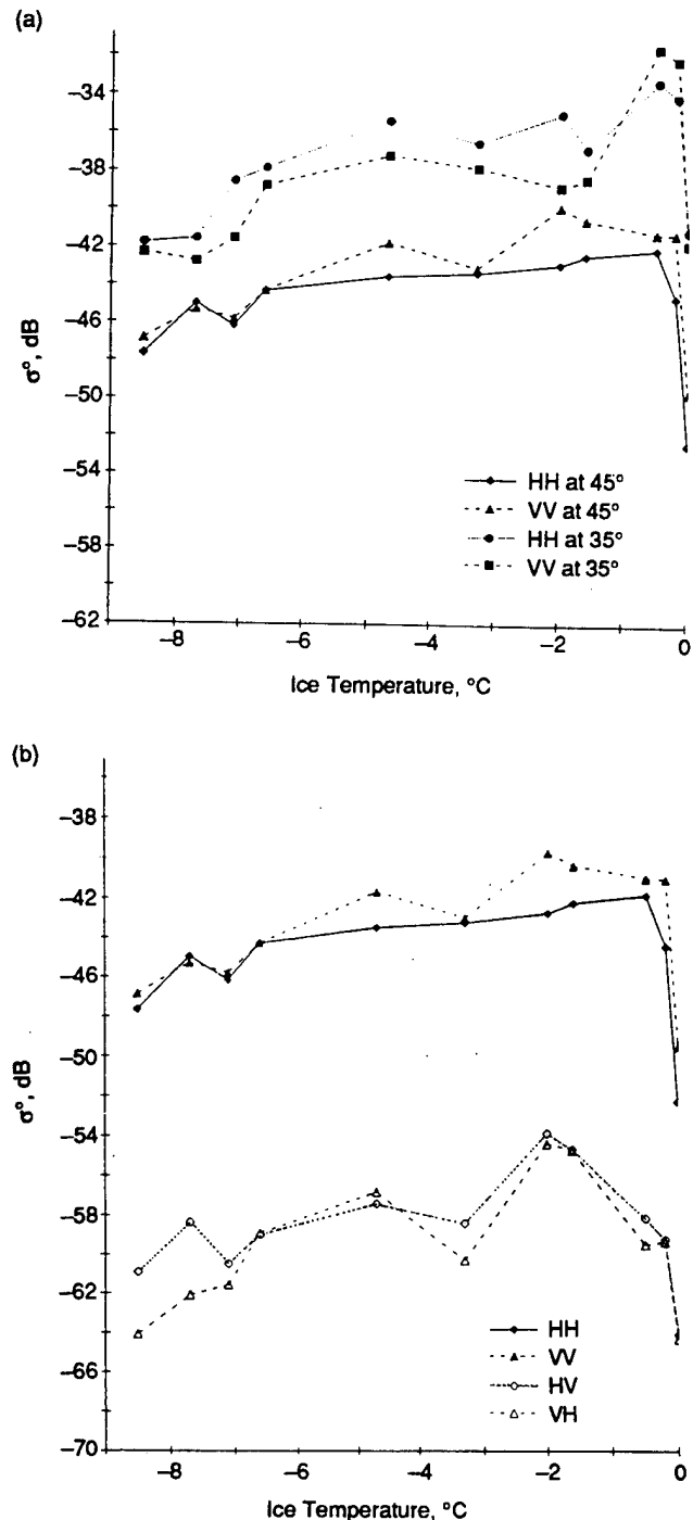
Fig. 9-18. Normalized radar cross section ( \sigma^0 ) versus ice temperature at (a) 35° and 45°, and (b) polarimetric cross sections at 45° [Colom, 1991].
