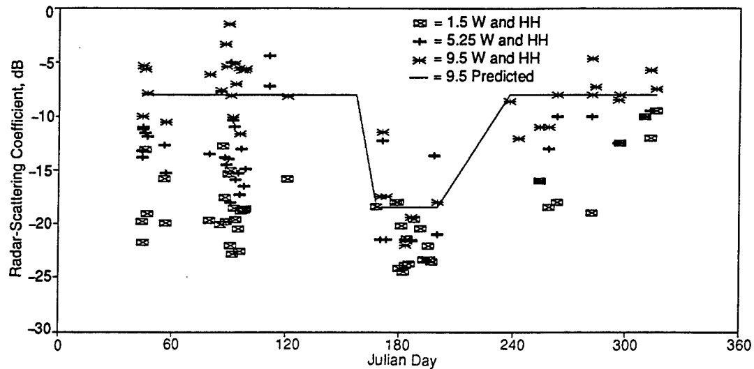
Fig. 5-22. Seasonal backscatter response for multiyear sea ice at 1.5, 5.25, and 9.5 GHz, an angle of 40^\circ , and like-polarization (VV or HH). (W = water.)
