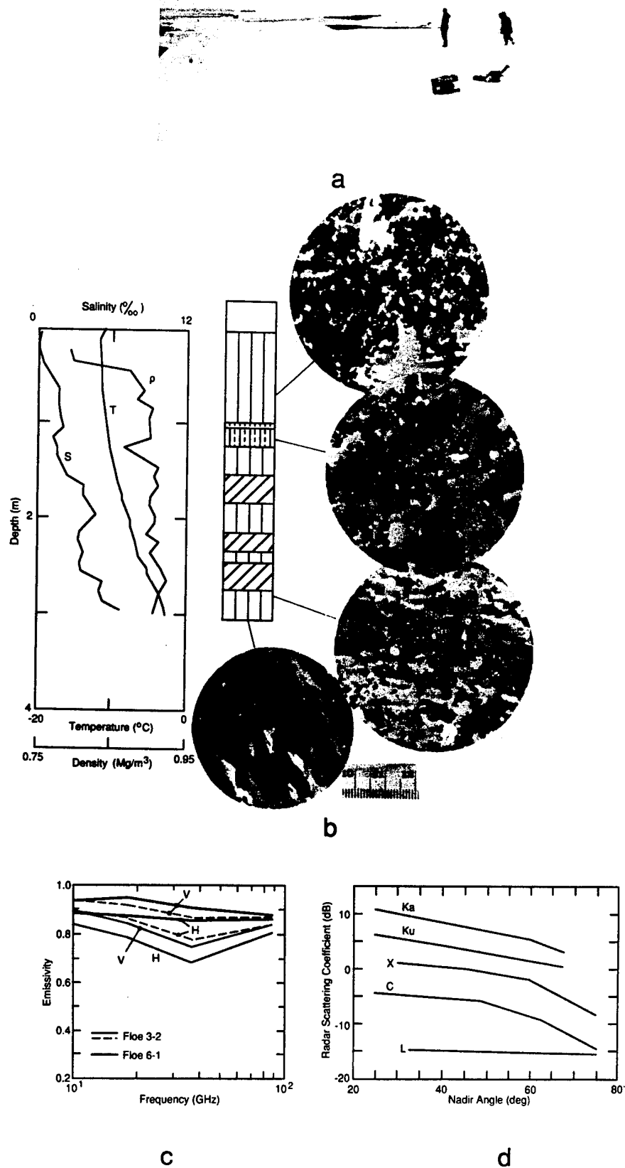
Fig. 6. Multiyear ice, April 3, 1987: (a) photograph of site (b) properties and structural profile, (c) emissivity, and (d) backscatter coefficient. Two emissivity spectra are presented for this site (3-2) in addition to that from another multiyear site (6-1).
