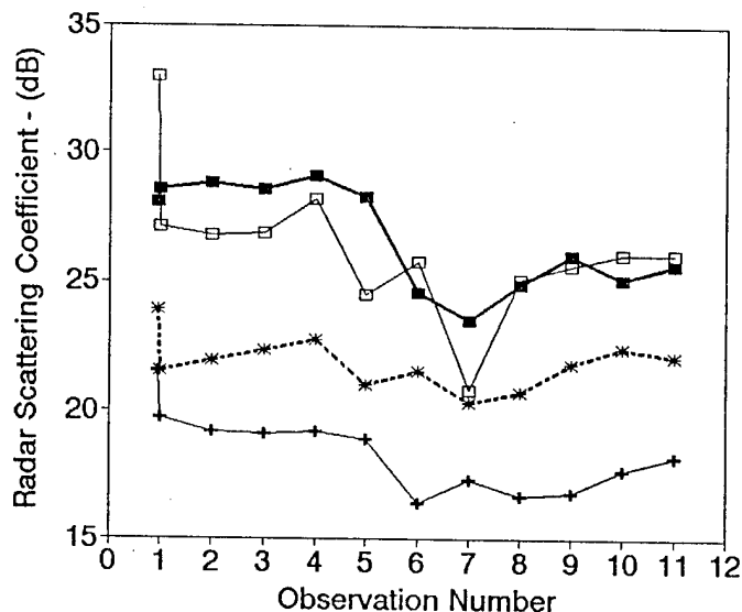
Figure 3. Time Series Response of the Backscatter at Vertical During the Evolution of Open Water to New Ice Shown as a Function from 5.25 GHz to 16.6 GHz.
