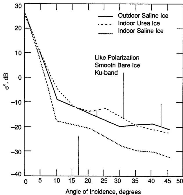
Figure 9-17. Beamwidth corrected backscatter coefficients for two saline ice sheets and an urea ice sheet. One of the saline sheets and the urea ice sheet were grown indoors. The second saline sheet was grown on an outdoor pond.
