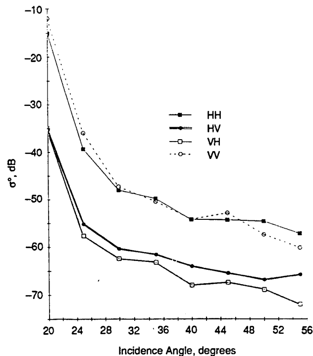
Fig. 9-16. Polarimetric normalized radar cross section ( \sigma^\circ ) of smooth urea ice at 35 GHz [Colom, 1991].
