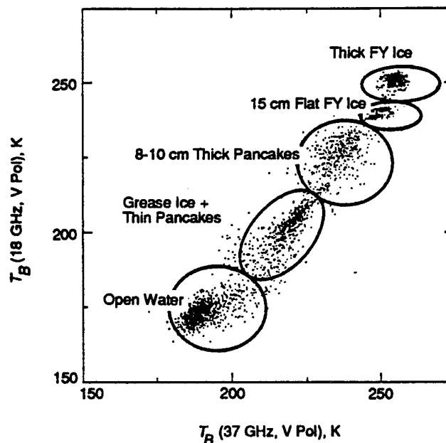
Fig. 14-6. Cluster observations of some thin ice types and first-year ice from MIZEX'87 in the northern Greenland Sea [Grenfell, T. C. and D. L. Bell, unpublished, University of Washington, Seattle, Washington, 1988]. V-pol observations are at a nadir angle of 50^\circ .
