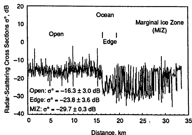
Fig. 5-9. Transect across the ice edge on July 5, 1984, at 9.6 GHz, HH-polarization, and 25° in the marginal ice zone in the Fram Strait [Onstott, 1990a].
