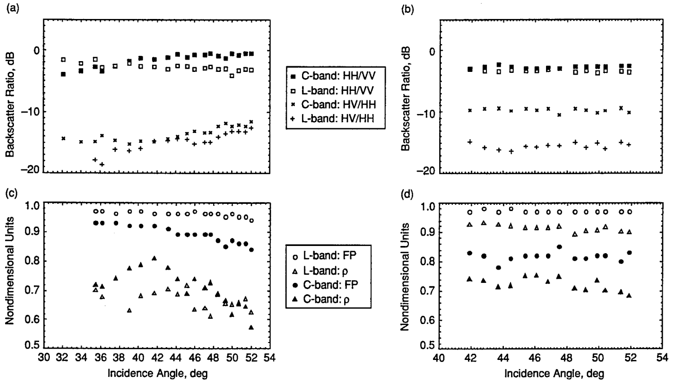
Fig. 24-4. Cross-swath C- and L-band polarimetric discriminant statistics. The upper panels show co- and cross-pol ratios in the Beaufort Sea for (a) FY and (b) MY ice. The lower panels show the correlation coefficient \rho between hh- and vv-pol returns and the corresponding fractional polarization (FP) for samples of (c) FY and (d) MY ice.
