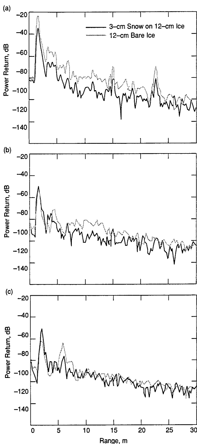
Fig. 9-38. Time domain response for a 13.9-GHz radar over bare and snow-covered saline ice. (a) The nadir signal from the ice surface corresponds to the large peak near the far left side. At (b) 25° and (c) 45° incidence angles, the backscattered signal with a slight time delay at oblique incidence also appears on the left side of each figure.
