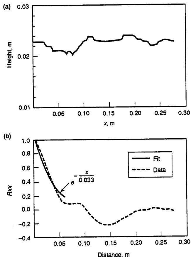
Fig. 9-19. For desalinated ice blocks studied during CRRELEX'89: (a) surface profiles, and (b) computed autocorrelations and minimum-mean-square-exponential fits.
