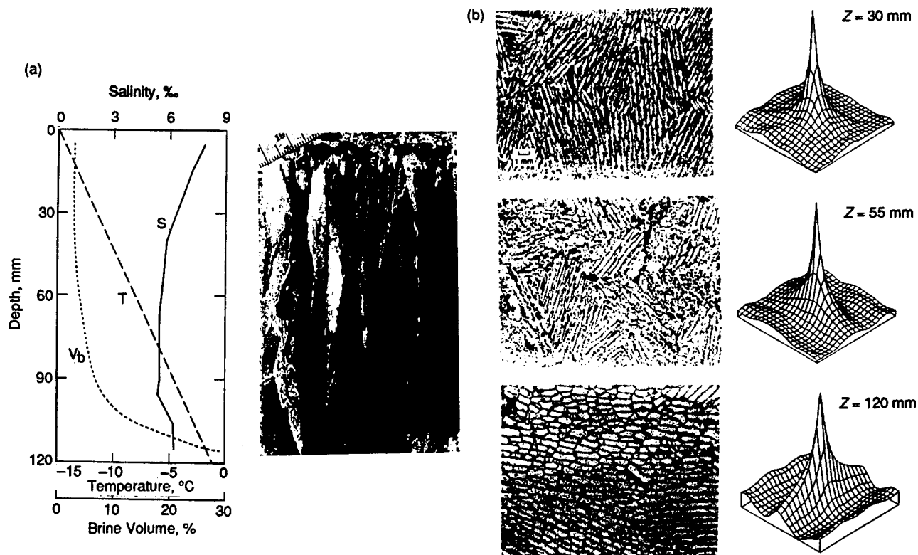
Fig. 9-5. Vertical profiles of temperature (T), salinity (S), and brine volume ( V_b ) for young sea ice. The vertical thin section shows that the ice structure is predominantly columnar with a thin surface layer of frazil. Also shown are horizontal thin sections from the top, middle, and bottom of the ice sheet with corresponding correlation functions [Perovich and Gow, 1991].
