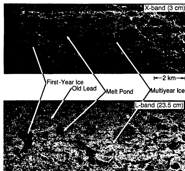
Fig. 5-30. Ice floe imagery obtained in July 1983, during MIZEX'83 at X-band (9.4 GHz) and L-band (1.2 GHz). Surface features include first-year ice, an old refrozen lead, a melt pond, and multiyear ice.
