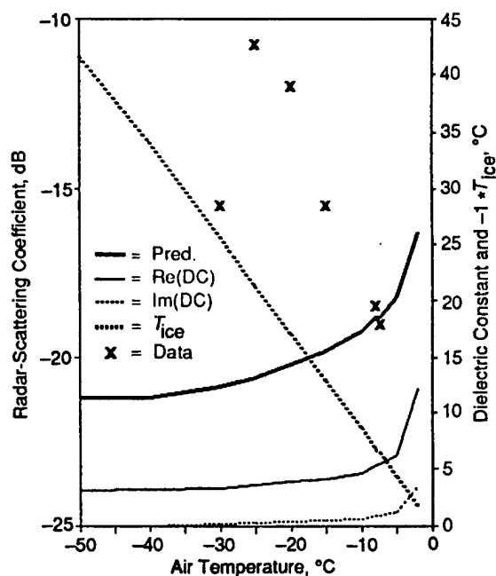
Fig. 5-11 Predicted and measured backscatter for first-year ice (1-m thickness) for air temperature from -50^{\circ} to -2^{\circ}\text{C} . The frequency is 9.6 GHz and the incidence angle is 40^{\circ} . (Pred. = predicted, Re(DC) = real part of complex dielectric constant, IM(DC) = imaginary part of complex dielectric constant, and T_{ice} = ice surface temperature.)
