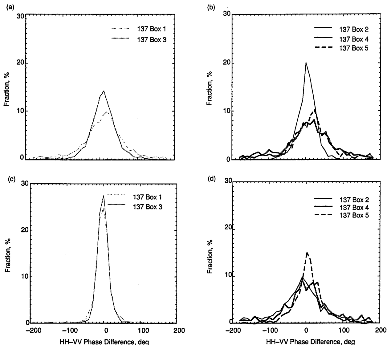
Fig. 24-5. Normalized C- and L-band hh-vv phase difference distributions derived from single pixel values from the boxes in Figure 24-1. Upper panels show C-band distributions for (a) the MY and (b) FY ice; the lower panels contrast L-band distributions of the same (c) MY and (d) FY examples.
