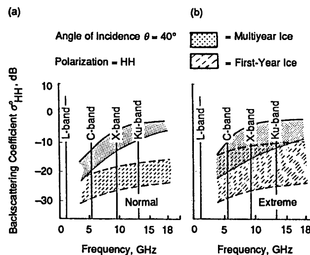
Fig. 5-18. Frequency dependence of the backscatter coefficient for first-year and multiyear ice at 40°. Theoretical \sigma^{\circ} for sea ice under (a) normal-winter and (b) extreme-summer conditions.
