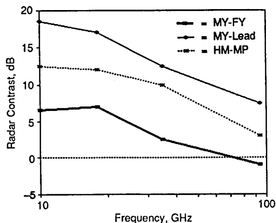
Fig. 5-33. The differences between radar-scattering coefficients of multiyear ice, first-year ice, lead ice (30-cm thick), and a multiyear hummock and melt pool are shown for fall conditions. The incidence angle is 40°, and the polarization is VV.
