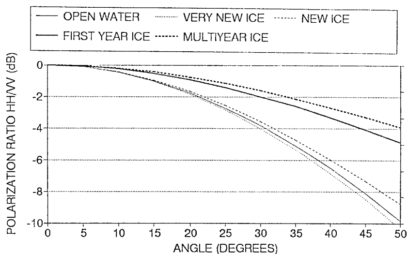
Figure 1. The Polarization Ratio ( \sigma^{\circ}_{HH}/\sigma^{\circ}_{VV} ) for Open Water, Very New Ice, New Ice, First Year Ice, and Multiyear Ice has Been Calculated Based on the Small Perturbation Model and Measured Dielectric Constants.
