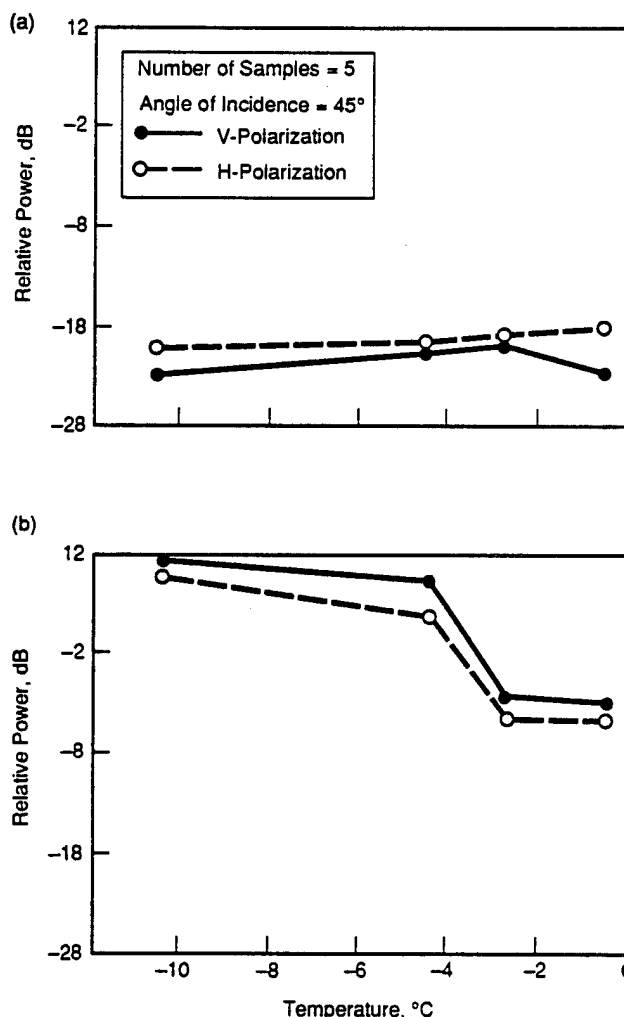
Fig. 9-22. Effect of temperature on backscatter from desalinated ice at (a) C-band and (b) X-band as determined from data obtained during CRRELEX'88.
