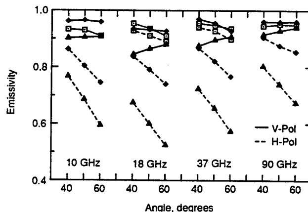
Fig. 9-27. Comparative spectra showing the effects of surface roughness for the natural surface (diamonds), the same surface after roughening (squares), and after the rough upper surface was scraped off (triangles) [Grenfell and Comiso, 1986].
