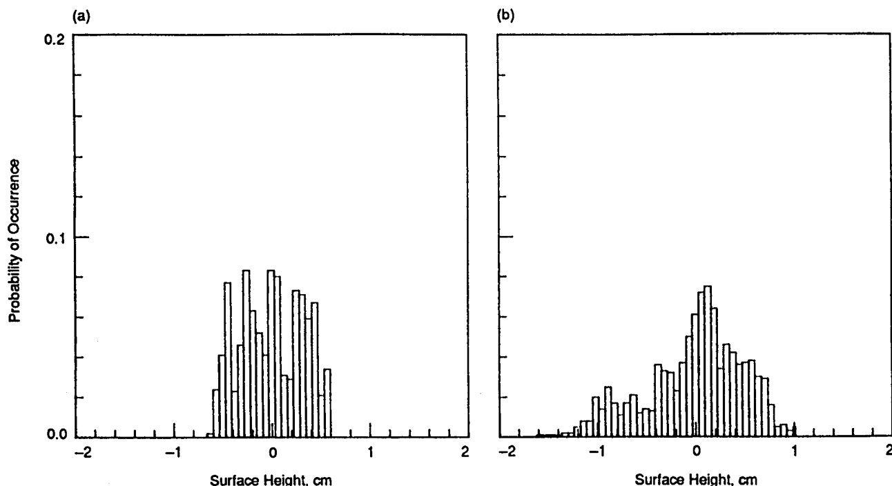
Fig. 5-24. First-year surface height histograms for a homogeneous ice sheet. (a) Data acquired June 14 are typical of early summer pre-melt, late fall, winter, and spring conditions. Height range, variance, and skewness were 0.932 cm, 0.044 \text{ cm}^2 , and 0.0003, respectively. (b) Data acquired June 20 are typical of early summer melt conditions. Superimposed ice increases the height range to 2.778, the variation to 0.243, and skewness to -0.588 [Onstott and Gogineni, 1985].
