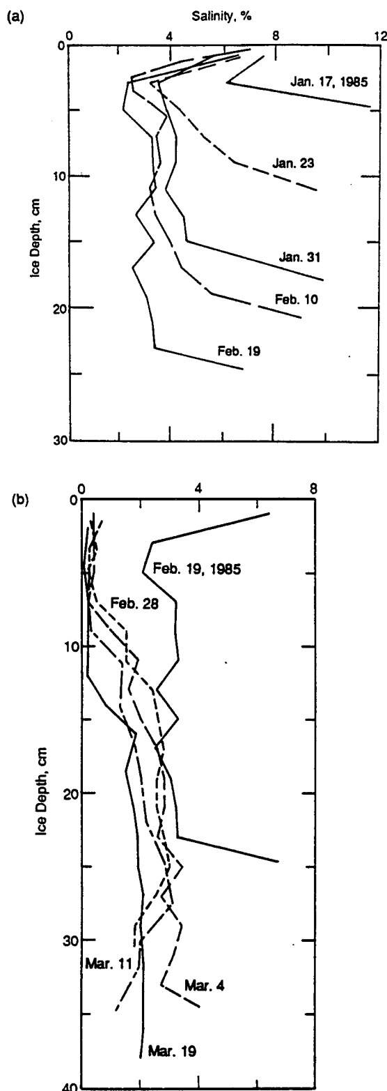
Fig. 9-4. (a) Salinity profiles at different stages of growth of sea ice grown in an outdoor pond at CRREL. Profiles closely simulate those found in Arctic first-year ice. (b) Transformation from a new ice to desalinated ice salinity profile in the outdoor pool at CRREL.
