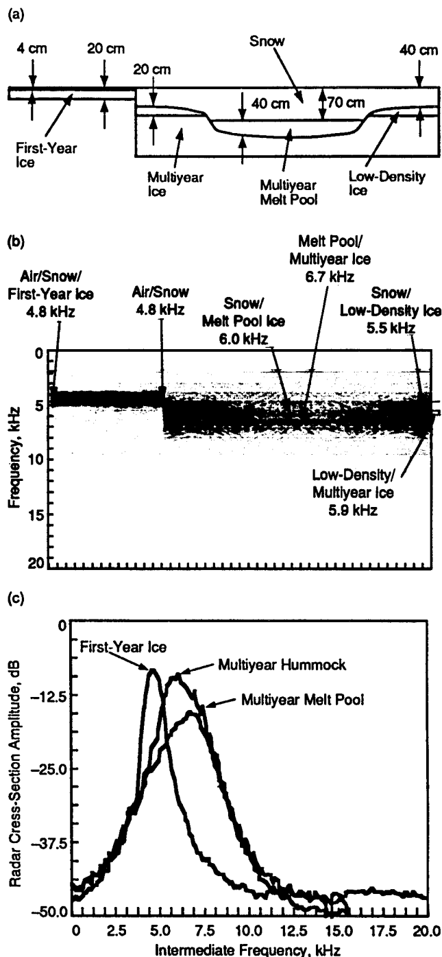
Fig. 5-7. The origin of backscatter in multiyear and first-year ice is illustrated with a probing radar scanned across a 40-m ground track. (a) The surface truth diagram is shown. (b) The backscatter response at 5.25 GHz, 45° incidence angle, and VH-polarization is shown as a function of ground position. (c) Average intensity responses for the first-year ice, hummock, and melt pool versus interior ice position are also shown. Intermediate frequency is proportional to the range at approximately 1750 KHz/m of ice.
