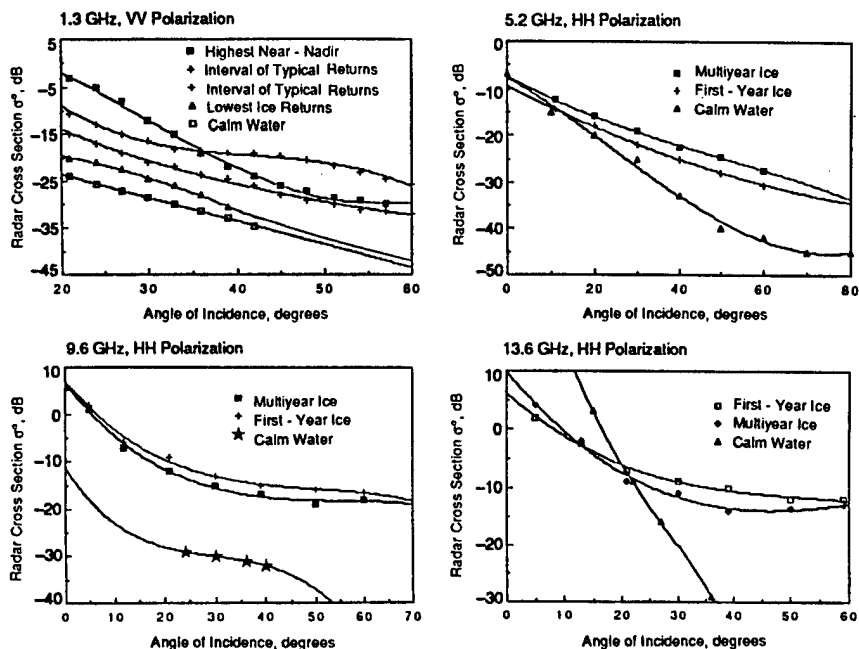
Fig. 5-20. Radar backscatter cross sections at L-, C-, X-, and Ku-bands during summer, illustrating the contrast in ice type and water signatures as a function of frequency and incidence angle.
