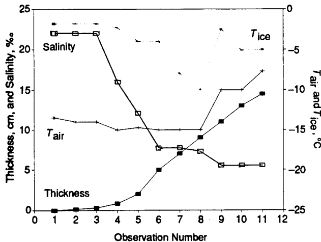
Fig. 9-9. Ice thickness, air temperature, ice temperature, and bulk salinity during the evolution of open water to new ice.
