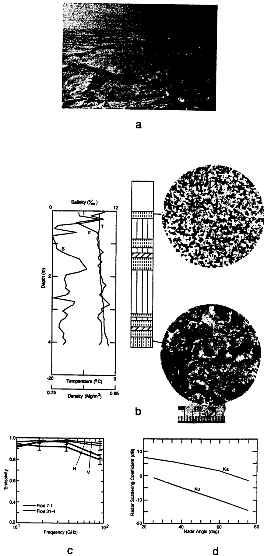
Fig. 7. Flooded multiyear ice, April 7, 1987: (a) photograph of floe, (b) properties and structural profile, (c) emissivity, and (d) backscatter coefficient. Emissivity spectra are shown for this site plus an additional flooded multiyear floe.
