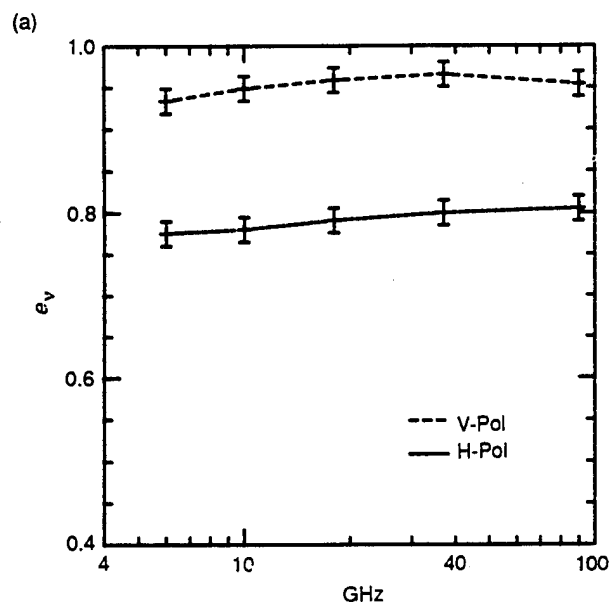
Fig. 9-24. Microwave emissivity versus frequency for the desalinated blocks in January 1989. The error bars denote the standard deviation for four independent samples.
