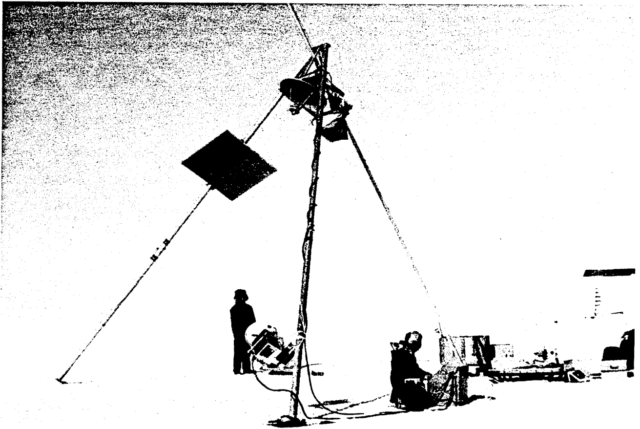
Fig. 5-2. TRAMAS was the first in-situ active microwave system to obtain measurements of sea ice, and was developed in 1976 at the University of Kansas [Onstott et al., 1979].
