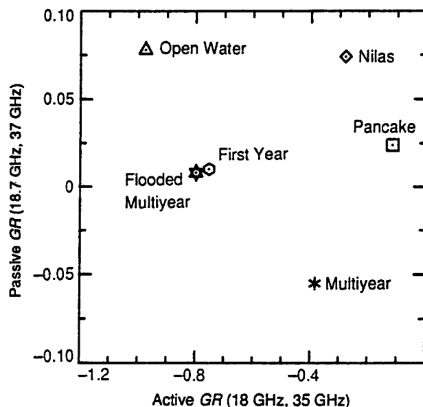
Fig. 14-14. Comparison of microwave observations for selected ice types measured during MIZEX'87 in the northern Greenland Sea in early spring.
