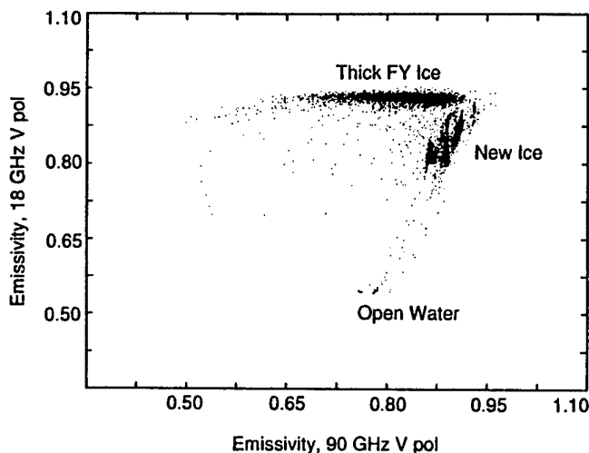
Fig. 14-7. Scatter plot of emissivities for thin ice obtained during the winter of 1986 in the Weddell Sea. New ice indicates nilas in different stages of development—undisturbed and overthrust with and without snow cover.
