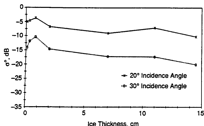
Fig. 9-7. Effects of ice growth on vertical polarization \sigma^\circ at 5.3 GHz.
