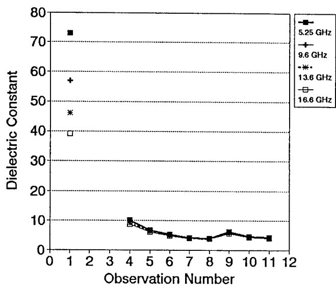
Figure 5. Predicted Magnitudes of the Complex Dielectric Constant ( \epsilon_r' ).
