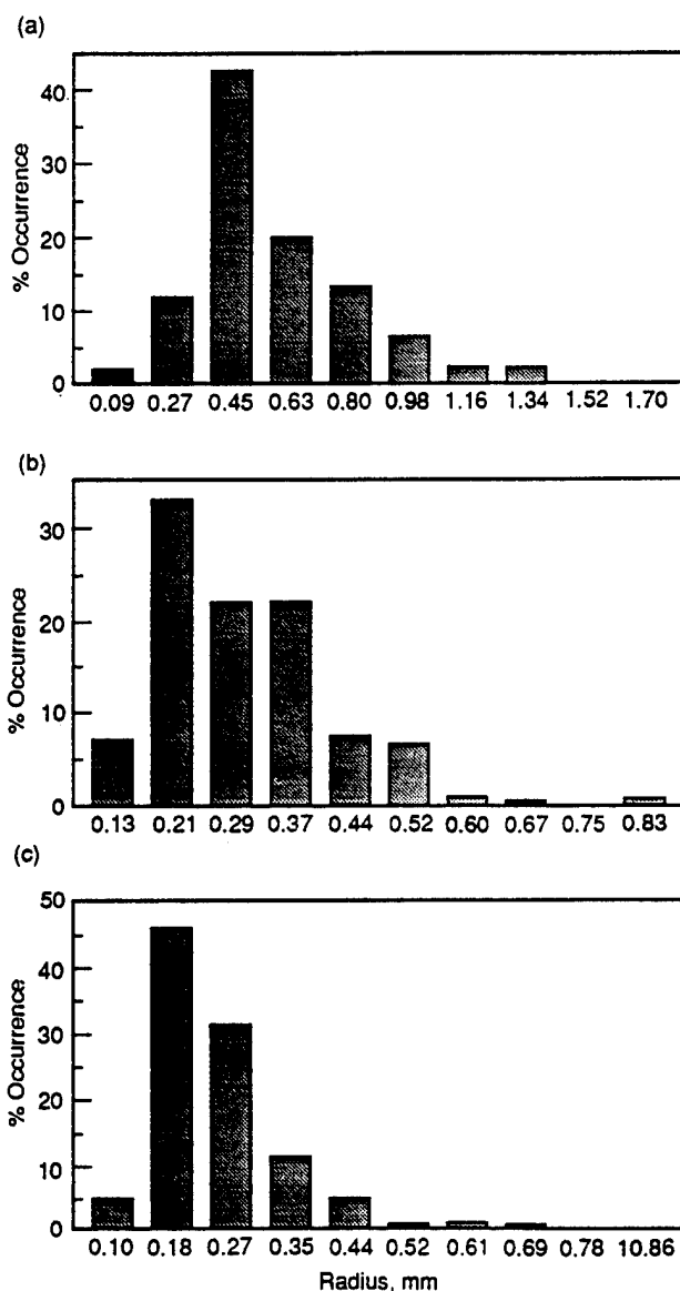
Fig. 9-20. Air-bubble size distribution from the (a) top, (b) middle, and (c) bottom of a block of desalinated ice studied during CRRELEX'89.
