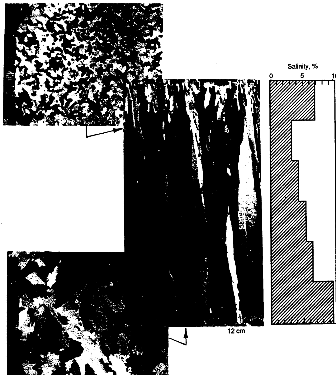
Fig. 9-2. The ice shown in these vertical and horizontal thin-section photographs and salinity profile is freshly grown saline ice from the CRREL test pond. Structurally, this ice closely simulates young Arctic sea ice. Scale subdivisions in horizontal sections measure 1 mm.
