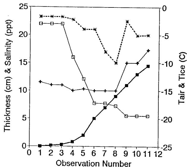
Figure 2. Ice Thickness, Air Temperature, Ice Temperature and Bulk Salinity During the Evolution of Open Water to New Ice.
