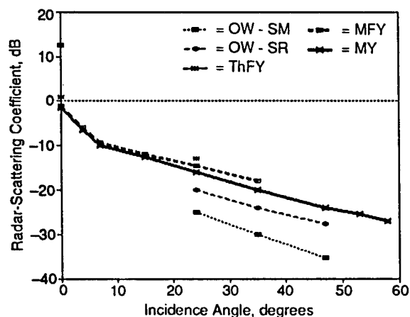
Fig. 5-25. The angular response at 5.25 GHz and HH-polarization for midsummer shown for open water, thin first-year (ThFY), medium first-year (MFY), and multiyear ice. The letters OW-SR indicate open water that is slightly rough, whereas OW-SM indicates open water that is smooth.
