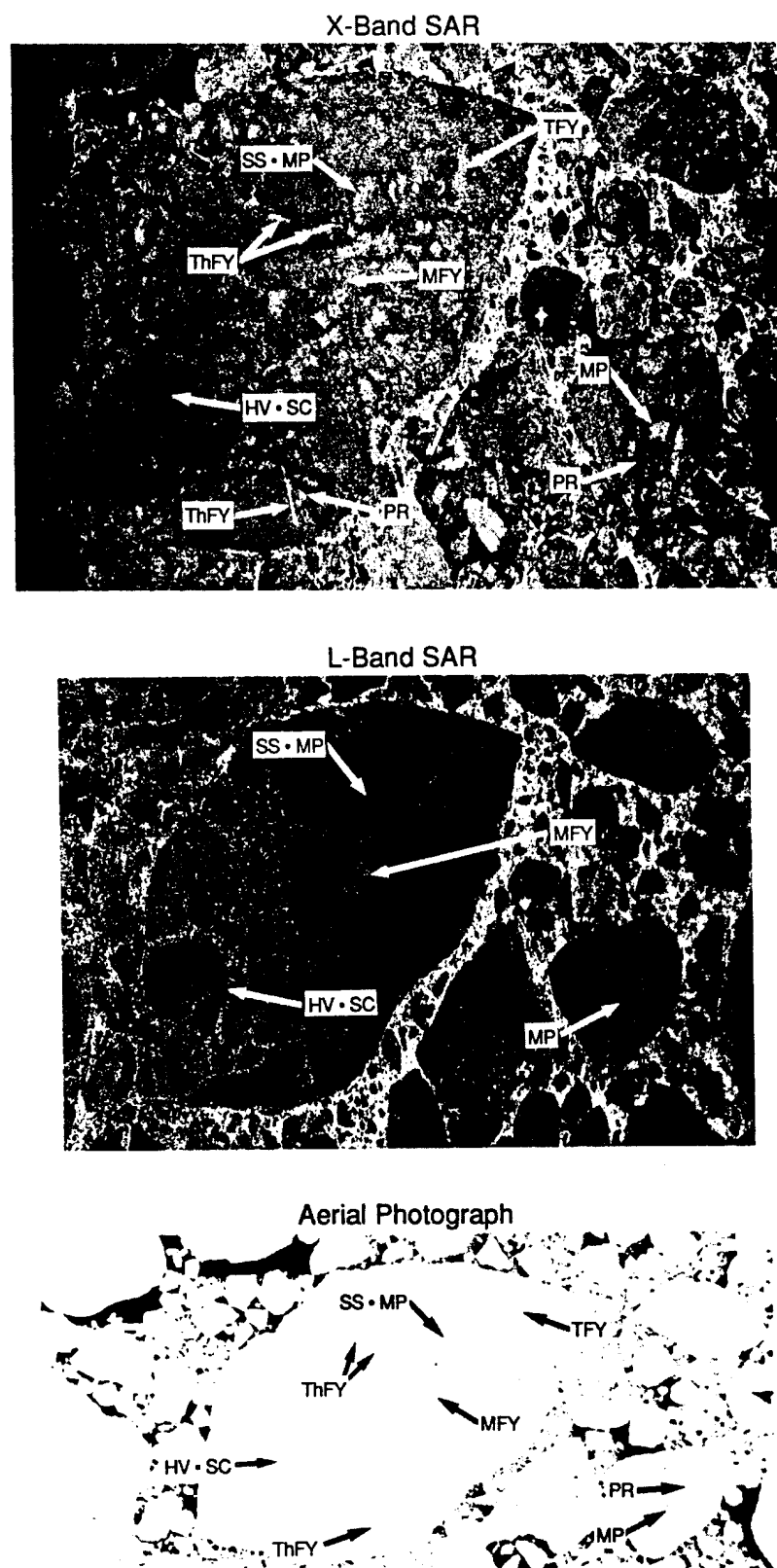
Fig. 10. Annotated ice floe imagery obtained on 29 June, 1984, with the ERIM X-band (9.4 GHz) and L-band (1.2 GHz) SAR and the CCRS aerial camera on the CV-580. Surface features include snow-covered ice (SCI); heavy-snow covered ice (HV.SC); thick (TFY), medium (MFY), and thin (ThFY) first-year ice; pressure ridges (PR); subsurface melt ponds (SS.MP); and melt ponds (MP).
