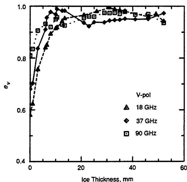
Fig. 9-12. Ice emissivity versus thickness for 18-, 37-, and 90-GHz vertical polarizations during initial growth of congelation ice [Grenfell et al., 1988].
