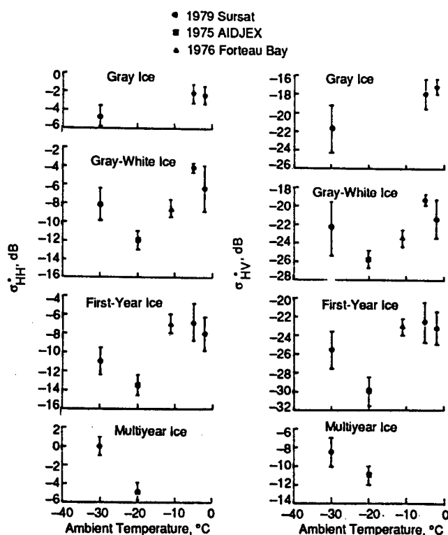
Fig. 5-12. Temperature dependence of \sigma_{\text{HH}}^{\circ} ( \theta \approx 25^{\circ} ) and \sigma_{\text{HV}}^{\circ} ( \theta \approx 25^{\circ} ) for gray, gray-white, first-year and multiyear ice [Livingstone et al., 1983].
