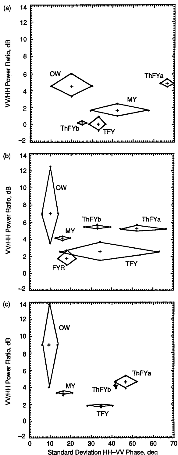
Fig. 24-7. Classification feature space for (a) C-band, (b) L-band, and (c) P-band, indicating the separability of ice types and open water using a polarimetric feature combining the spread in the hh-vv phase difference and the vv/hh power ratio. The categories are thin first-year ice (ThFYb), anomalous thin ice surfaces (ThFYa), thick first-year ice (TFY), rough Bering Sea first-year ice (FYR), multiyear ice (MY), and open water (OW).
