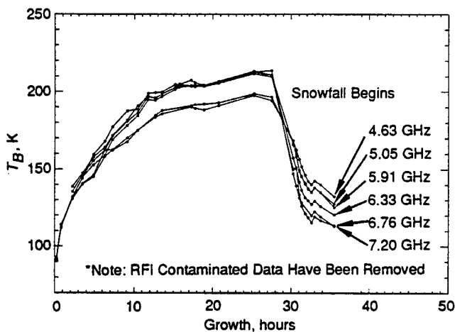
Fig. 9-34. C-band brightness temperature measurements illustrate the effect of light snowfall on a sheet of frazil ice. The snow thickness reached only 1 cm and became very moist over time.
