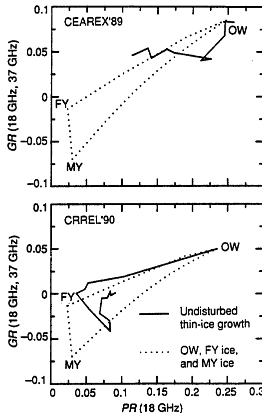
Fig. 14-10. Results for new ice from the northern Greenland Sea (CEAREX'89) and for young ice at the CRREL pond (CRREL'90).
