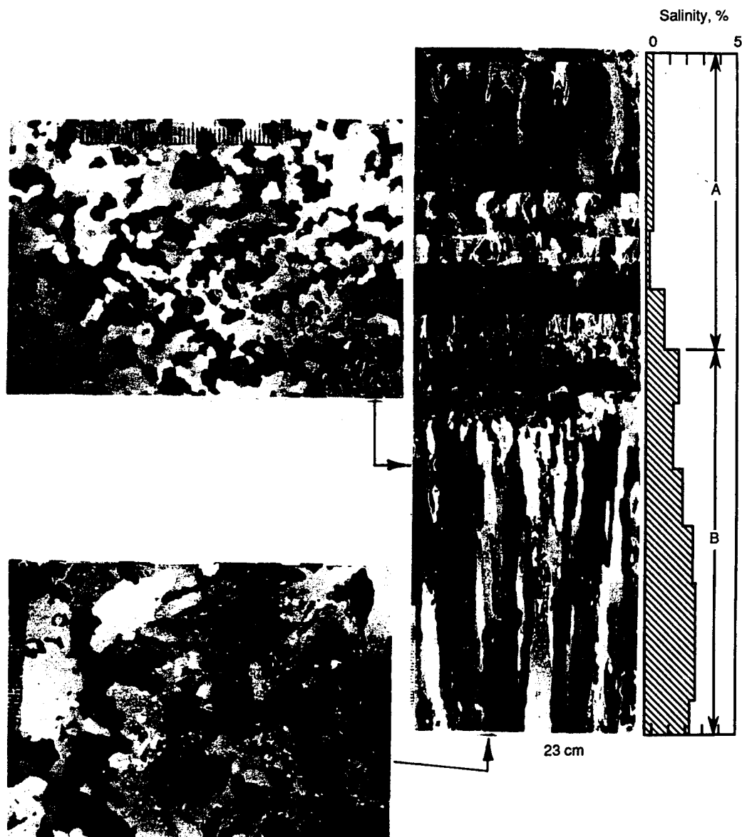
Fig. 9-3. Crystalline structure and salinity characteristics of ice desalinating in the CRREL test pond. In this example, several layers of melt pond ice (A) overlie desalinated columnar saline ice (B). Scale subdivisions in horizontal sections measure 1 mm.
