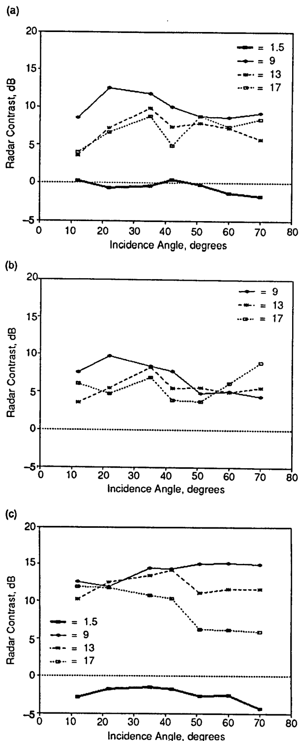
Fig. 5-32. The contrast in scattering coefficients of multiyear and first-year ice is shown as a function of polarization, angle, and frequency. In (a) the polarization is VV, in (b) it is HH, and in (c) it is VH.
