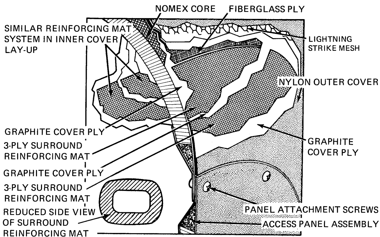
Figure 29. Access Panel Surrounding Reinforcement.
