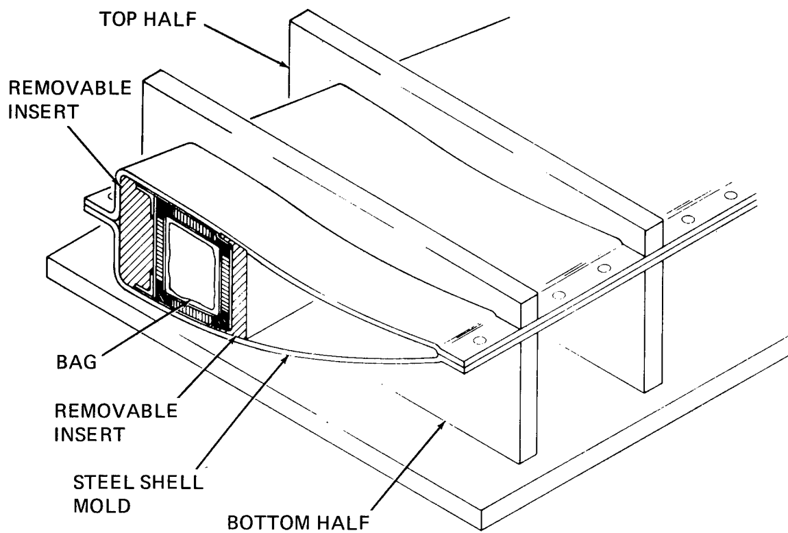
Figure 26. Fabrication of Vertical Fin Torque Box.
