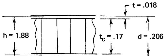
Figure 47. Forward Honeycomb Panel Section.
