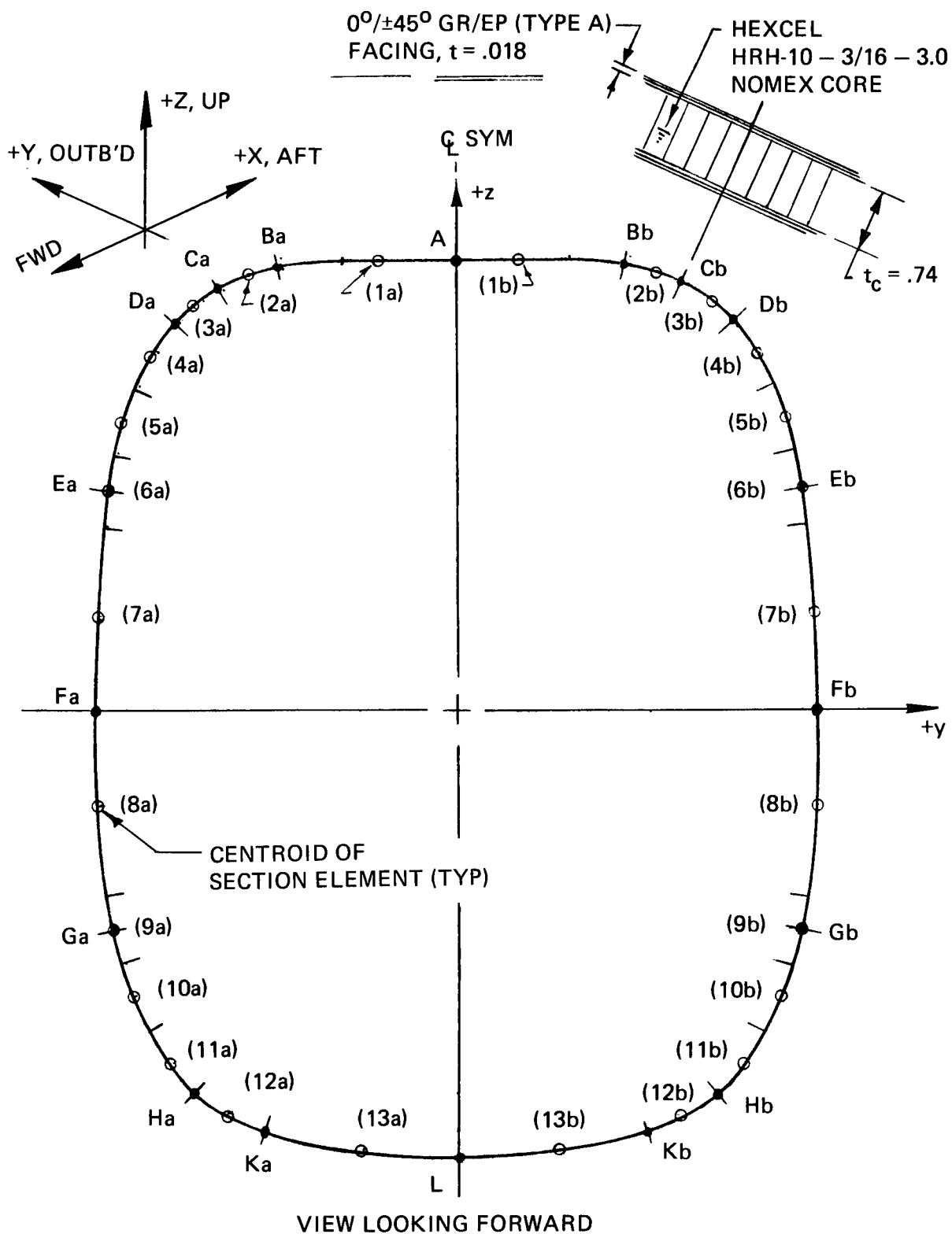
Figure 41. Concept 1 - Section Through Tail Boom.
