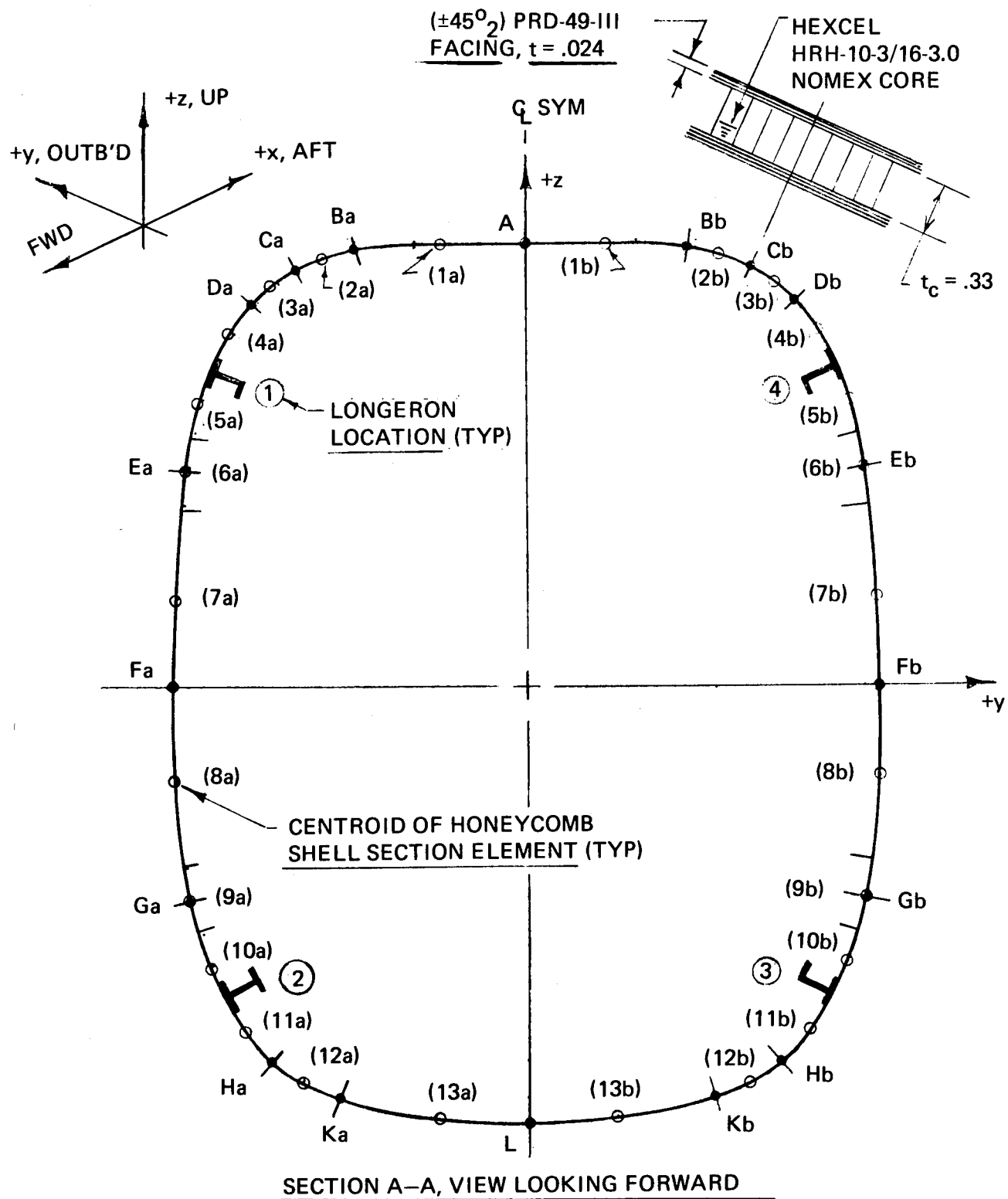
Figure 54. Concept 2 - Section Through Tail Boom.
