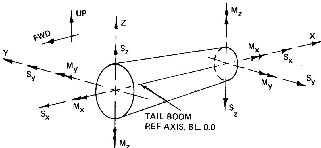
Figure 15. Sign Convention.
