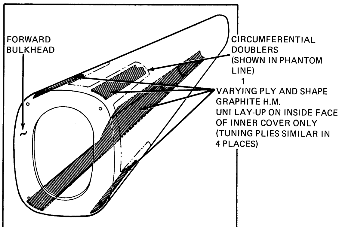
Figure 28. Structural Tuning System and Circumferential Doublers.
