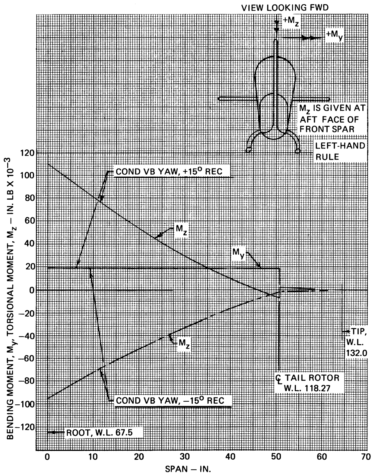
Figure 21. Vertical Fin Chordwise Bending and Torsional Moments.
