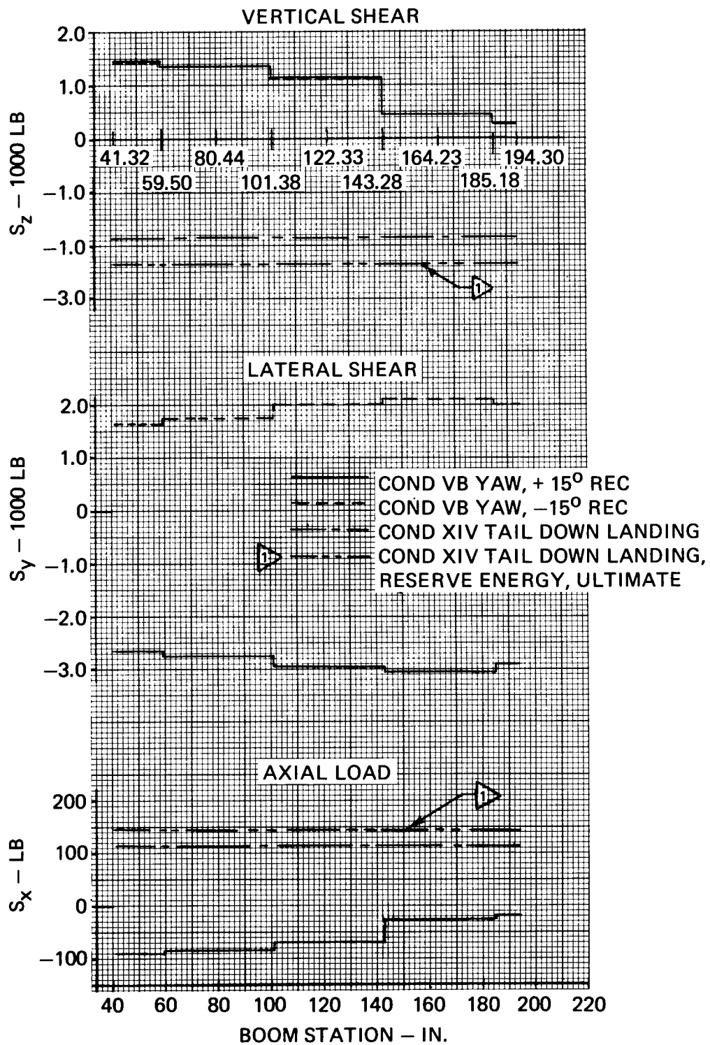
Figure 17. Tail-Boom Structural Strength.
