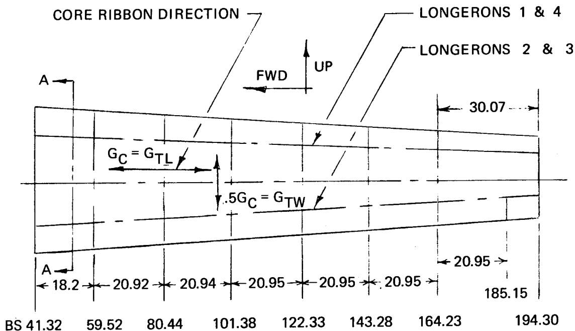
Figure 53. Longerons and Frame Spacing Geometry BS 41.32 - 194.30.
