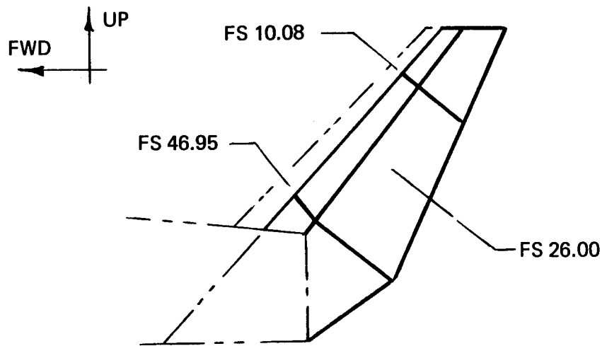
Figure 46. Vertical Fin Geometry.
