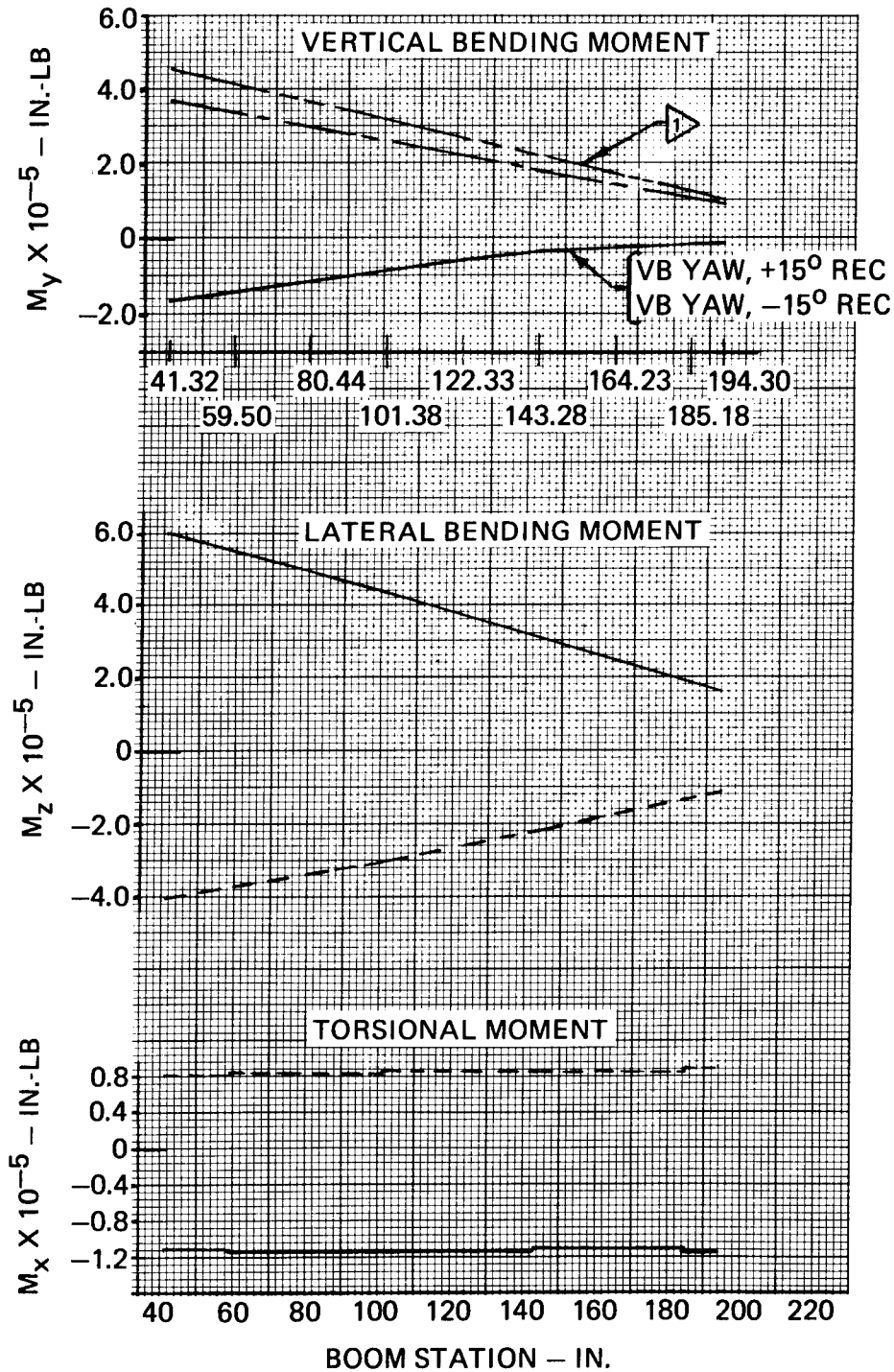
Figure 18. Tail-Boom Bending and Stiffness.
