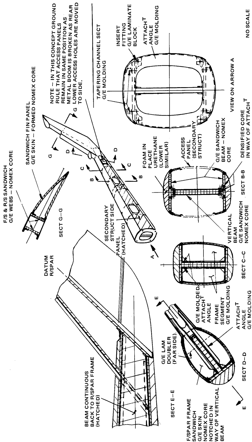
Figure 8. I-Beam Primary Structure-Secondary Side Panels.
