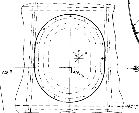
VIEW ON ARROW A SCALE 1/2" = 2 3/8" FWD LOWER ACCESS PANEL
