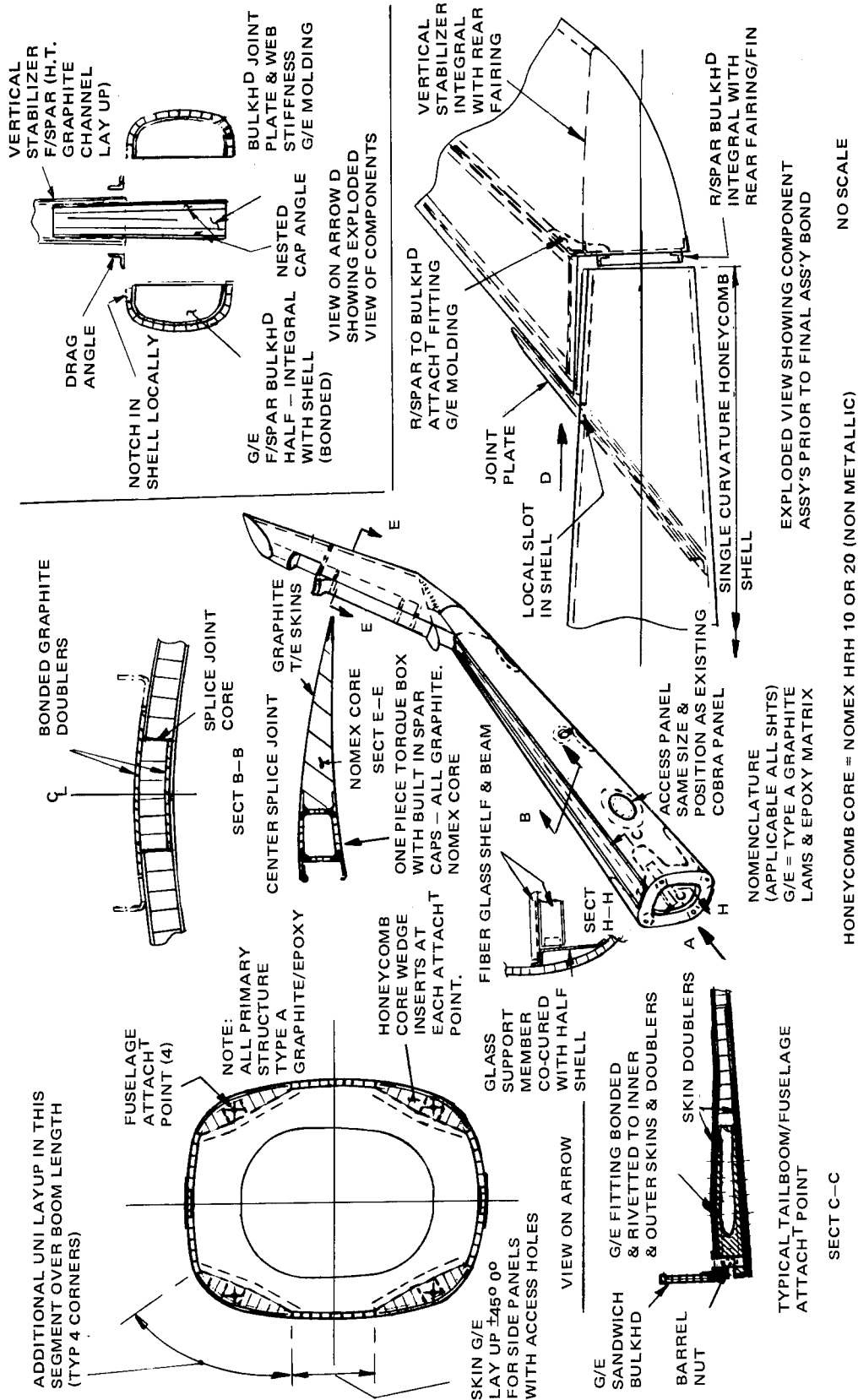
Figure 3. Monocoque Sandwich-Clamshell.
