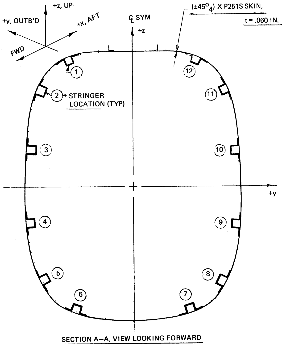
Figure 62. Concept 3 - Section Through Tail Boom.
