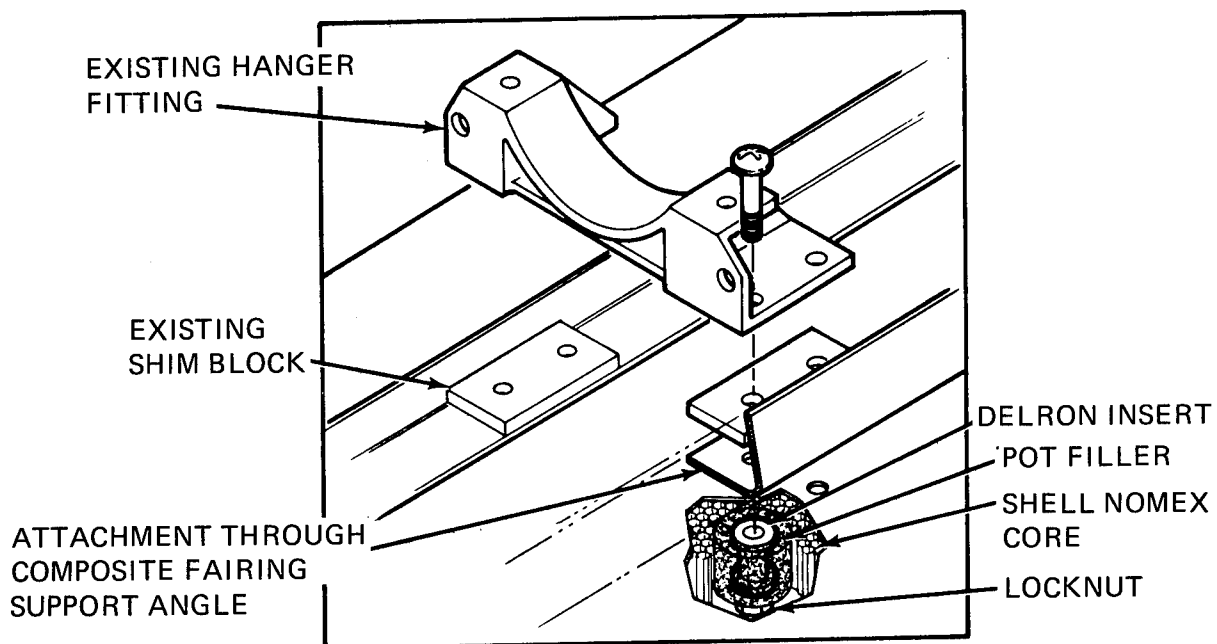
Figure 34. Drive Shaft Hanger Attachment.
