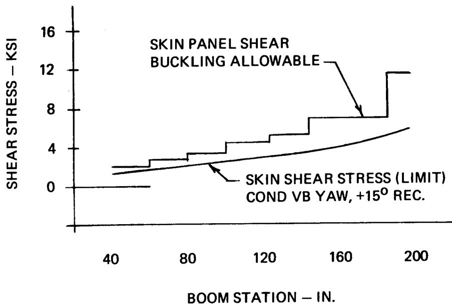
Figure 66. Shear Stress - Panel, Stringers ⑩ and ⑪ .
