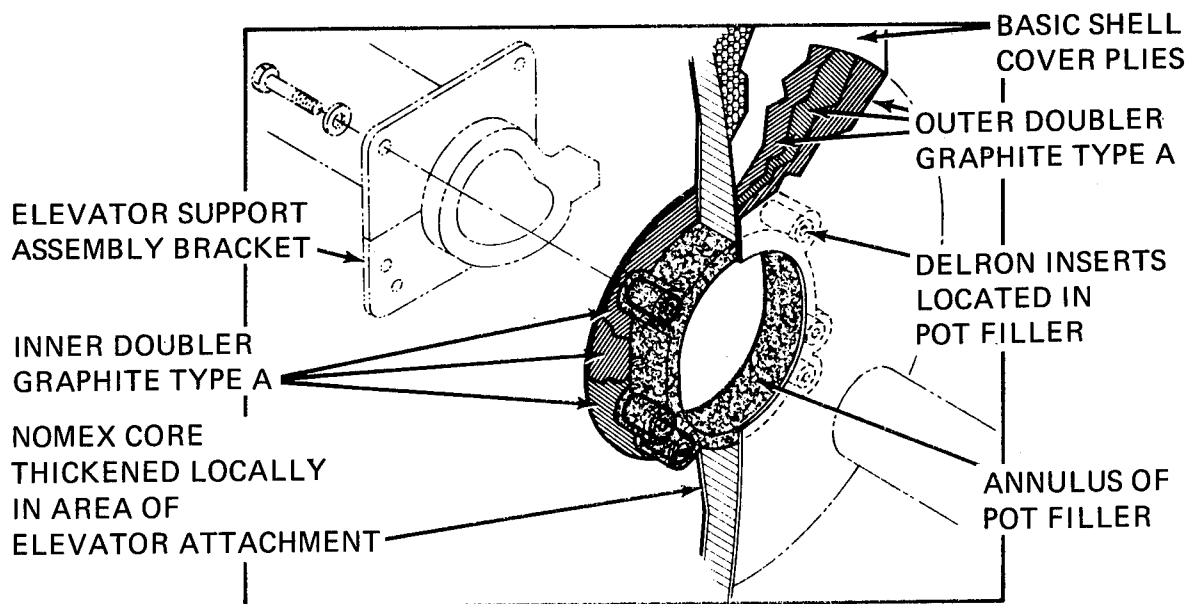
Figure 33. Elevator Support Structure.
