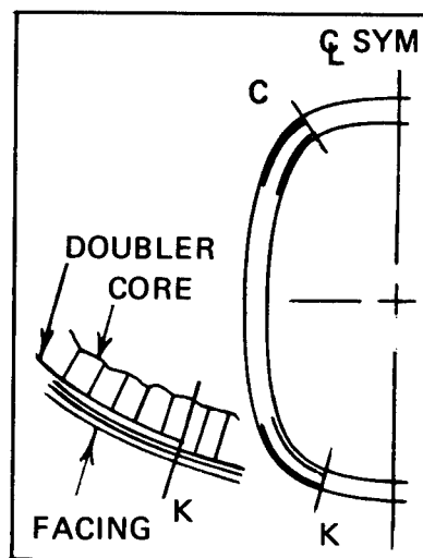
Figure 51. Doublers.
