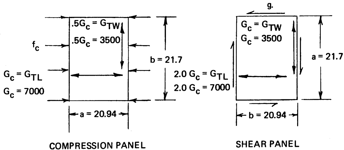
Figure 57. Side-Panel Geometry BS 80.44-101.38.
