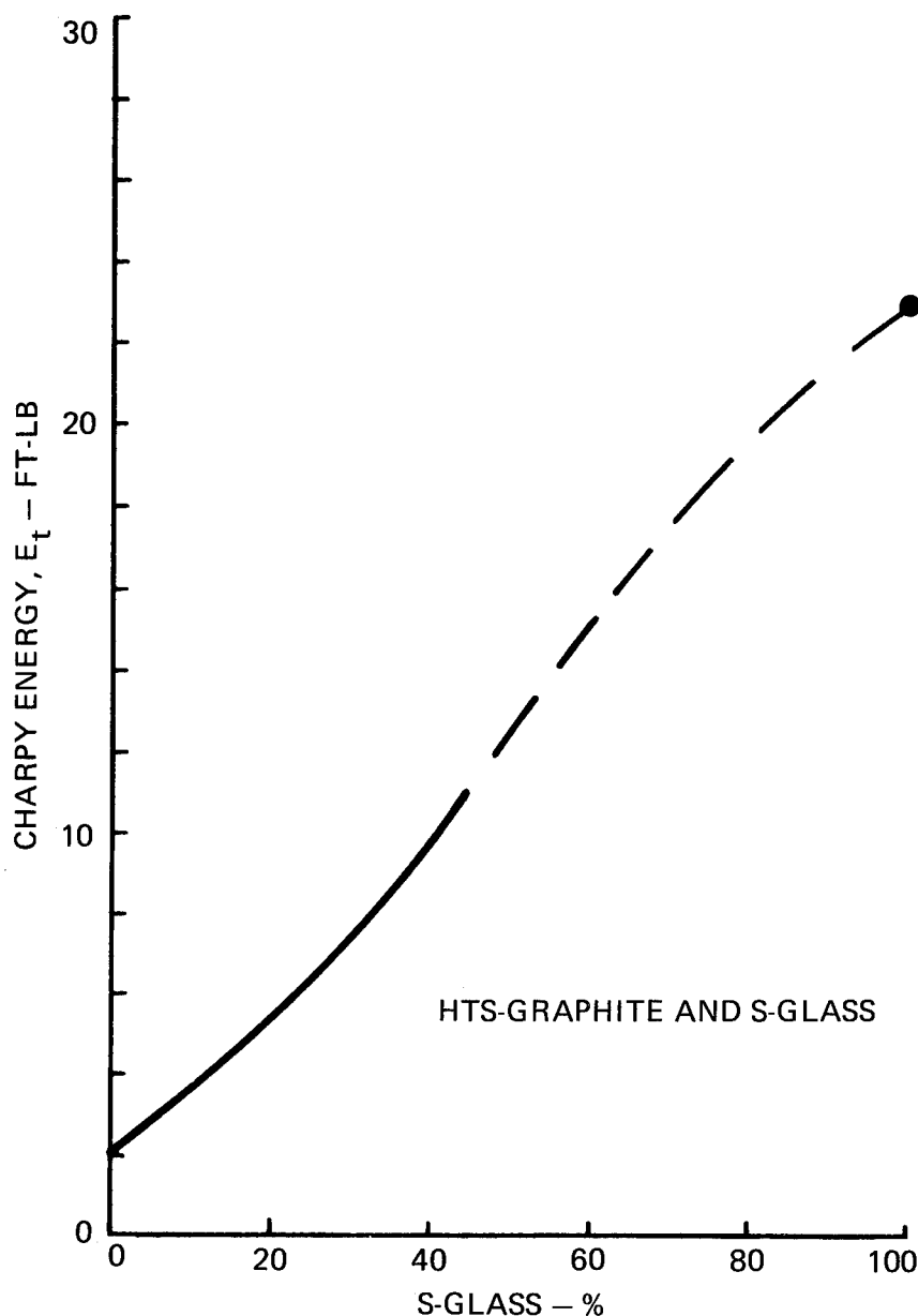
Figure 40. Charpy Impact Energy Relationship for a Hybrid Composite of Varied Proportions.
