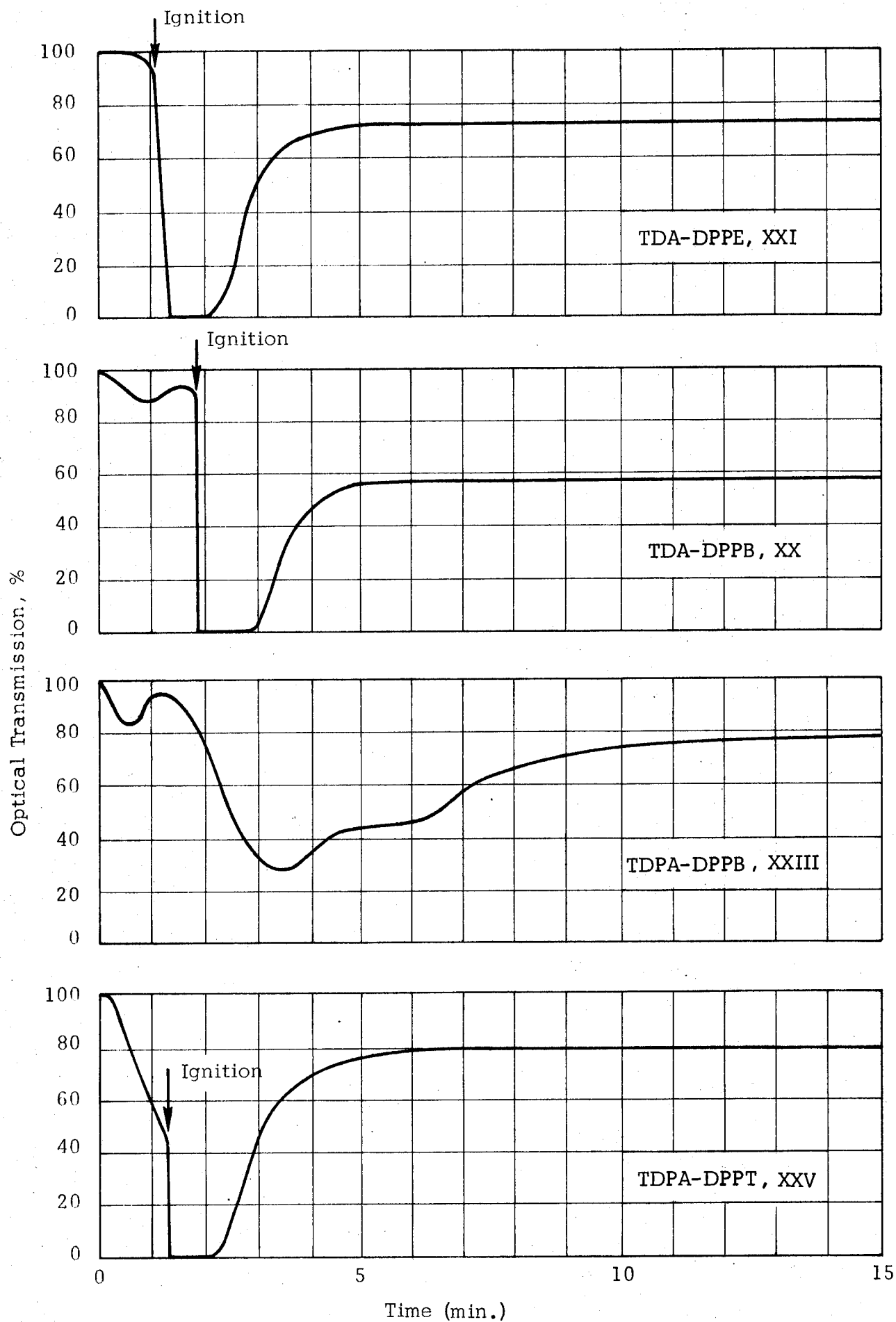
Fig. 45: Stagnation Burner Smoke Density Changes
