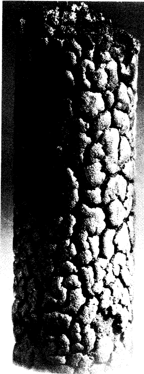
(g) Test 9; small-grain model tested in N 2 ; T_t = 3575^{\circ} \text{R} (1986 L-66-1121 K); t = 6.17 sec.
