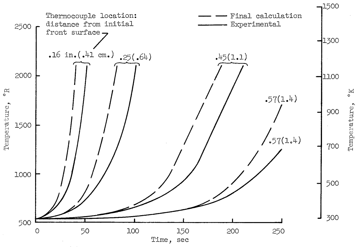
(b) Temperature histories.
