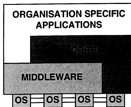
Figure 7. Application construction and maintenance services for interoperable ISs (OS = operating system, CORBA = Common Object Request Broker Architecture).
