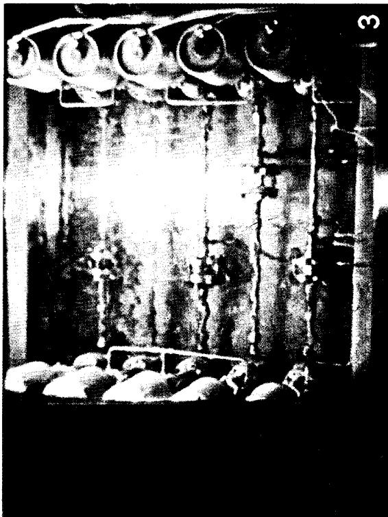
Figure 8. - Dynamic ELOX compatibility test for Lucite. Film speed, 24 frames per second; time interval between frames 3 and 4, 9 seconds.
