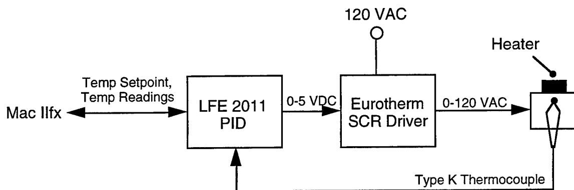
Figure 2.14 - Substrate Temperature Control Structure
