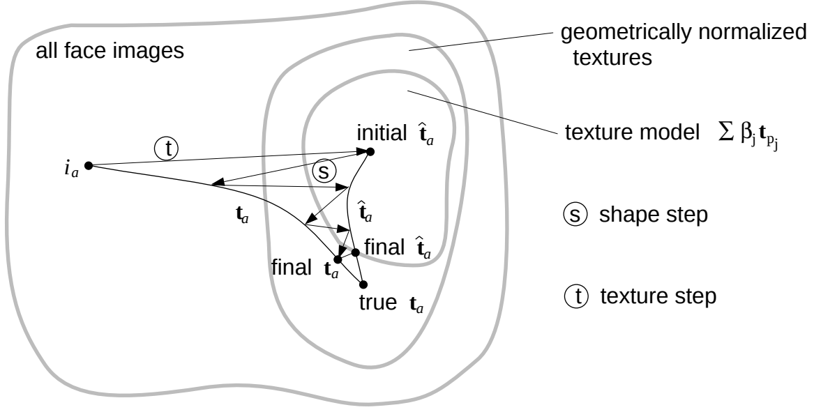
Figure 8: Convergence of the vectorization procedure with regards to texture. The texture and shape steps try to make \hat{\mathbf{t}}_a and \mathbf{t}_a converge to the true \mathbf{t}_a .
