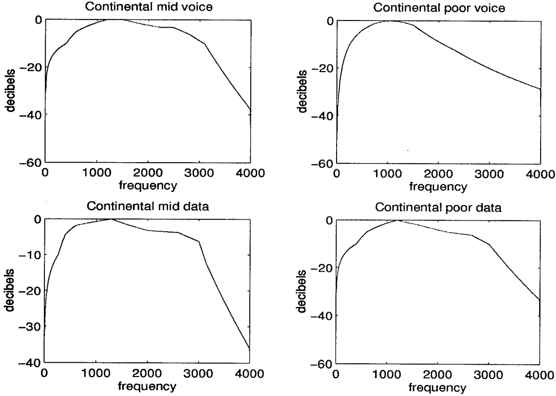
Figure 3.1: Various transmission channel characteristics.
