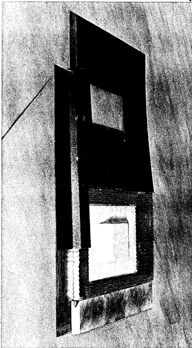
FIGURE 11. DETAILS-WING SKIN ASSEMBLY (ADVANCED CONCEPT)
