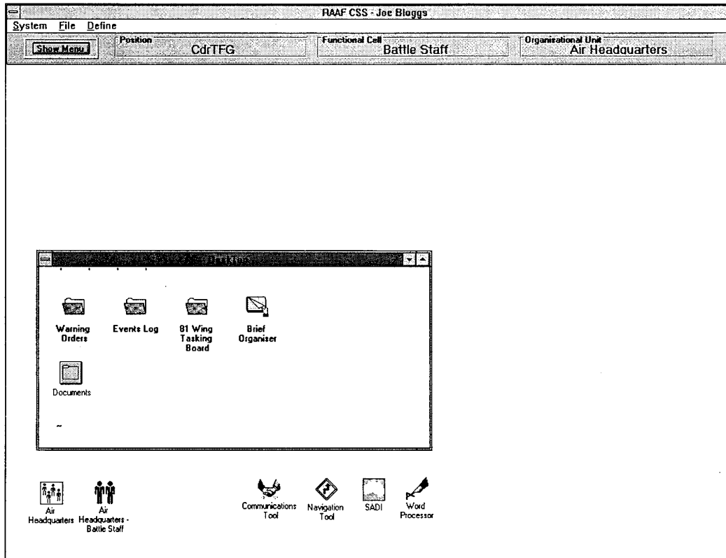
Figure 1. CDRTFG's Desktop.
