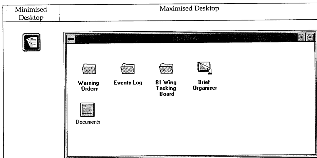
Figure 7. A desktop.
