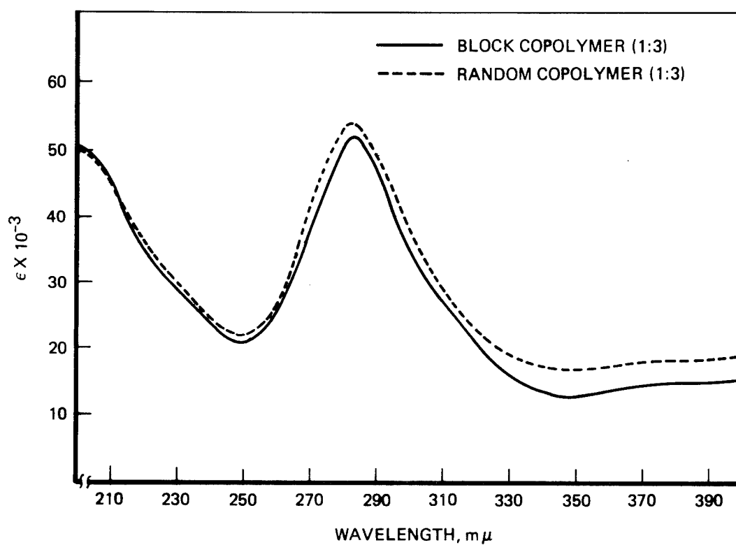
Figure 2: ULTRAVIOLET SPECTRA OF POLYPHENYLQUINOXALINES (IN \text{H}_2\text{SO}_4 )
