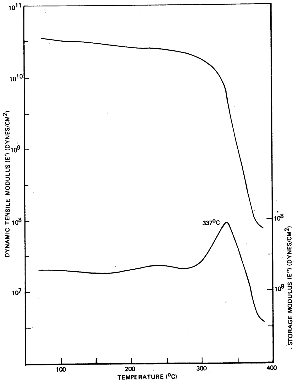
Figure 6: DYNAMIC MECHANICAL RELAXATION SPECTRUM OF PPQ 1
