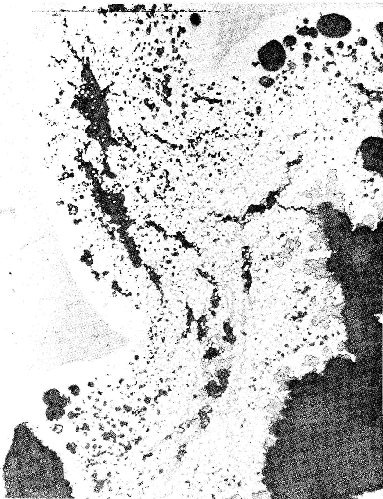
Figure A-7: CROSS SECTION OF DRIED GRAPHITE TOW IMPREGNATED WITH PPQI (POLYMER 3, TABLE 2) X80
