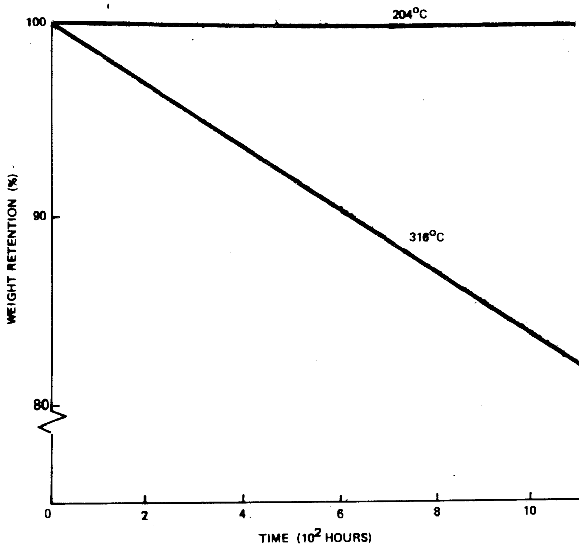
Figure 22 ISOTHERMAL AGING OF BiCo (1:3) LAMINATES AT 204°C (400°F) AND 316°C (600°F)
