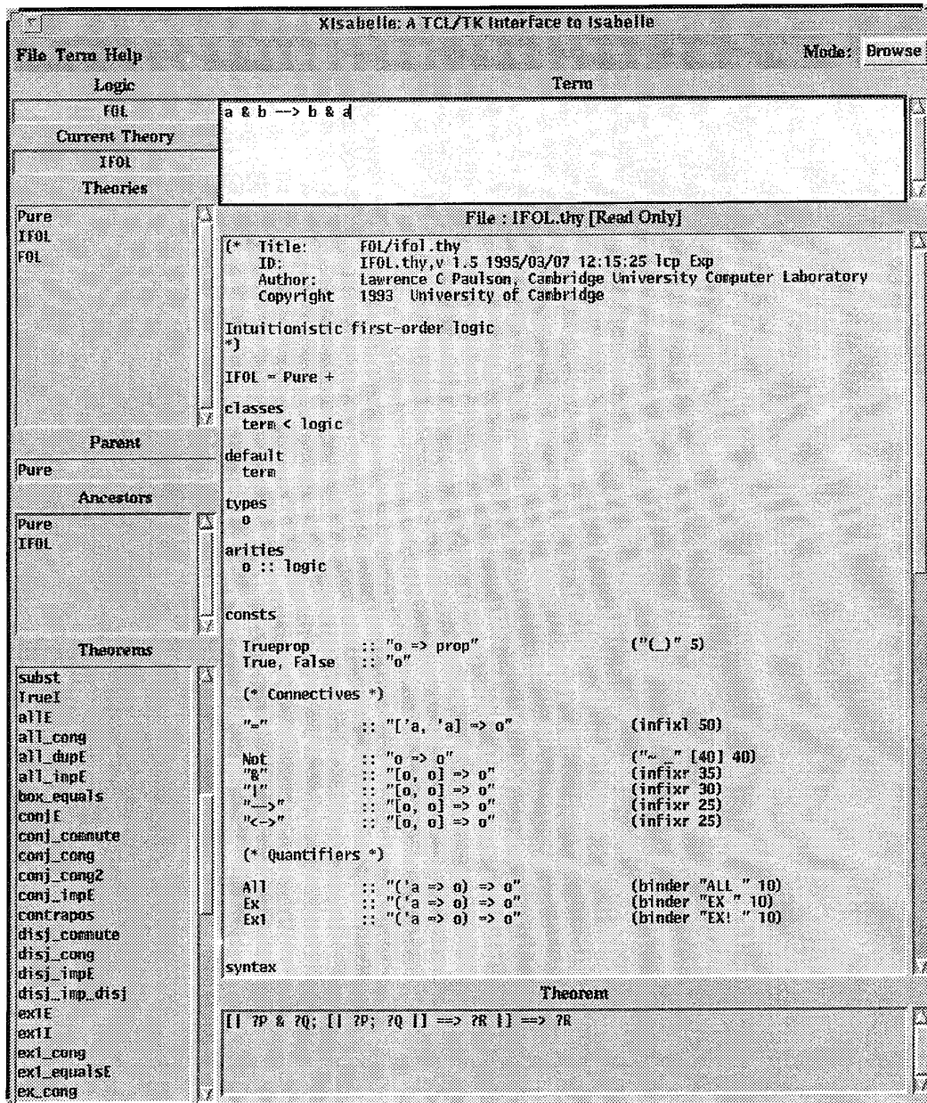
Figure 3: Browsing IFOL
