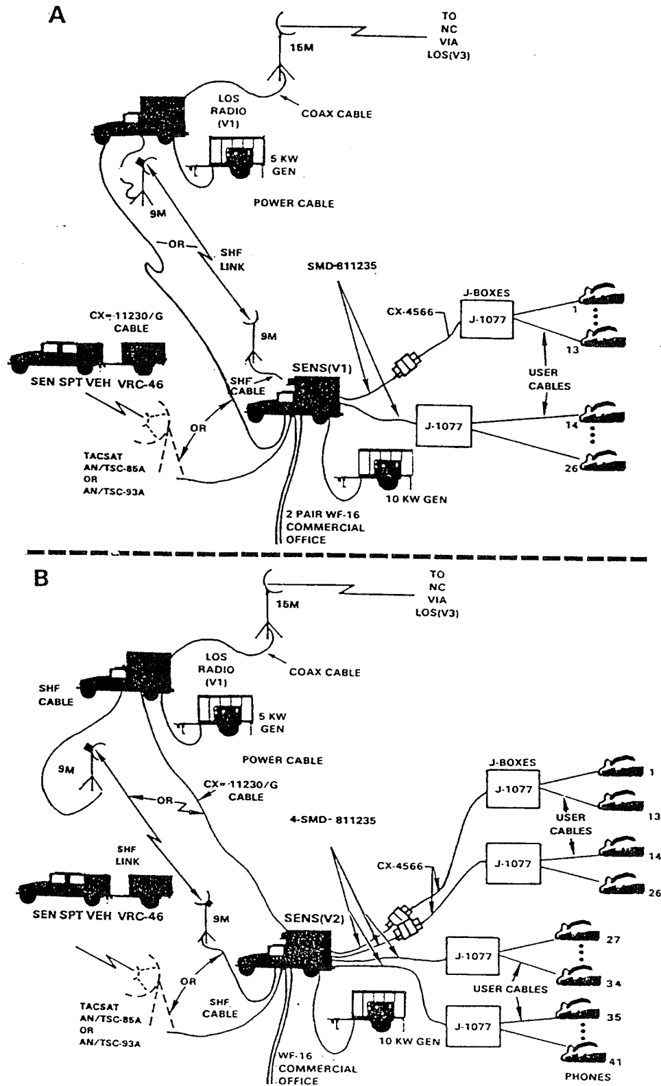
Figure 2. SENS deployment and connectivity.
