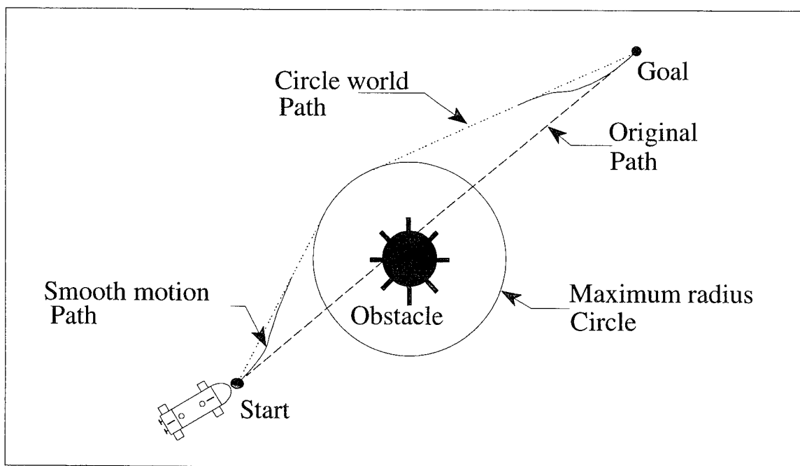
Figure 24. Smooth motion path planning of circle world.
