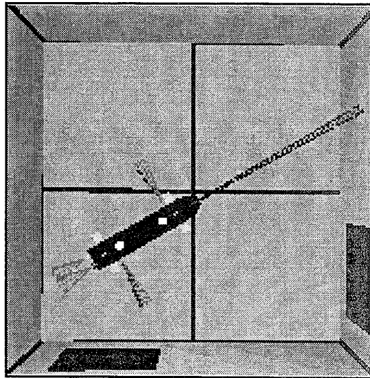
Figure 11. Sonar simulation of Phoenix in virtual CAUV test tank [Brutzman 94].
