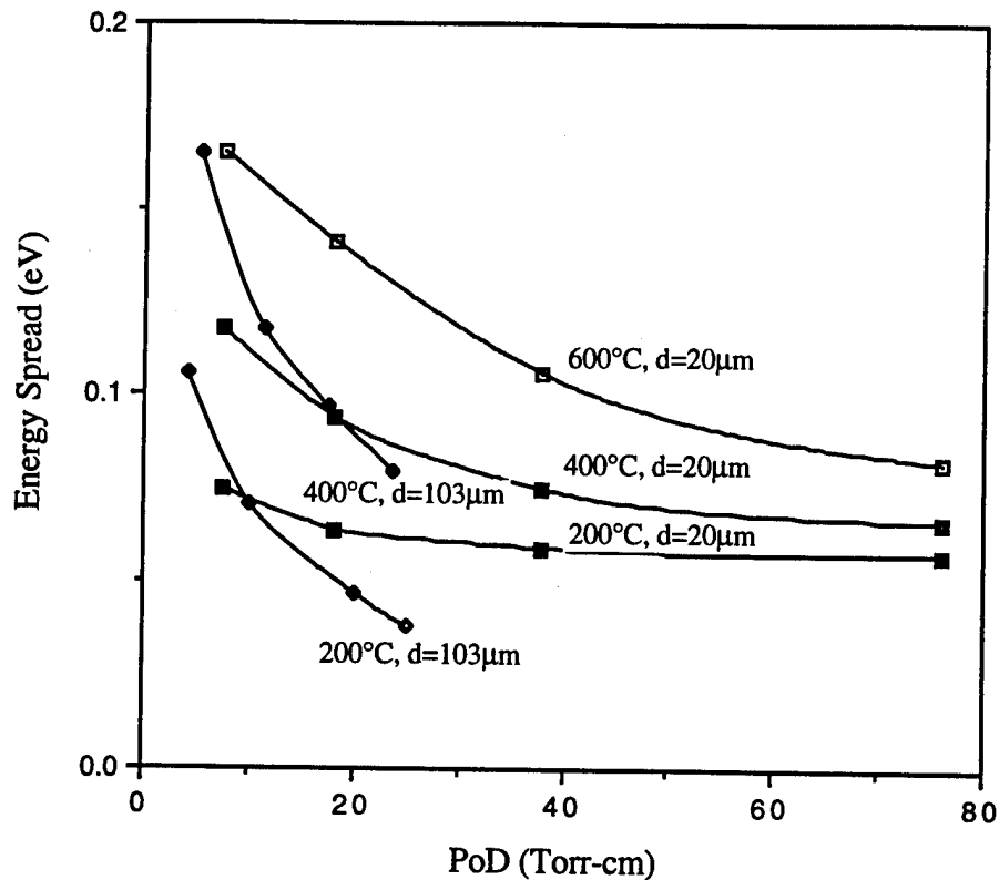
Figure 5. Energy spread as a function of the stagnation pressure-diameter product.
