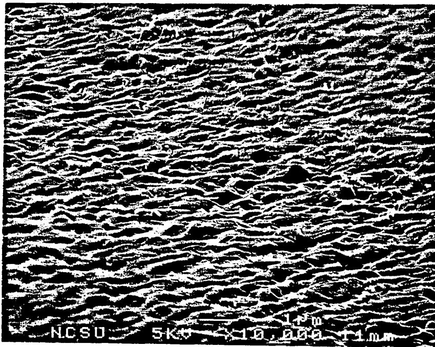
Figure 2. GaN film grown using He as the carrier gas.
