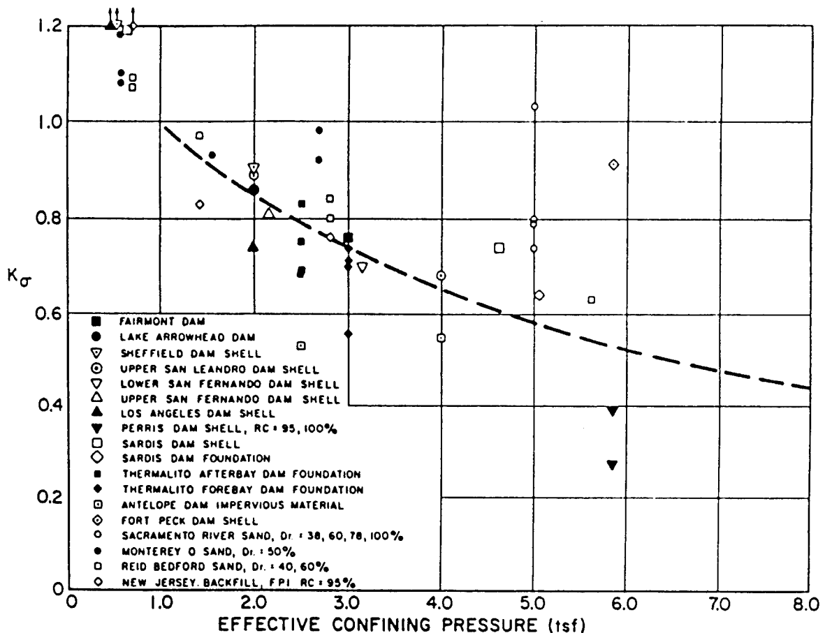
Figure 17. Adjustment to cyclic stress ratio to account for influence of vertical effective stress (Harder 1988)
