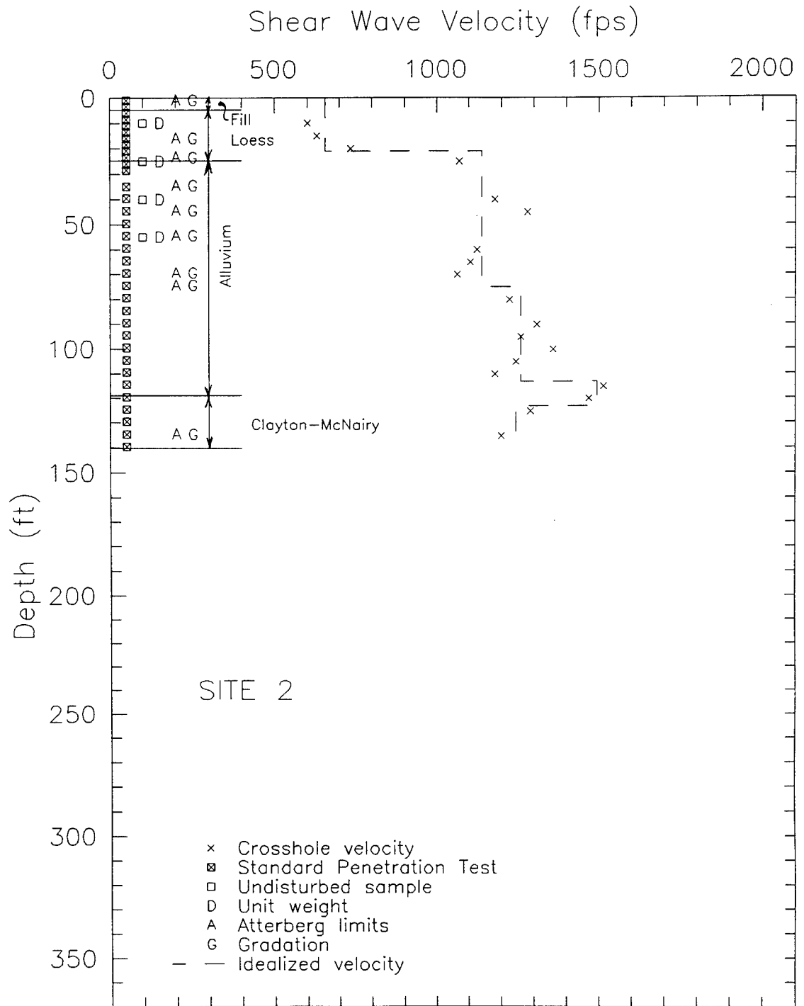
Figure 10. Depths of geotechnical testing and results of shear wave velocity measurements at Site 2
