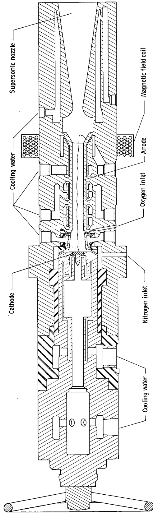
(b) Apparatus D arc-heater.
