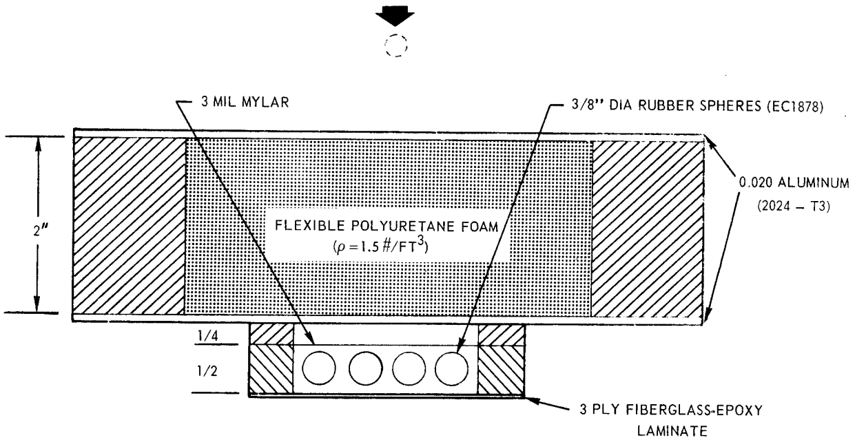
FIGURE 18 SELF-SEALING TILE — MECHANICAL SEALING CONCEPT (TYPE SST - B)
