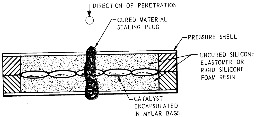
FIGURE 2 CHEMICAL SYSTEM SELF-SEALING CONCEPT
