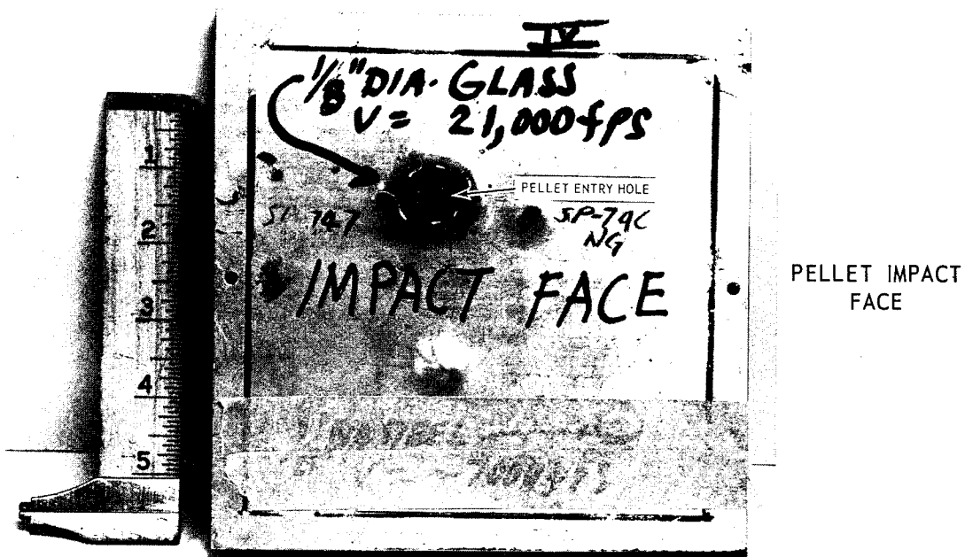
1/8" DIA. GLASS SPHERE V = 21,000 FPS
