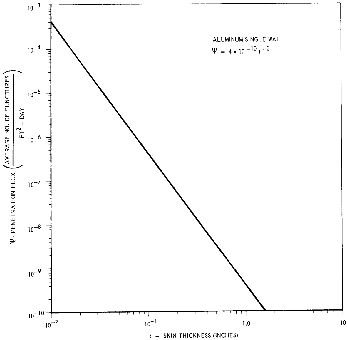
FIGURE 24 PENETRATION FLUX VS SKIN THICKNESS
