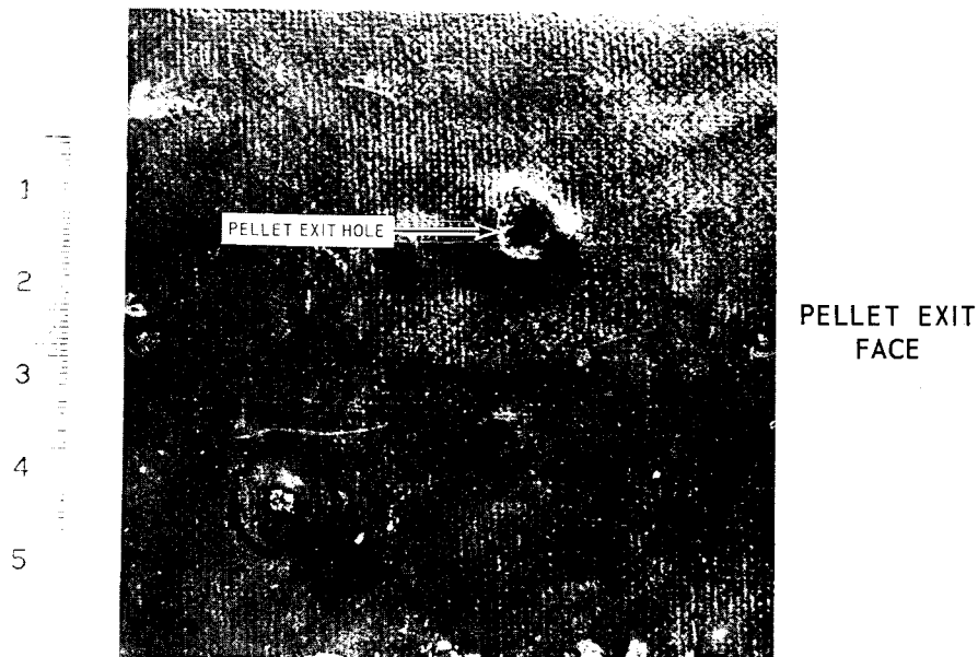
FIGURE B-1 RUPTURED HONEYCOMB CORE-ELASTOMER PANEL
