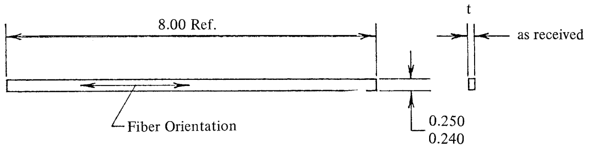
Figure B-1 Longitudinal Tensile Specimen Unidirectional Material
