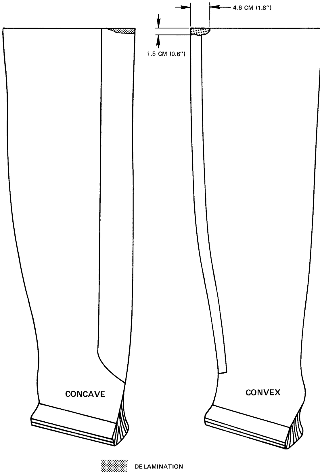
Figure 23 Visual Damage to Graphite/Epoxy Blade C-1 Following Impact with Ice Ball
