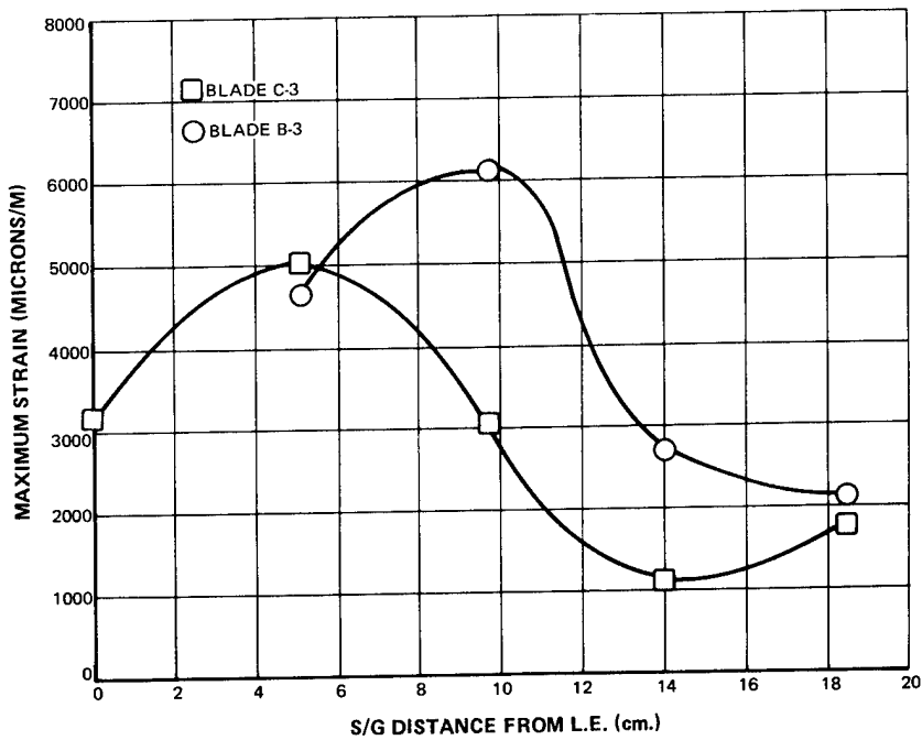
Figure 43 Maximum Strain at Impact Section K-K
