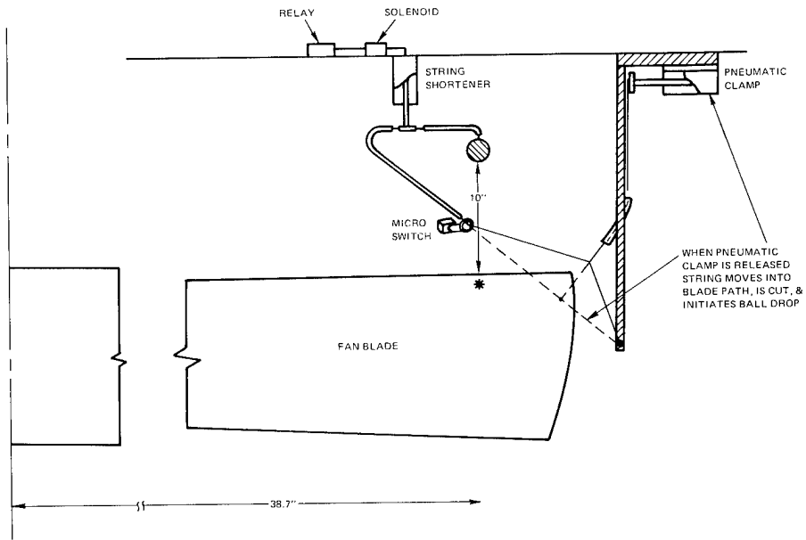
Figure 21 Schematic of Impact Object Drop Mechanism
