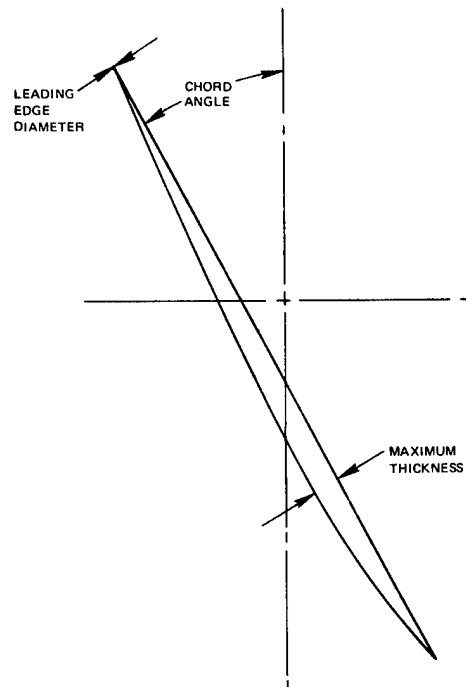
Figure 14 Composite Fan Blade - Airfoil Impact Section K-K 18.5 cm (7.3 in) from blade tip
