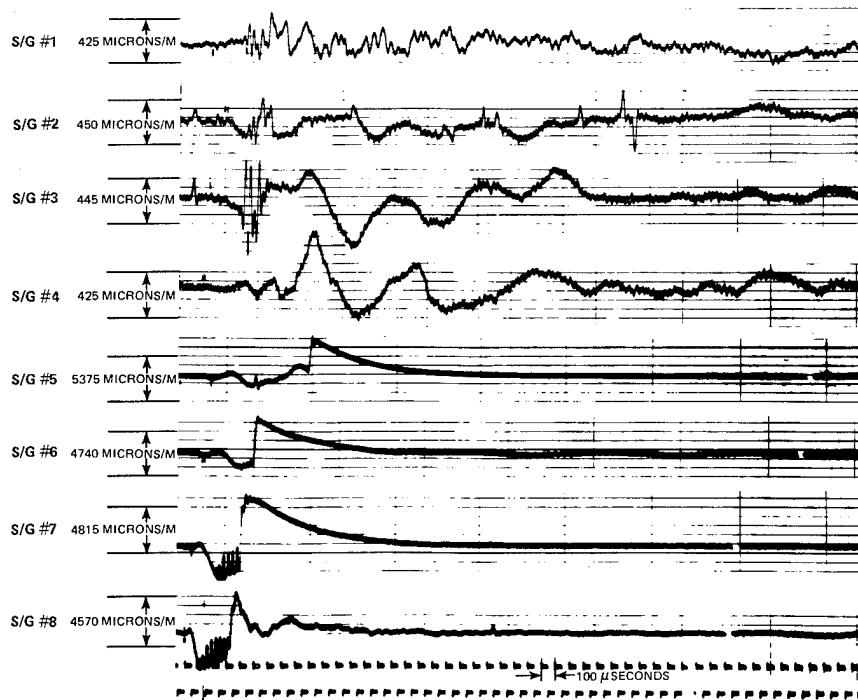
Figure 39 Strain Gage Oscillograph Record from Impact Test of Graphite/Epoxy Blade C-3
