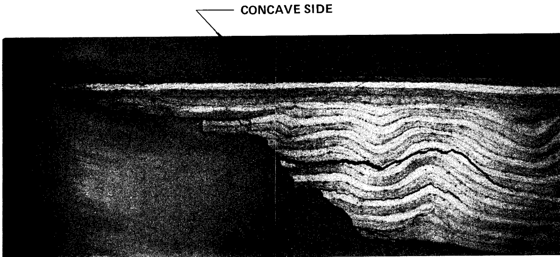
Figure 56 Photo-micrograph of Area 2, (Figure 54), Graphite/Epoxy Blade C-3 Showing Interlaminar Separations (13X)
