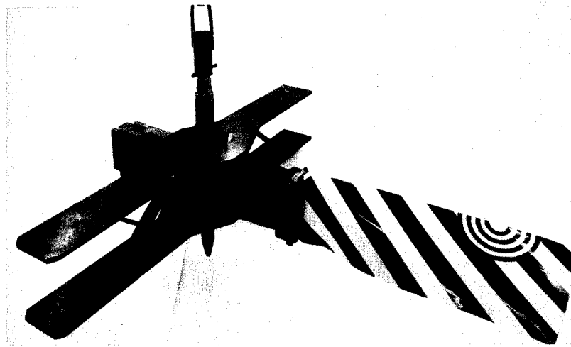
Figure 18 Composite Fan Blade in Spin Test Rig
