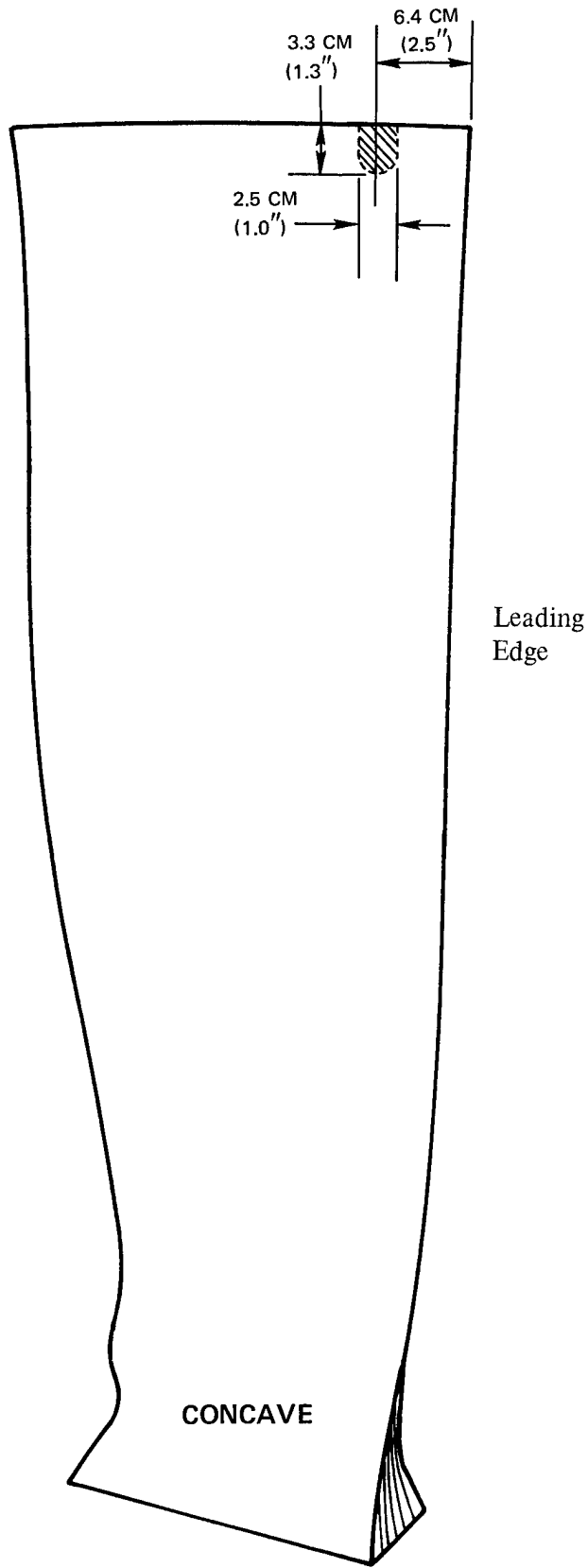
Figure 11 Ultrasonic Indications on Graphite/Epoxy Blade C-5 Before Impact.
