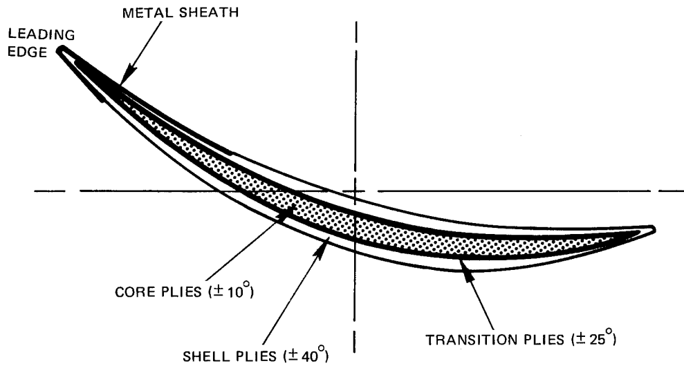
Figure 2 Composite Fan Blade - Typical Airfoil Section
