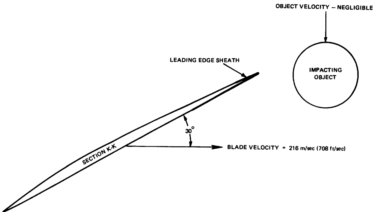
Figure 15 Composite Fan Blade - Impact Testing Condition
