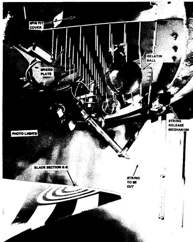
Figure 22 Drop Mechanism For Impact Testing
