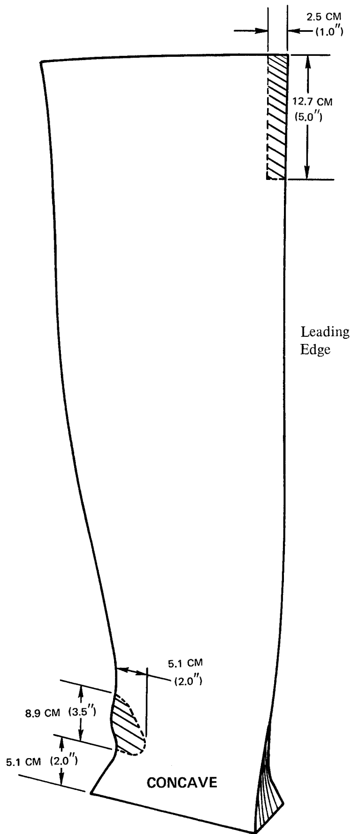
Figure 9 Ultrasonic Indications on Graphite/Epoxy Blade C-1 Before Impact.
