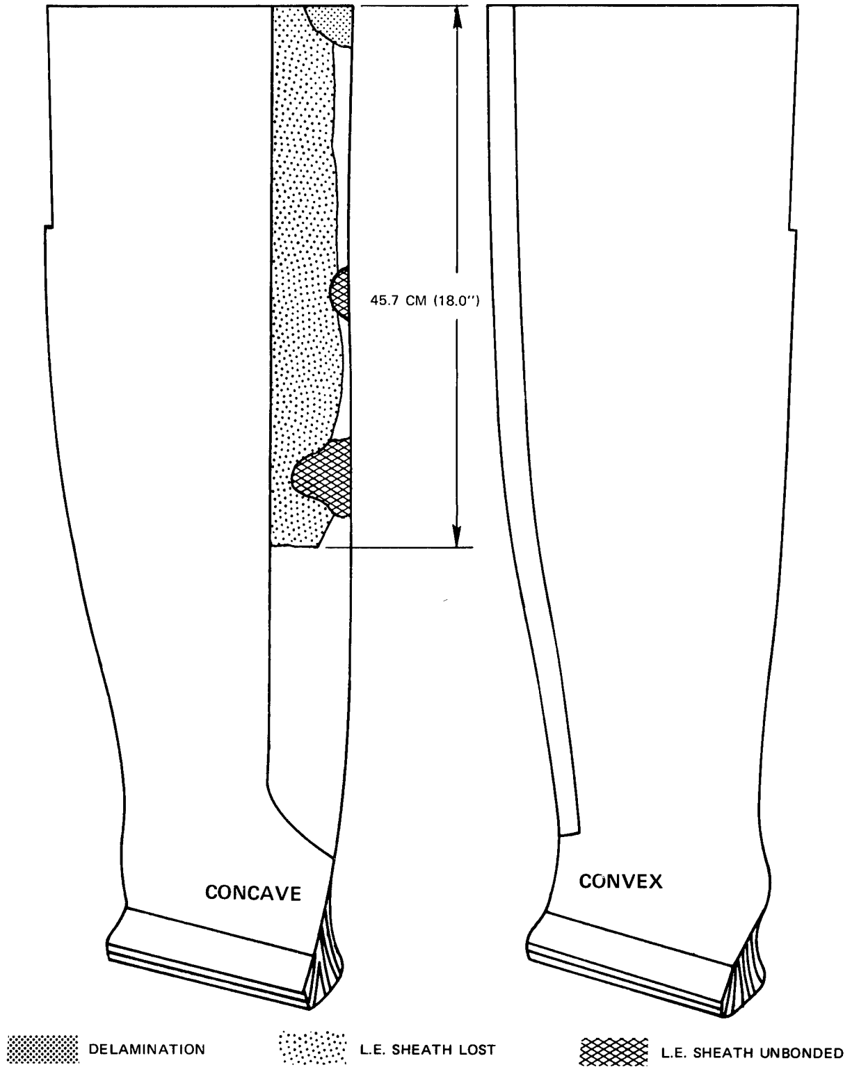
Figure 44 Visual Damage to Graphite/Epoxy Blade C-4 Following Impact with Gravel
