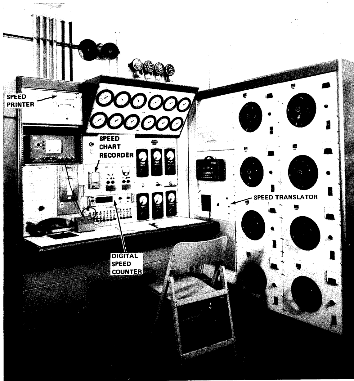
Figure 20 Spin Pit Test Stand Control Panel
