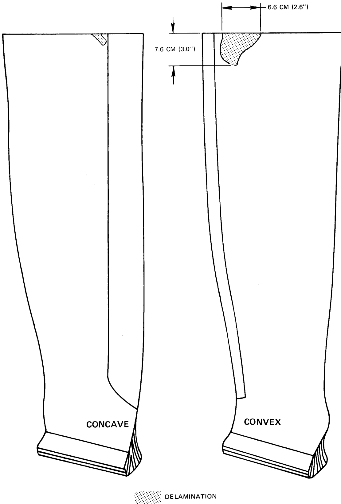
Figure 52 Visual Damage to Graphite/Epoxy Blade C-5 Following Impact with Starling
