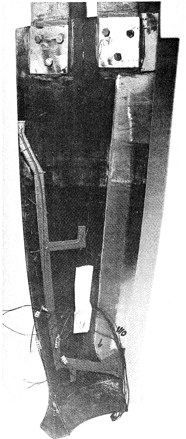
Figure 39. NG5 Graphite/Epoxy Blade after Impact (Concave Surface), Test No. STOL 1.
