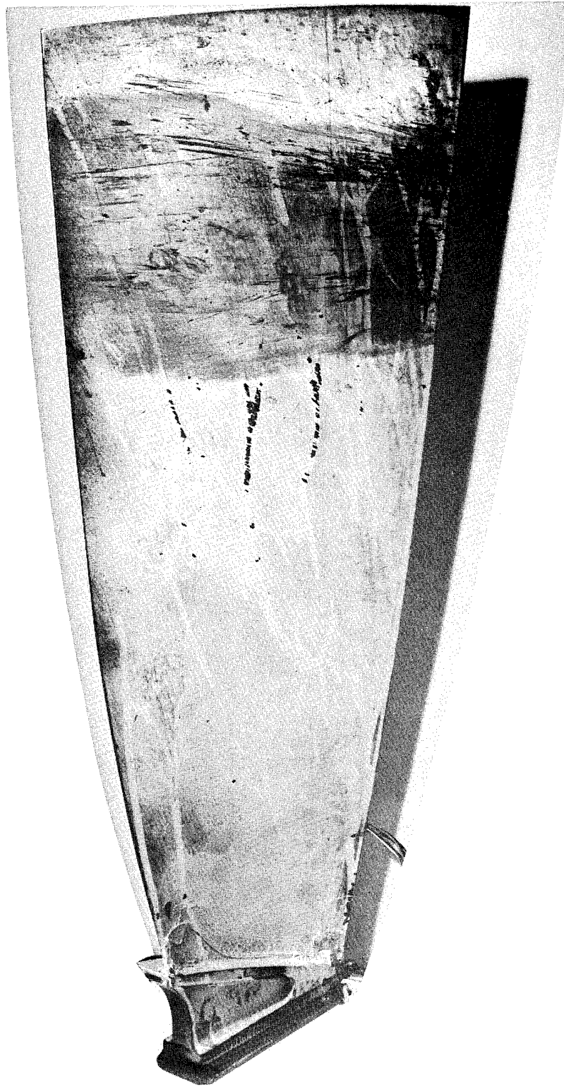
Figure 43. Titanium Blade after Impact (Concave Surface), Test No. STOL 3.
