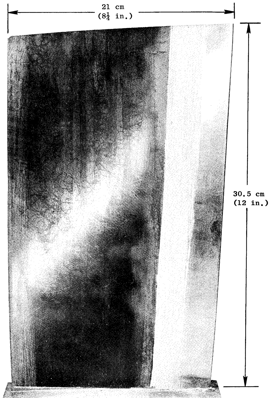
Figure 45. Typical NASA-FOD Hybrid Test Panel Before Impact.
