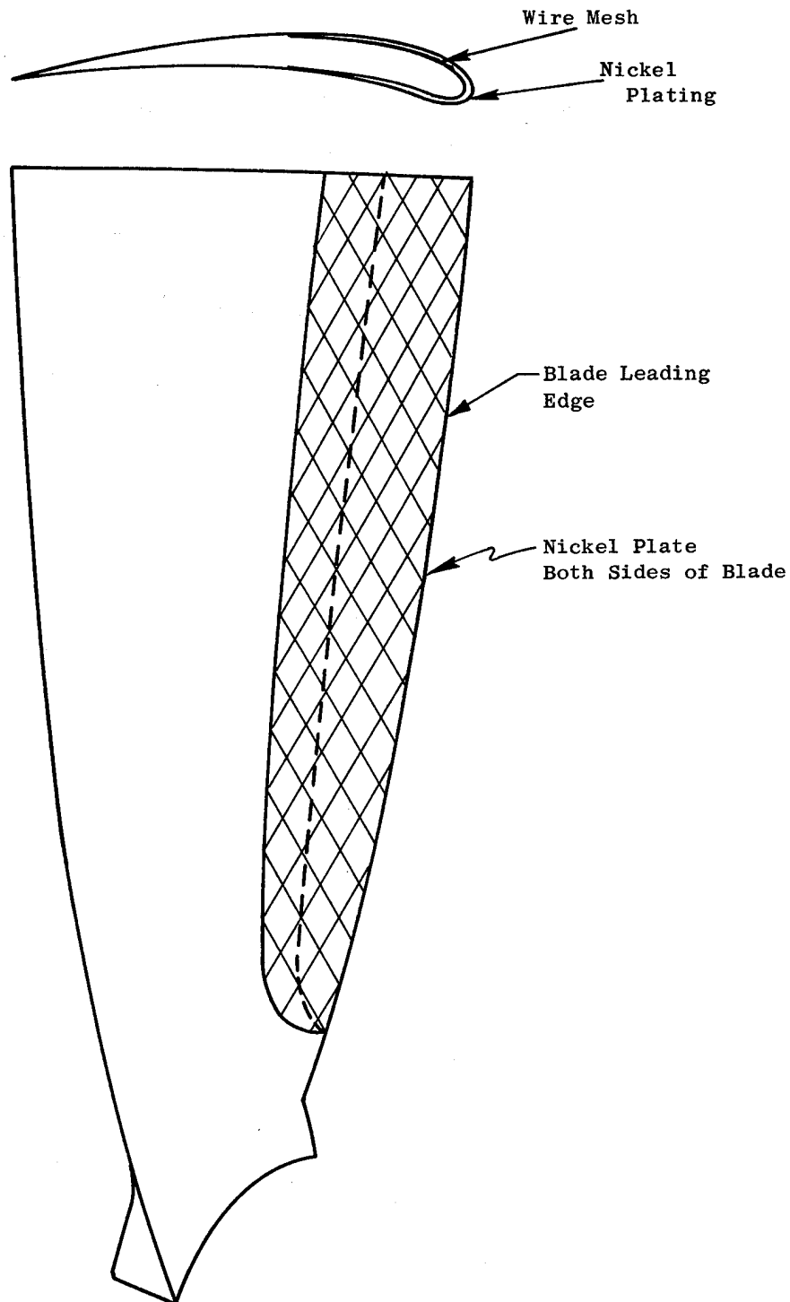
Figure 4. Nickel-Plated Areas on TF39 Polymeric Composite Blades.
