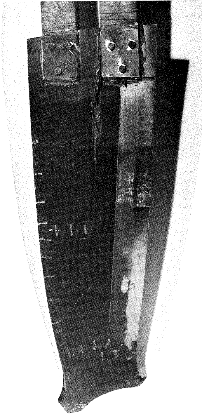
Figure 41. NB5 Boron/Epoxy Blade after Impact (Concave Surface), Test No. STOL 2.
