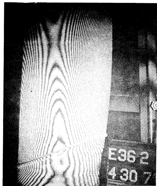
Figure 11. Holographic NDT of Graphite/Epoxy Blade. Upper and Lower Portions of Each Side are Inspected Separately. Leading Edge Disbonds are Prevalent. Note Trailing Edge Discrepancy.
