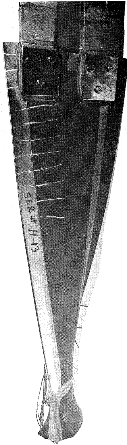
Figure 38. NG5 Graphite/Epoxy Blade after Impact (Convex Surface), Test No. STOL 1.
