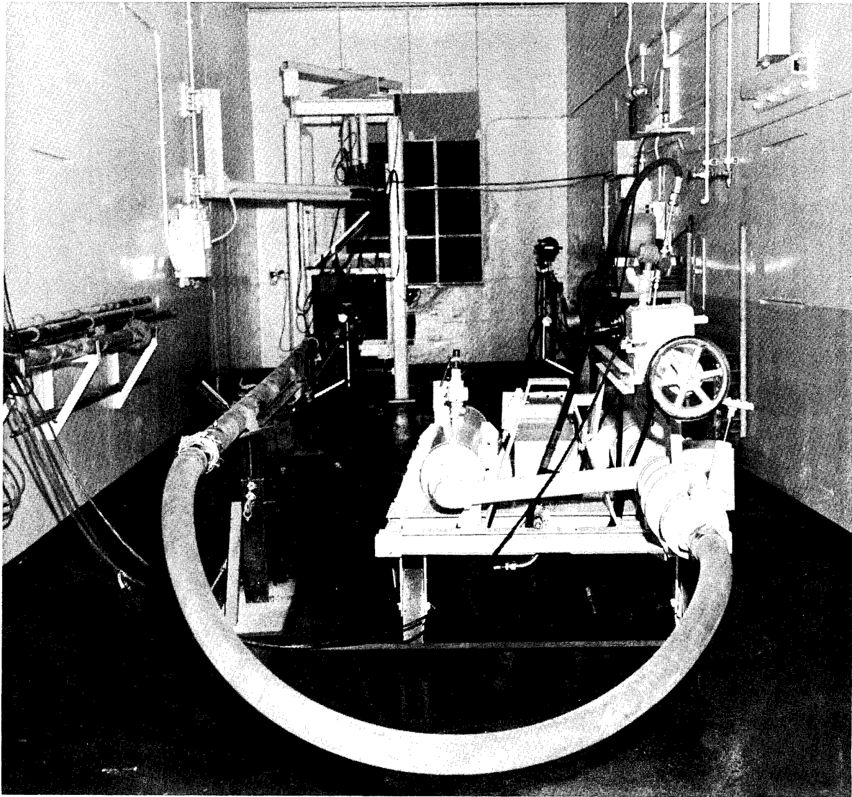
Figure 15. Static Test Facility Ballistic Gun and Gas Pressurization Dolly.
