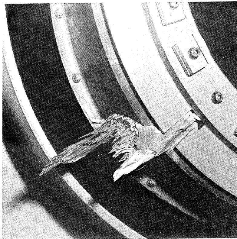
NASA-FOD Impact Resistance Test Blade S/N NB4 Boron/Epoxy Tip Speed: 244 m/sec (800 ft/sec) 794 g (28 oz) RTV Bird 340 g (12 oz) Slice 0.384 Radians (22°) Incidence Angle
