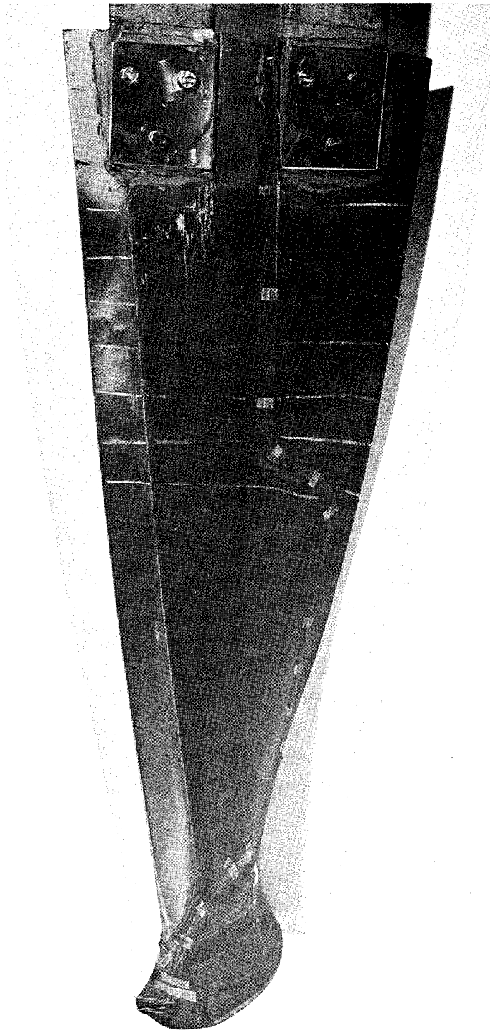
Figure 40. NB5 Boron/Epoxy Blade after Impact (Convex Surface), Test No. STOL 2.
