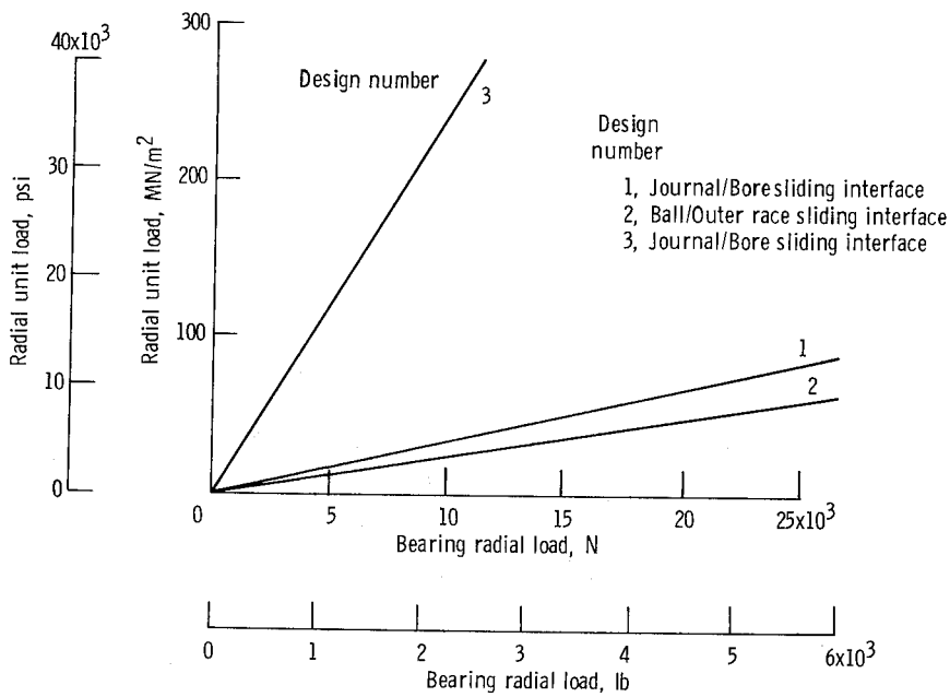
Figure 2. - Unit loads at sliding surface as a function of total radial load for three bearing designs used in this study.
