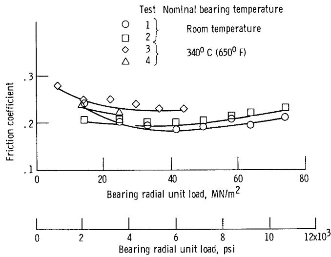
Figure 5. - Friction for journal/bore sliding contact (polyimide composite ball) design 1. Oscillation frequency at \pm 15^\circ amplitude, 1 hertz.
