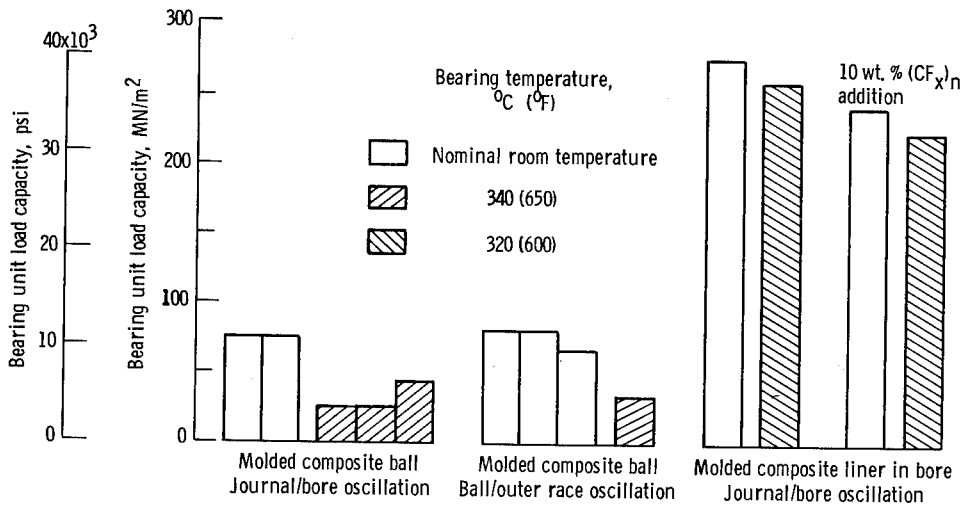
Figure 9. - Unit load capacities of three bearing designs with graphite-fiber - polyimide composite self-lubricating elements. Capacities determined during oscillation frequencies of 1 hertz at ±15° amplitude.
