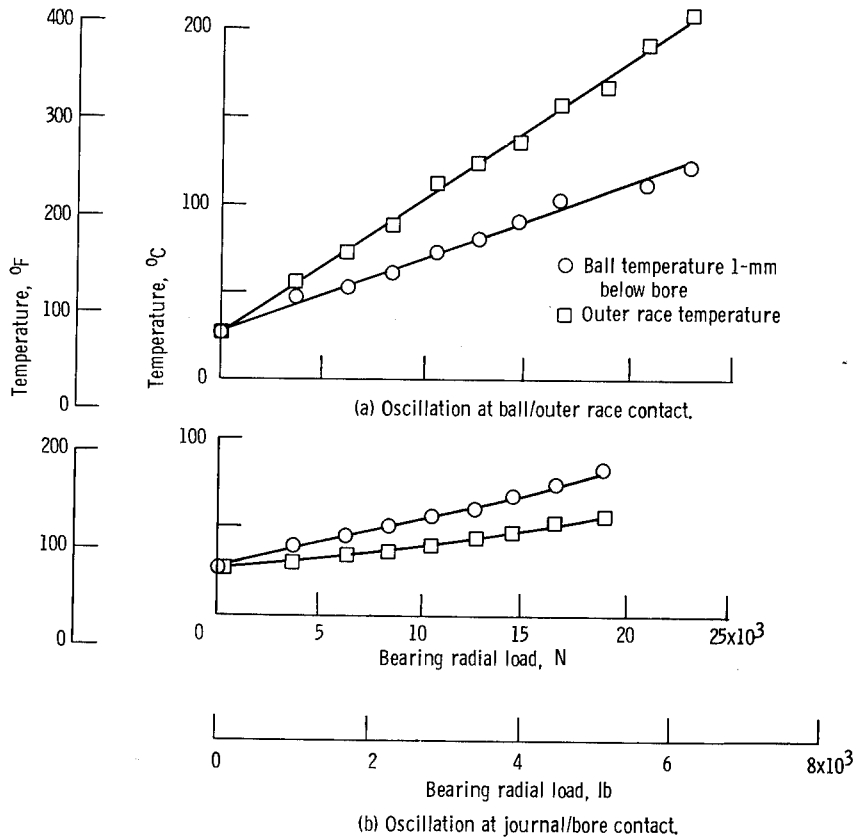
Figure 7. - Friction-induced bearing temperatures for two methods of bearing mounting. Nominal room temperature tests; oscillation frequency at \pm 15^\circ amplitude, 1 hertz.
