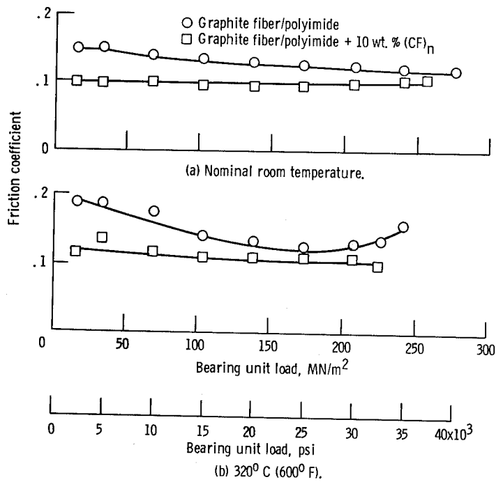
Figure 8. - Influence of (CF) n addition on friction of bearings with thin-wall polyimide composite liner in cylindrical bore. Oscillation frequency at ±15° amplitude, 1 hertz.
