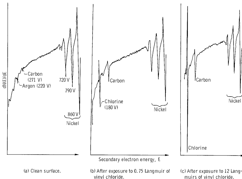
Figure 3. - Auger spectra of nickel surface; clean surface, after exposure to 0.75 Langmuir of vinyl chloride, and after exposure to 12 Langmuirs of vinyl chloride. Beam current, 10 microamperes.
