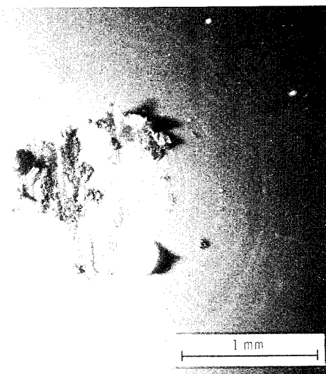
Figure 10. - Photomicrograph of wear scar of poly(vinyl chloride) rider after sliding on iron disk.
