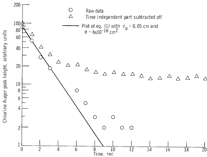
Figure 6. - Time dependence of chlorine peak from poly(vinyl chloride) absorbed from solution of tetrahydrofuran onto a steel disk. Beam current, 1 microampere.
