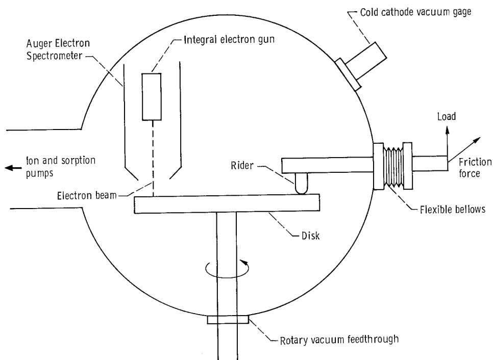
Figure 1. - Experimental apparatus with Auger Electron Spectrometer.
