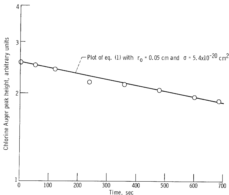
Figure 8. - Time dependence of chlorine Auger peak from nickel disk after sliding poly(vinyl chloride) 15 revolutions at 500-gram load. Beam current, 10.6 microamperes.
