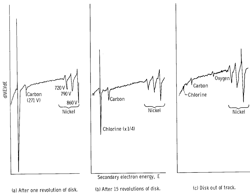
Figure 7. - Auger spectra of nickel disk after sliding poly(vinyl chloride) at 500-gram load after one revolution of disk, after 15 revolutions of disk, and where disk is out of track.
