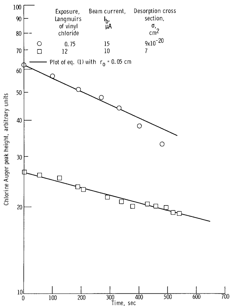
Figure 4. - Time dependence of chlorine Auger peak from nickel disk exposed to 0.75 and 12 Langmuirs of vinyl chloride.
