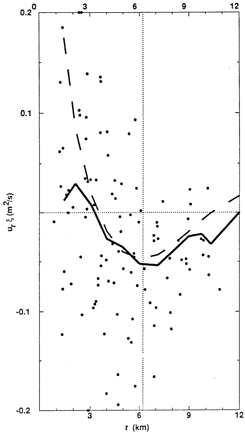
Figure 19: Radial structure of the real (co-spectral) part of the radial displacement flux u_r \xi' in the \lambda_z = 100\text{-}300 m band. Dots and triangles correspond to values from individual XCPs and HRPs, respectively. Solid curves are radial bin averages. The dashed curve depicts a vortex-trapped wave model prediction.
