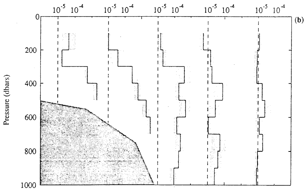
Figure 23: Average kinetic energy dissipation rates \epsilon (a) and diapycnal eddy diffusivities K_\rho (b) as a function of depth and radial distance from the seamount. The 0.5-m \epsilon estimates are averaged into 100-m thick vertical bins and lateral bins grouped (i) above the summit plain, (ii) at the summit rim, (iii) about the 1500-m isobath, (iv) about the 2500-m isobath, and (v) more than 10 km from the seamount. Lateral spacing of the average profiles is not to scale and the topography is schematic. The bracketing 95% uncertainties were computed with a bootstrap technique (Efron and Gong 1983; Polzin 1992) and do not differ substantially from those computed assuming a log-normal distribution (Baker and Gibson 1987). Eddy diffusivities (b) were inferred from the kinetic energy dissipation rates following Osborn (1980) using a mixing efficiency of 0.25 (Oskey 1982). Error bounds in (b) are 95% confidence limits from (a).
