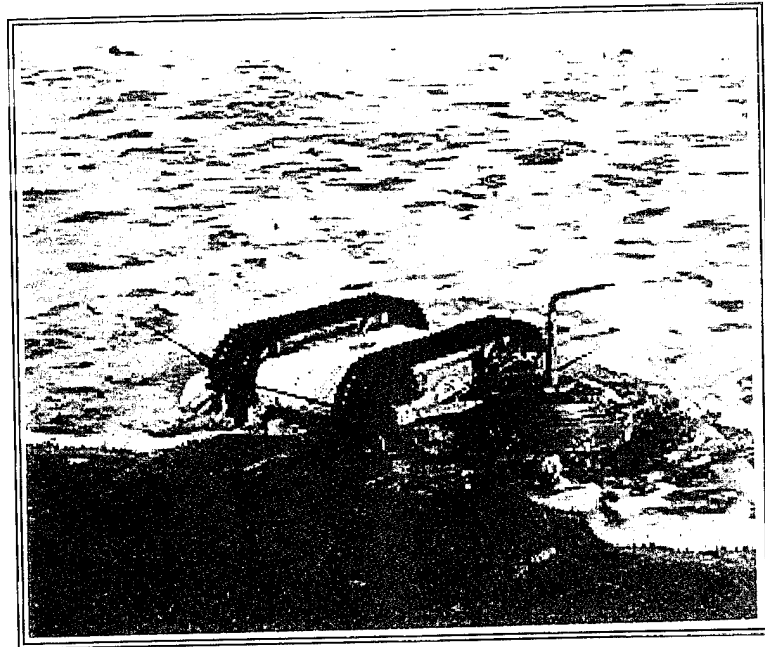
Figure 1. A Lemming Vehicle Detecting a Tilt-Rod Mine. Photo courtesy of Foster-Miller, Inc.
