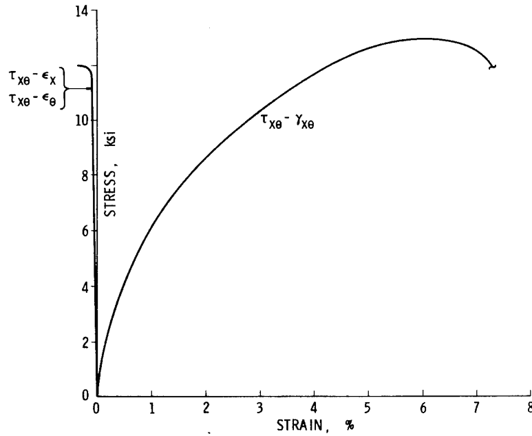
FIGURE III.34. STRESS-STRAIN CURVE, CT-43
