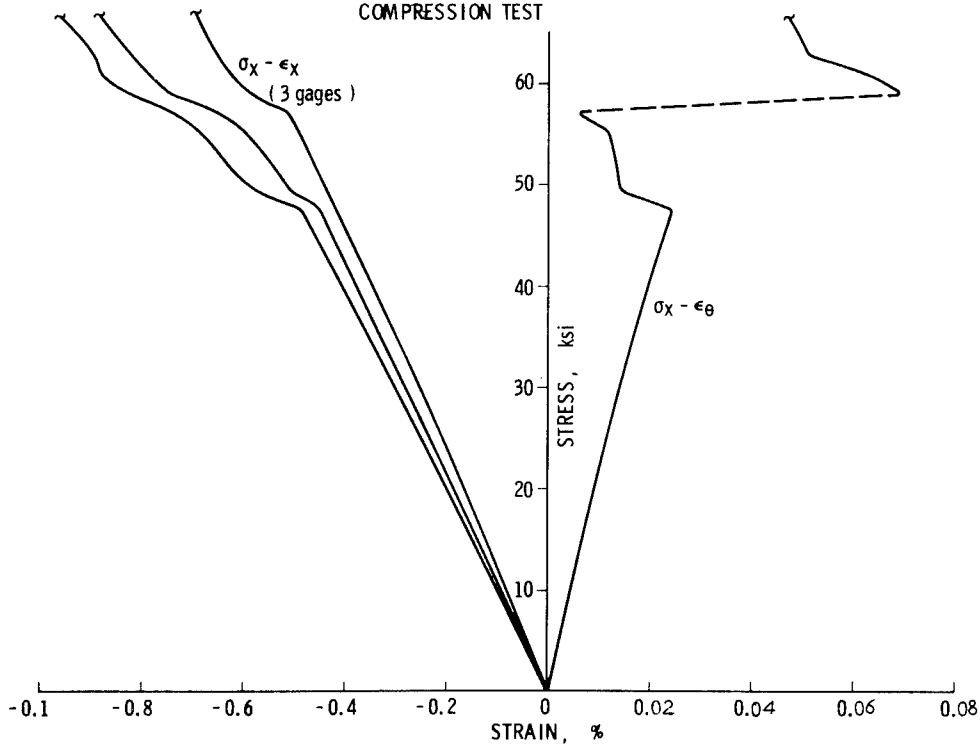
FIGURE III.35. STRESS-STRAIN CURVE, CT-44
