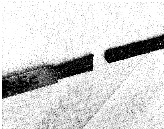
FIGURE II.18. UNIAXIAL COM- PRESSION SPECIMEN 5-5C AFTER FAILURE, [0] 12T
