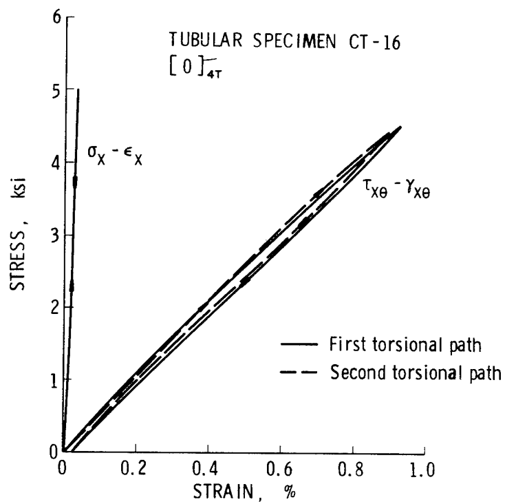
FIGURE III.27. STRESS-STRAIN CURVE, CT-16
