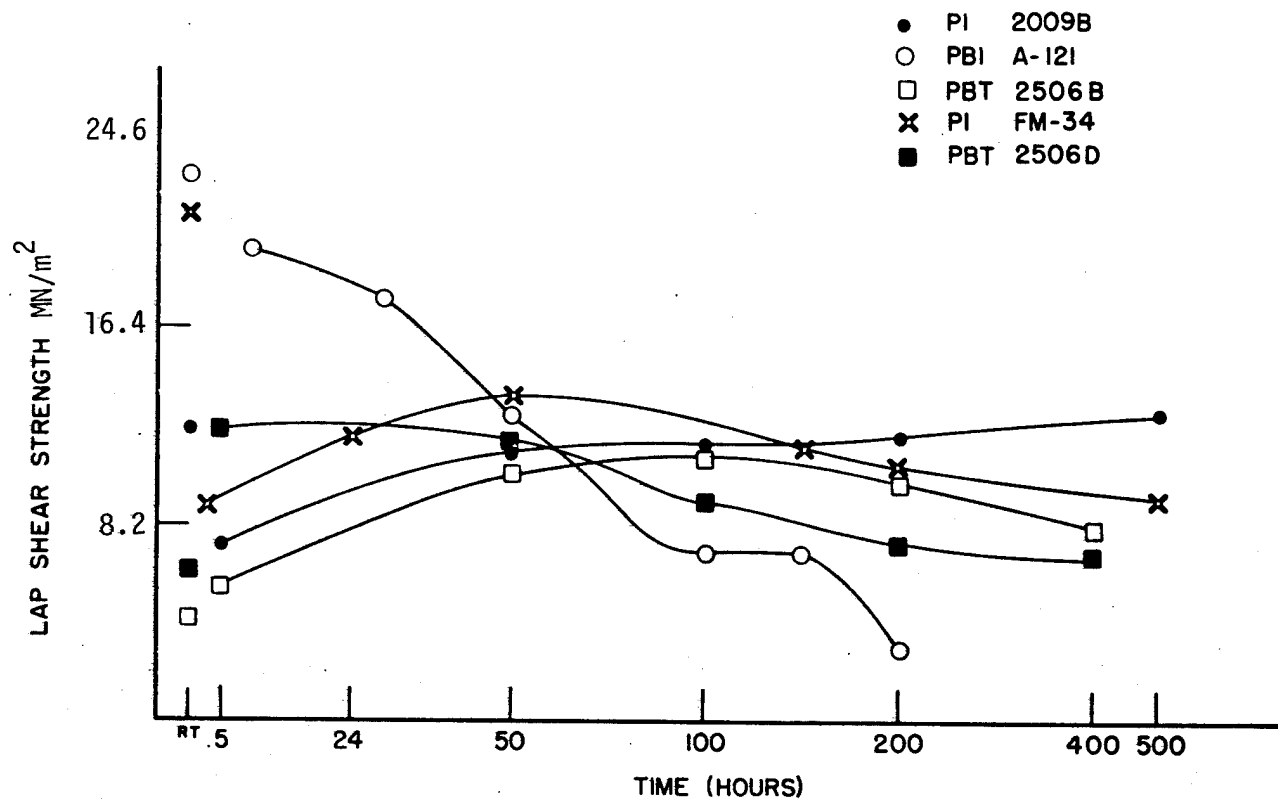
Figure 4. 589°K Lap-shear Strengths of Titanium Joints Bonded With Various High Temperature Adhesives
