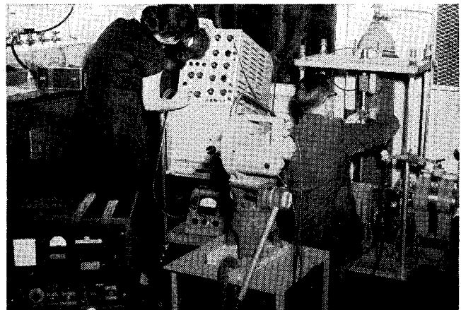
Figure 1. High-rate tensile apparatus showing Fastex camera set-up.
