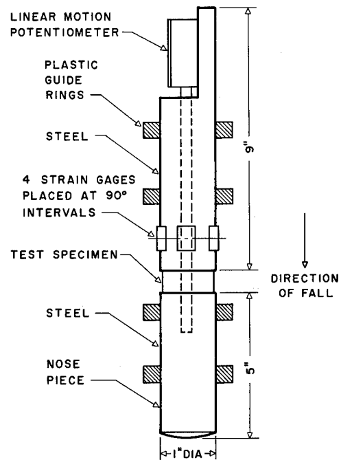
Fig. 4 Impact test vehicle
