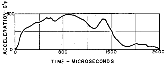
Fig. 7 Typical impact test data
