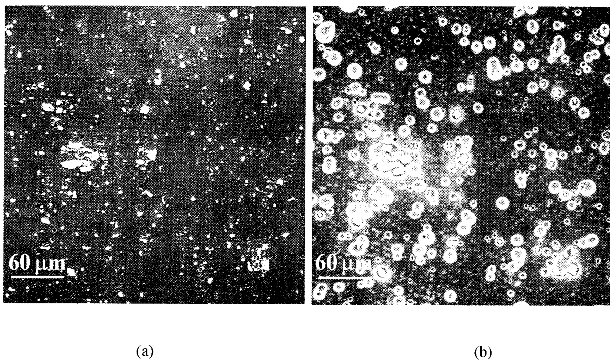
FIGURE 8. SEM MICROGRAPHS SHOWING PARTICLES AND CORROSION PITS FOR THE SAME AREA OF (a) AS-POLISHED SURFACE (BACKSCATTERED ELECTRON IMAGES) BEFORE 3-DAY EXPOSURE, AND (b) CORRODED SURFACE (SECONDARY ELECTRON IMAGES) AFTER 3-DAY EXPOSURE TO 0.5M NaCl SOLUTION AT 65°C
