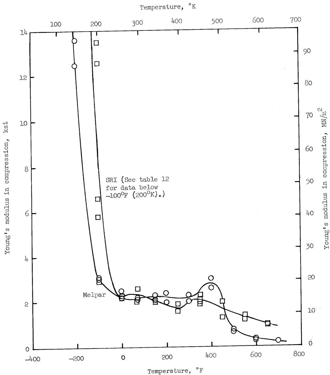
Figure 67.- Young's modulus of filled silicone resin in compression.
