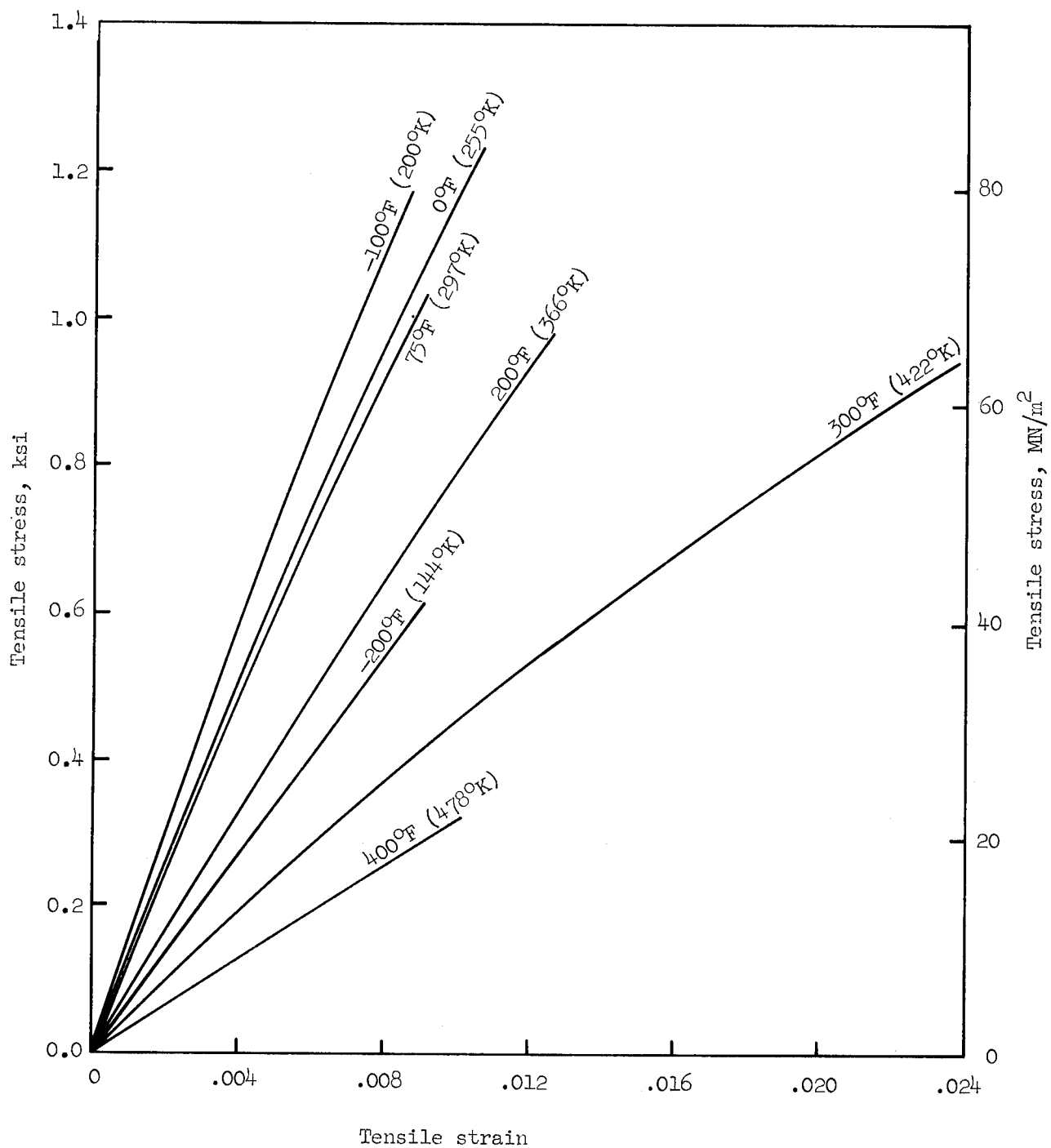
Figure 42.- Tensile stress-strain curves for low-density phenolic-nylon (Melpar).
