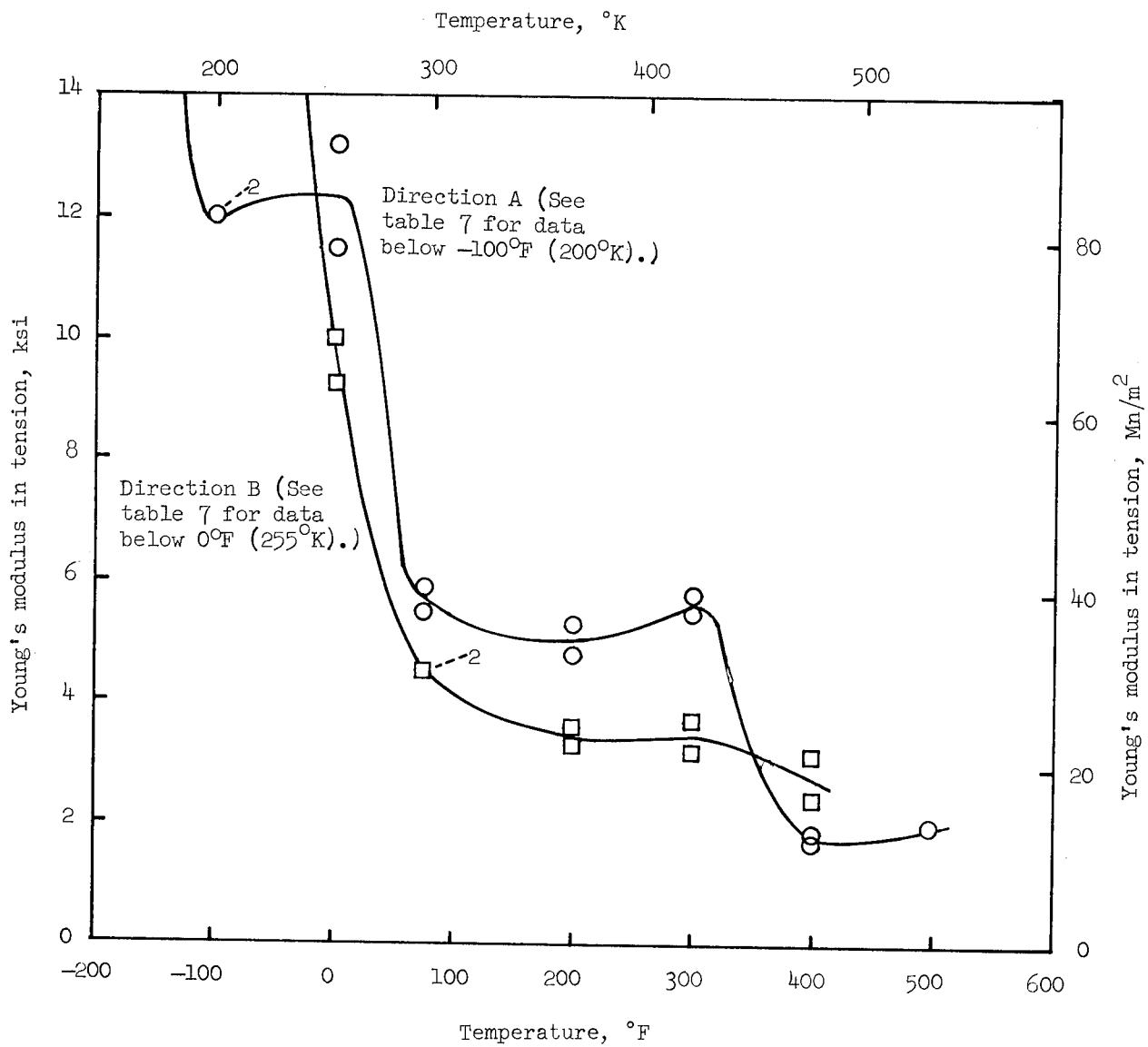
Figure 68.- Young's modulus in tension for filled silicone resin in honeycomb (Melpar).
