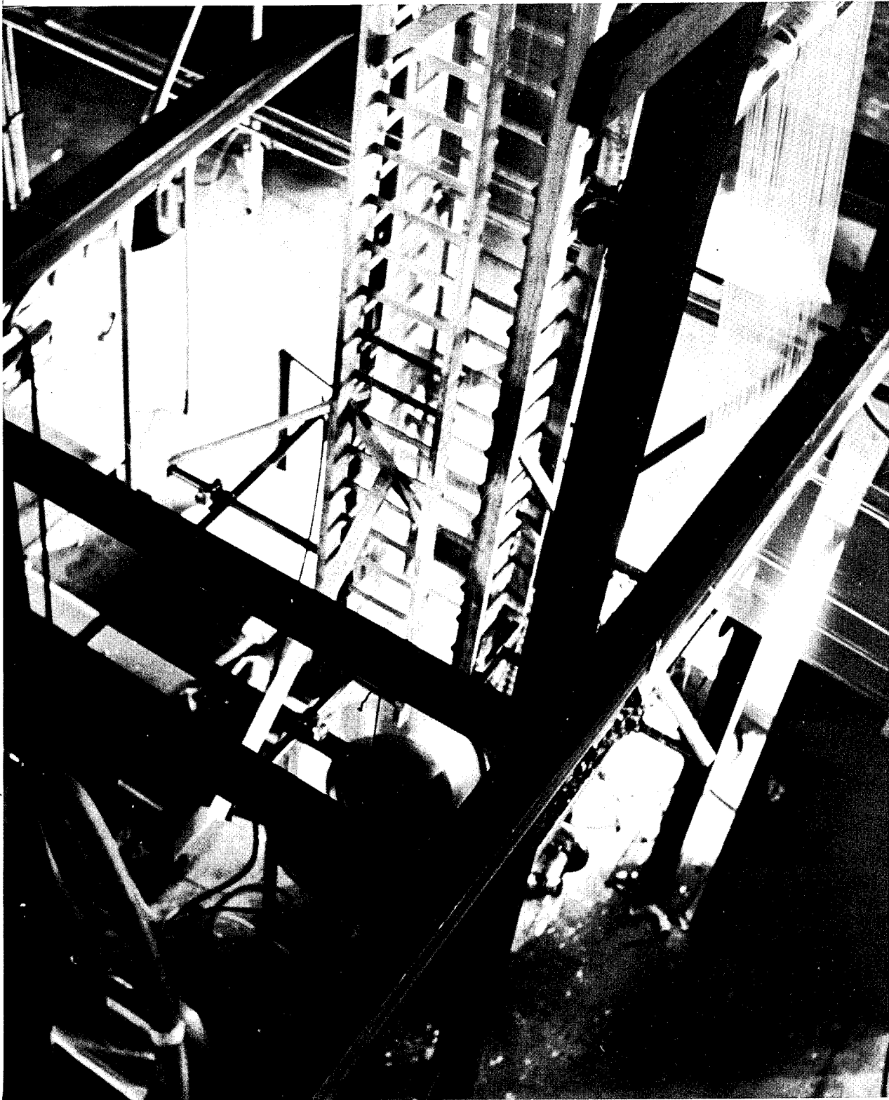
High Tower Take Up System Used for UTG Film Extrusion
