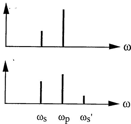
Figure 1(a). FWM-1
