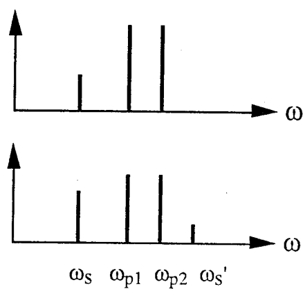
Figure 1(b). FWM-2
