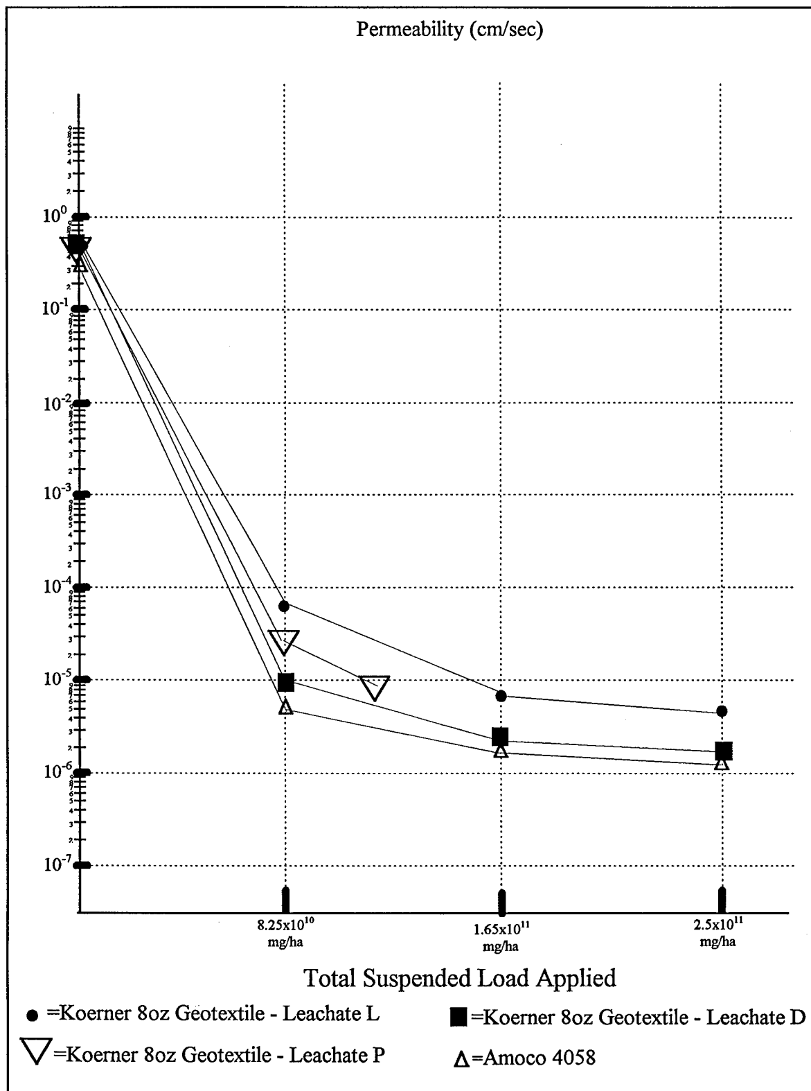
Figure 7.3: Permeability versus. TSS Load
