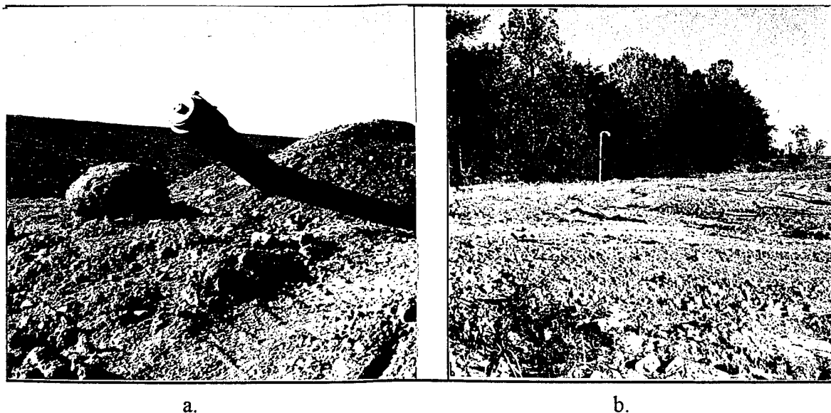
Figure 2.3: a. Leachate Collection Pipe Installed. b. Offgas Vent
