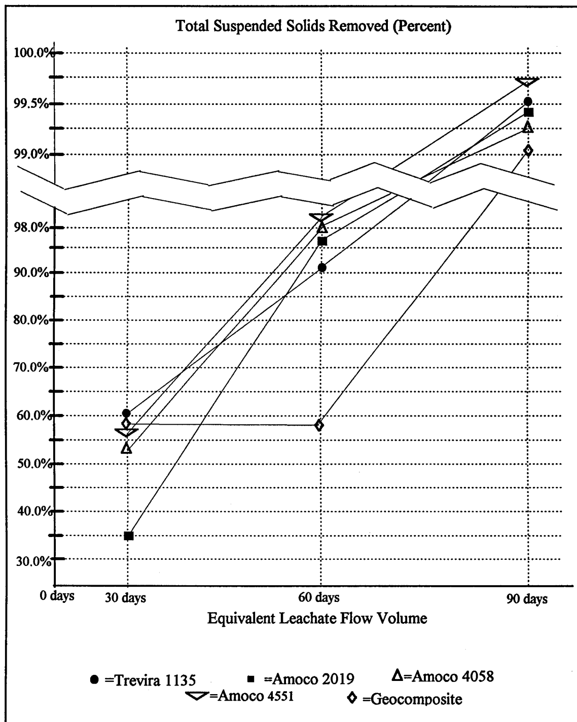
Figure 7.9: Total Suspended Solids Removal Percentages for All Geotextiles High Concentration Leachate Flow
