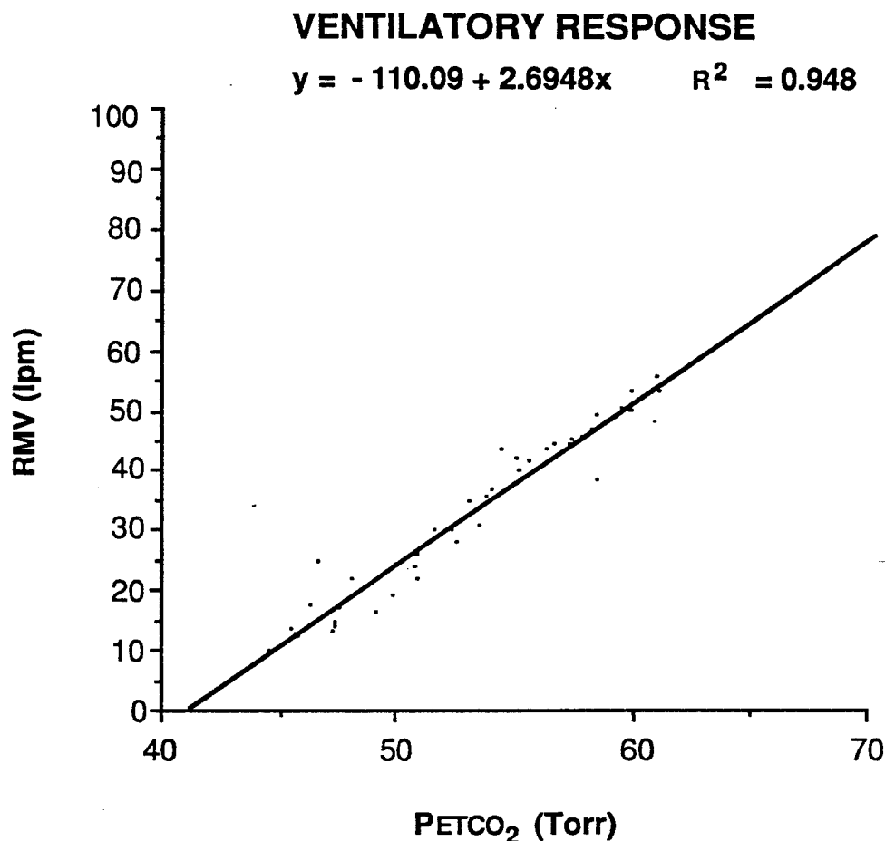
Figure 3: Ventilatory response to CO 2 determination from data recorded during a hypercapnic exposure at 0.21 ATA P I O 2 .
