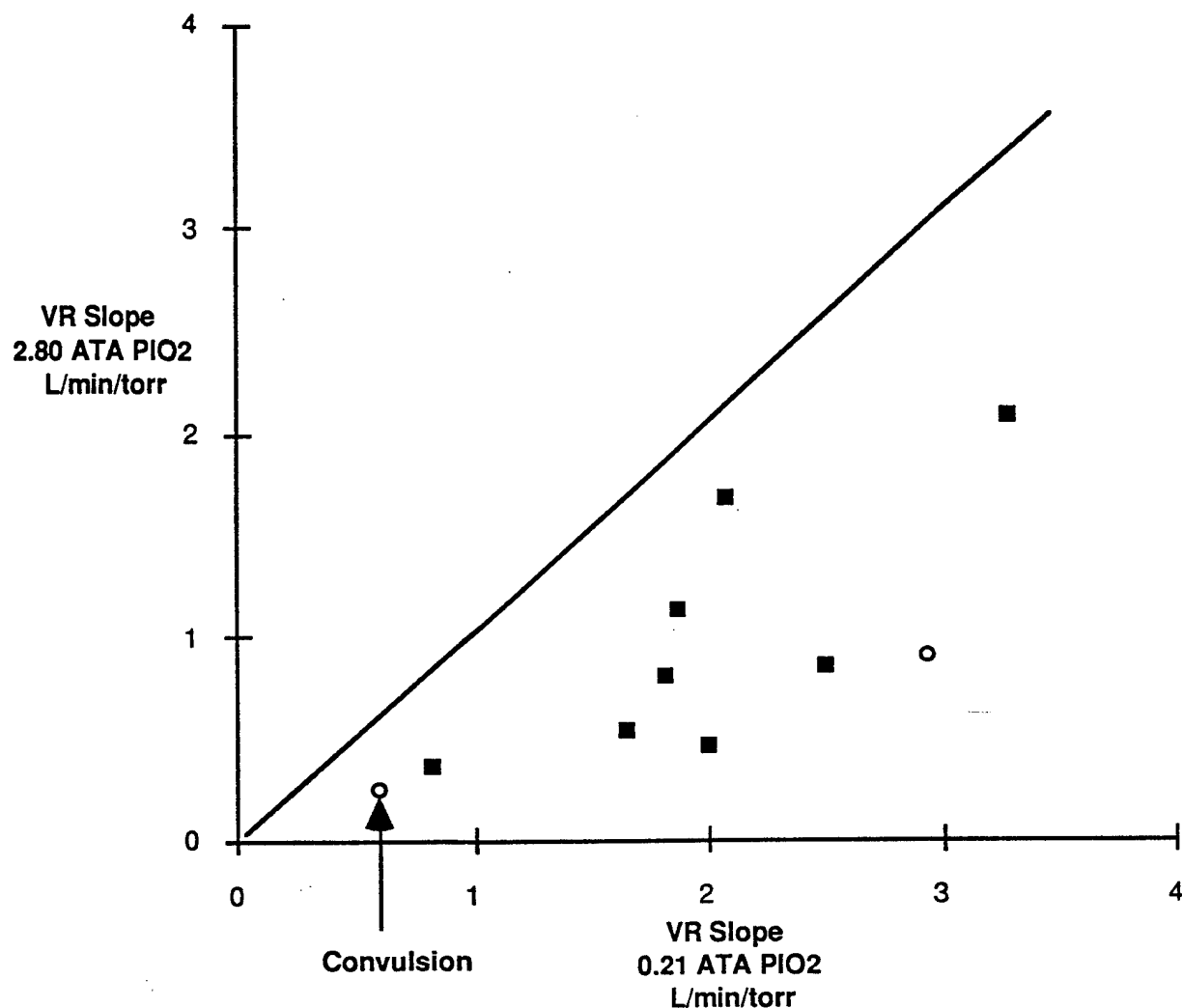
Figure 13 : Ventilatory response slopes from 0.21 ATA and 2.80 ATA P_{IO_2} experiments . The subjects with symptoms are designated by circles and the subject with the convulsion is indicated by the arrow.
