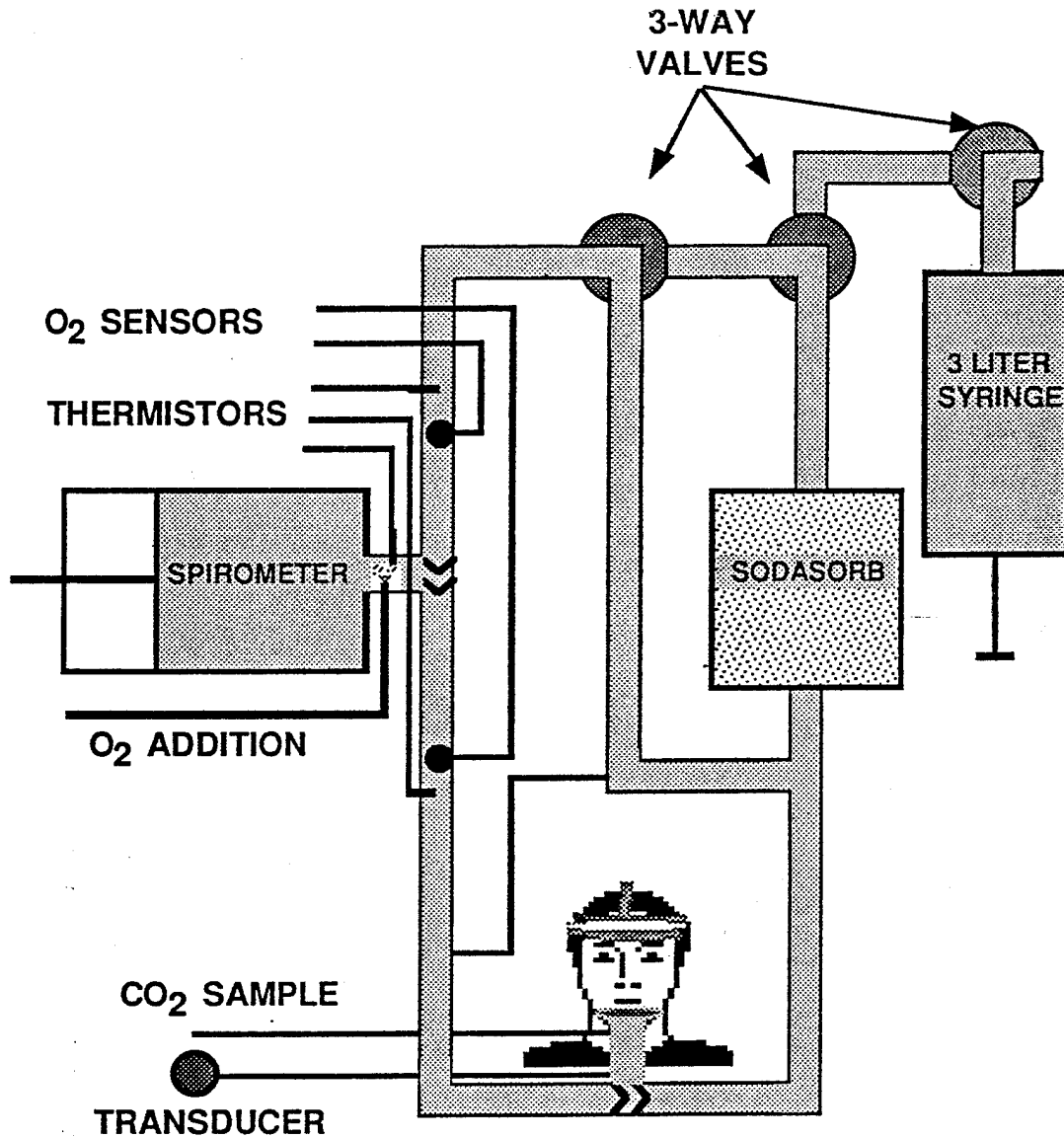
Figure 3: Closed-circuit breathing apparatus used to achieve oxygen and carbon dioxide pressures required for experimental conditions.
