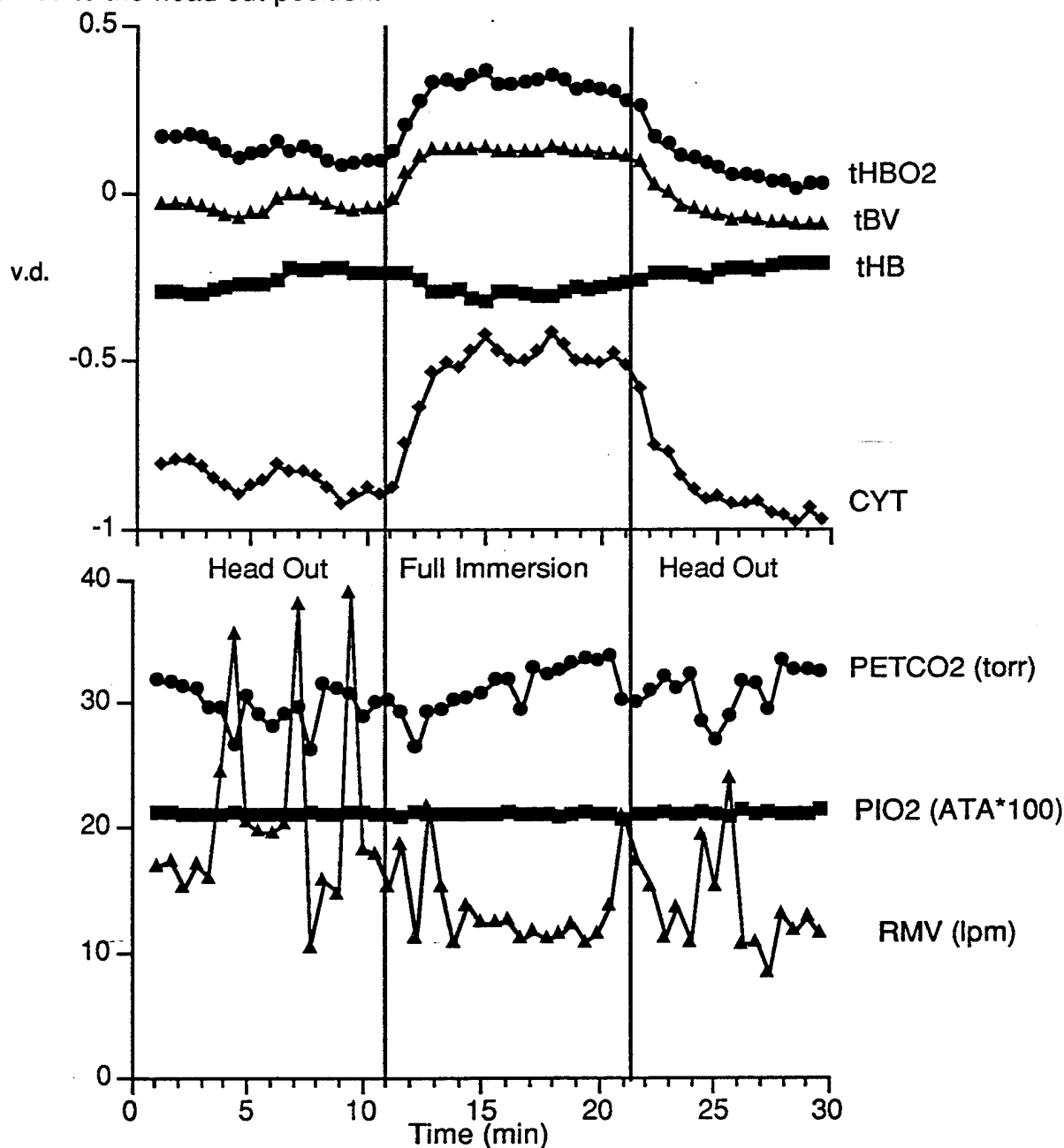
Figure 26: Typical head out / total immersion with negative static lung load experiment. Cerebral oxygenation measurements - brain tHb , tHbO_2 , tBV , and oxidized Cyt a,a_3 and ventilation, PIO_2 , and PETCO_2 are shown for an experiment at the surface on air at rest.
