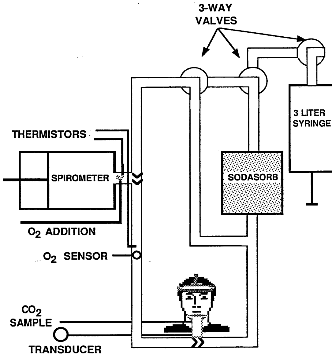
Figure 1: Closed-circuit breathing apparatus used to achieve oxygen and carbon dioxide pressures required for experimental conditions.
