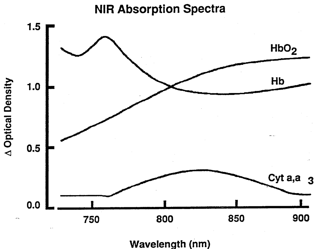
Figure 2: NIR absorption spectra of Hb, HbO 2 , and oxidized cytochrome a,a 3 (Piantadosi 1989 p. 311).
