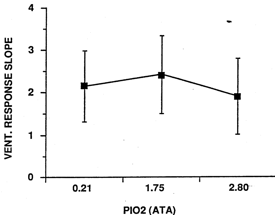
Figure 12: Mean ventilatory response slopes, \pm SD, (lpm·torr -1 ) at 0.21, 1.75, and 2.80 ATA PI_{O_2} for 30 experiments.
