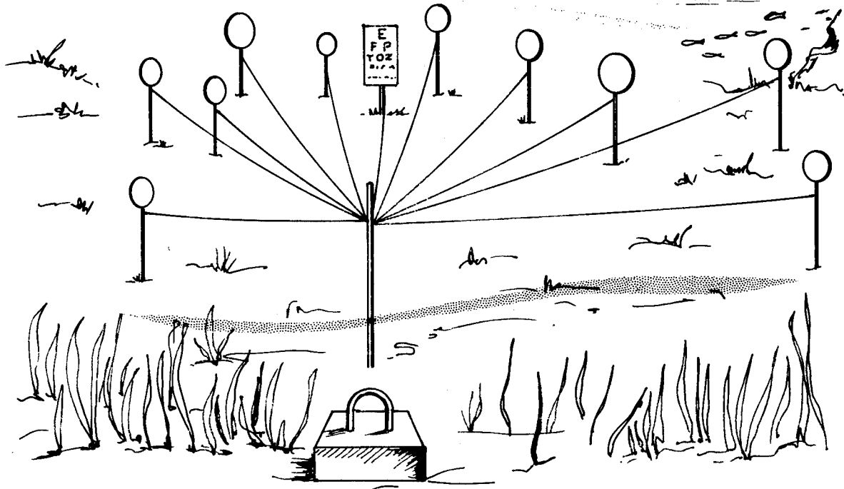
Figure 2. Visibility array.
