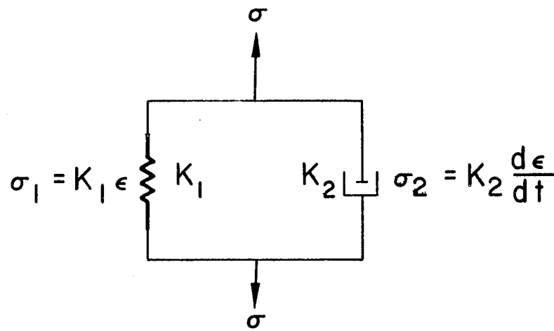
Fig. 4. Kelvin model.
