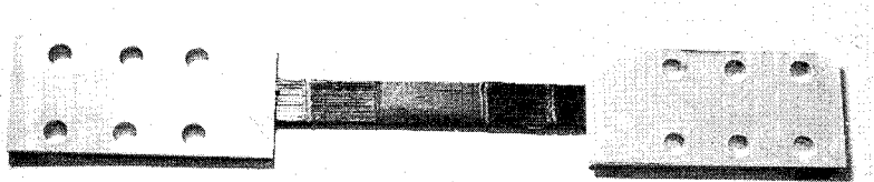
(c) Aluminum-tabbed tensile specimen showing test section and extensometer mounting pads.
