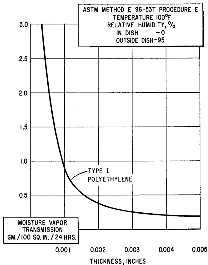
Figure III MOISTURE VAPOR TRANSMISSION VERSUS THICKNESS
