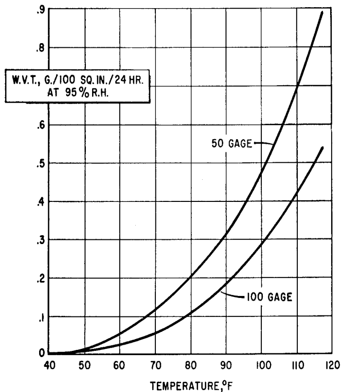
Figure I WATER VAPOR TRANSMISSION VS TEMPERATURE OF SARAN WRAP No's. 20 THRU 39
