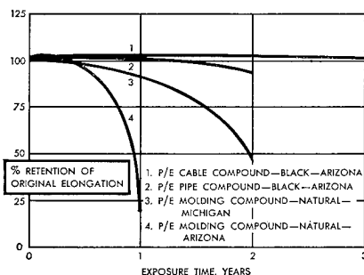
FIG. 1 RELATIVE EFFECT OF OUTDOOR EXPOSURE ON POLYETHYLENE FORMULATIONS
