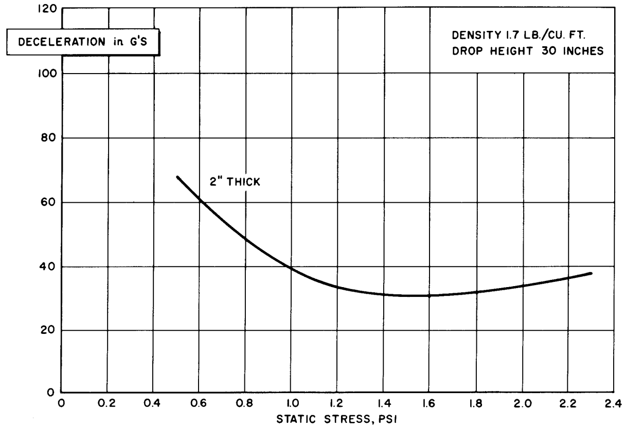
FIGURE 5 DYNAMIC CUSHIONING PROPERTIES OF STYROFOAM
