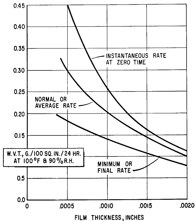
Figure II WATER VAPOR TRANSMISSION VS THICKNESS OF SARAN WRAP No's. 1 THRU 19
