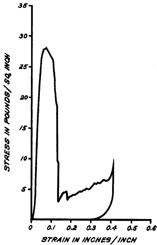
FIG. 22A BALSAM WOOD BLOCK TEST SPEED 2 INCHES/MINUTE SIZE 4"x 4"x 2"
