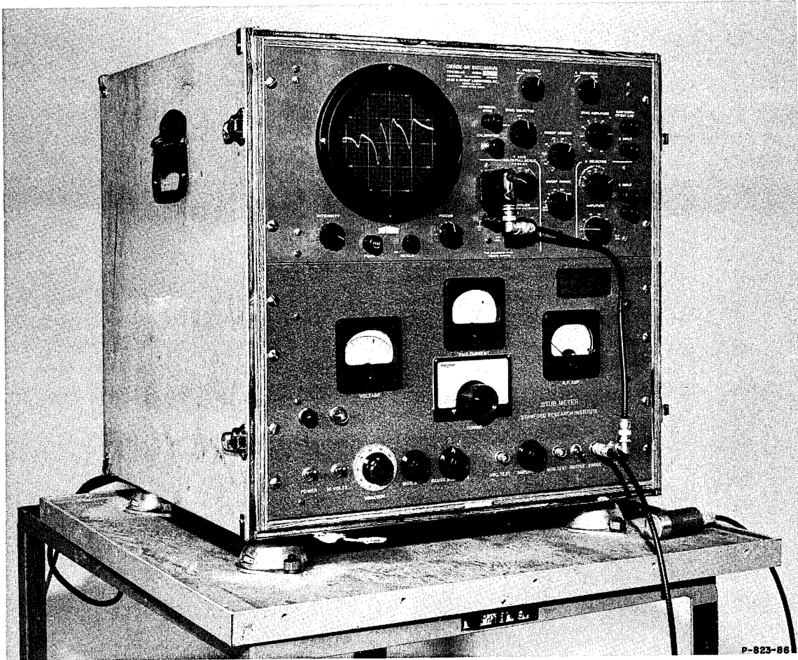
FIG. 9 MODEL 3 STUB-METER
