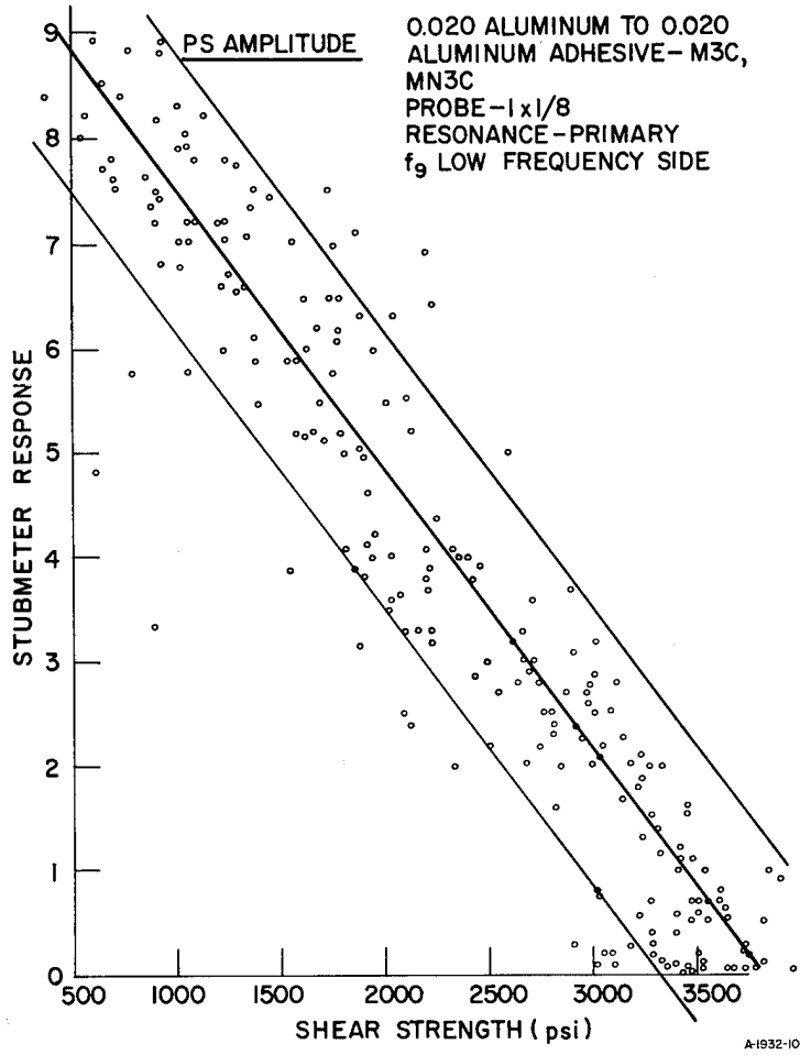
FIG. 10 CORRELATION PLOT Shear Strength vs STUB Meter Response
