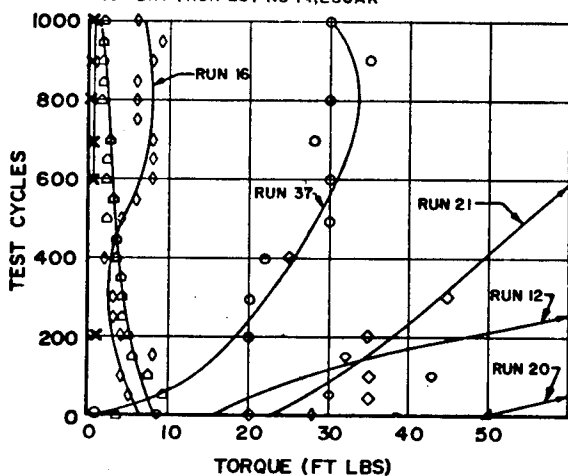
Figure 5. Cycling Tests: Materials and Conditions
